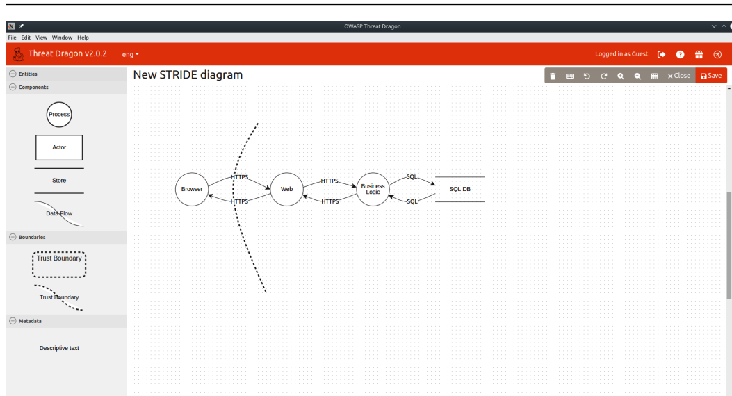
Figure 4.7 – Threat Dragon
