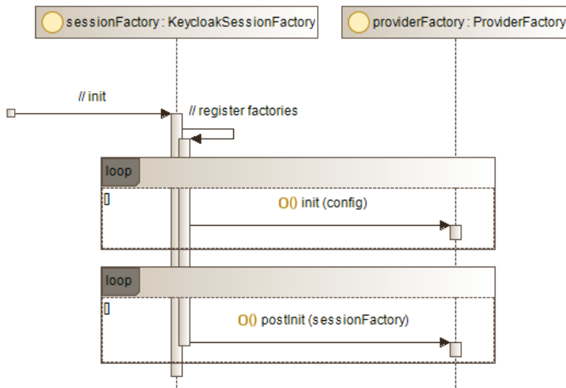
Figure 13.5 – Initialization of factories during server startup
