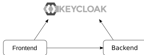
Figure 2.1 – Application overview
