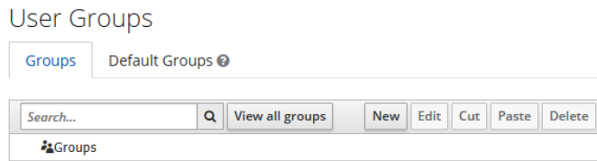
Figure 8.3 – Listing groups
