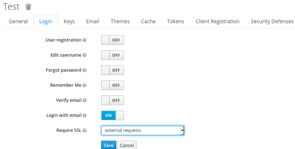
Figure 9.1 – Enforcing HTTPS on a per-realm basis
