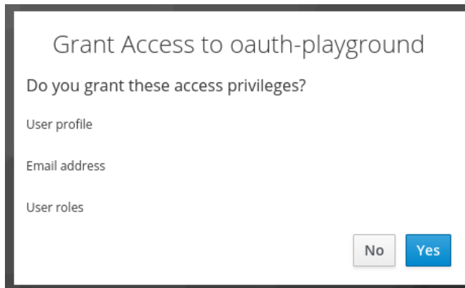
Figure 5.6 – Granting access
