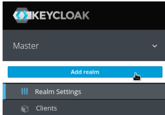
Figure 1.4 – Realm selector
