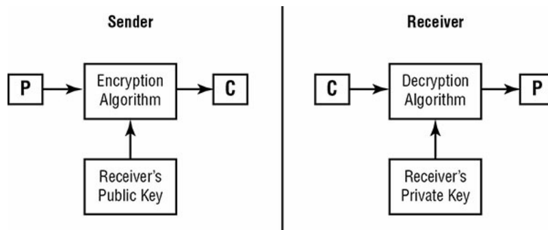
FIGURE 6.4 Asymmetric key cryptography
