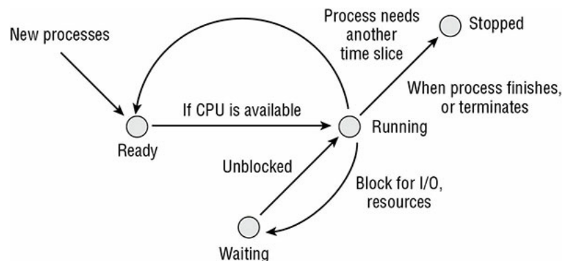
FIGURE 9.2 The process scheduler
