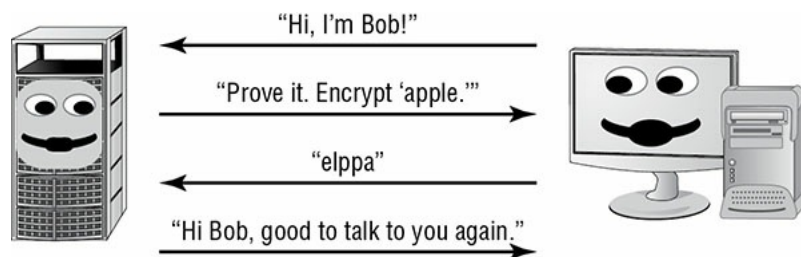
FIGURE 6.1 Challenge-response authentication protocol
