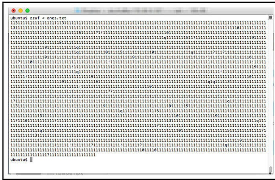
FIGURE 15.11 The input file from Figure 15.10 after being run through the zzuf mutation fuzzing tool
