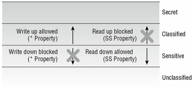
FIGURE 8.3 The Bell-LaPadula model
