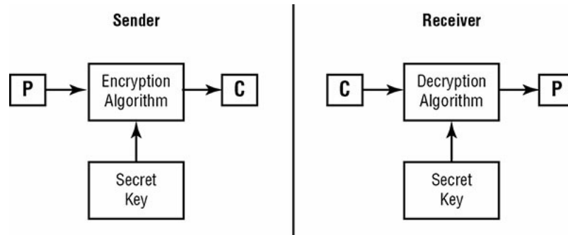
FIGURE 6.3 Symmetric key cryptography
