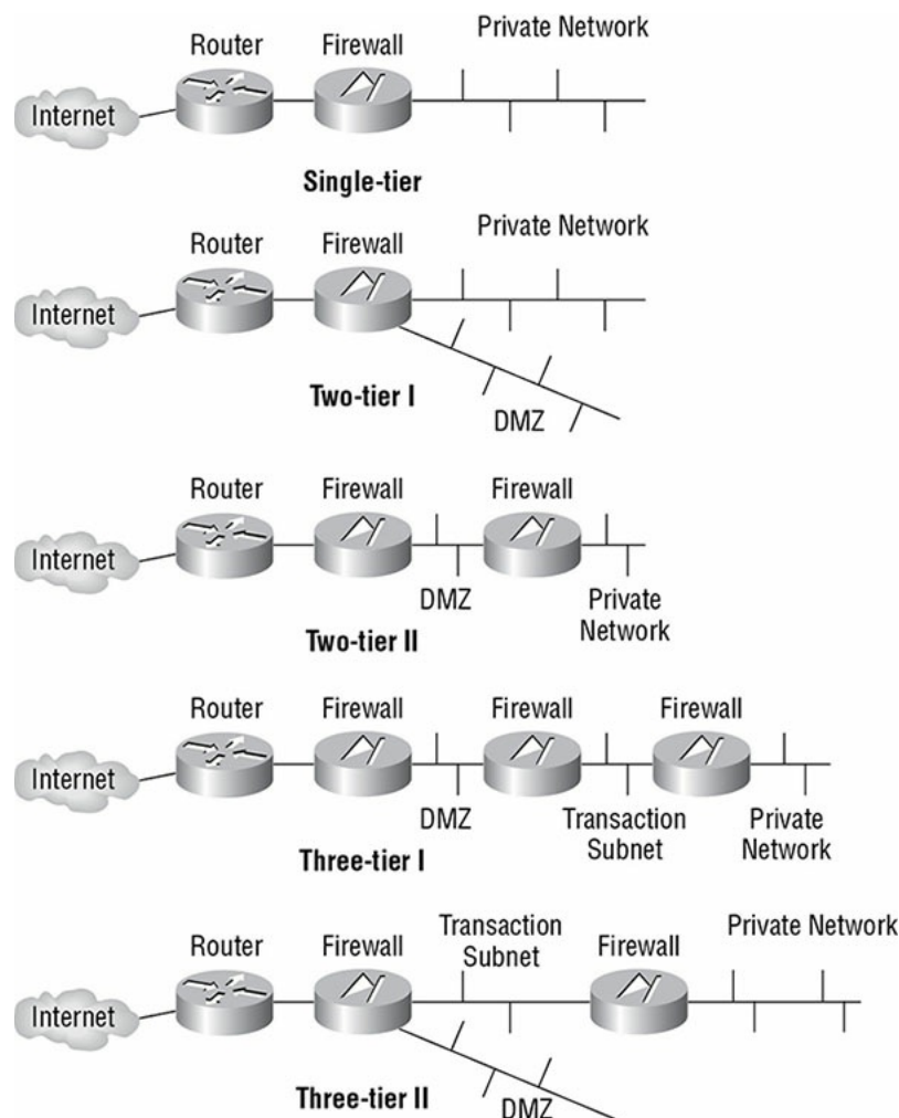
FIGURE 11.8 Single-, two-, and three-tier firewall deployment architectures
