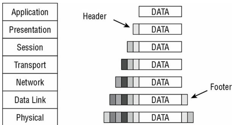
FIGURE 11.2 Representation of OSI model encapsulation
