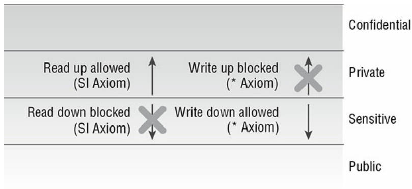
FIGURE 8.4 The Biba model
