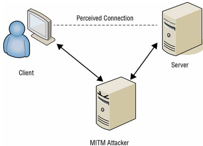
FIGURE 17.3 A man-in-the-middle attack
