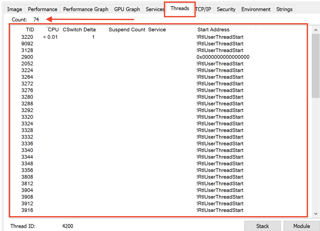
Figure 2.2 – Running threads under a process in Windows 10
