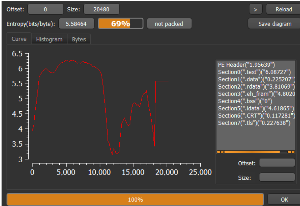
Figure 5.15 – DiE entropy value
