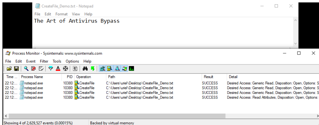
Figure 4.10 – ProcMon CreateFile example
