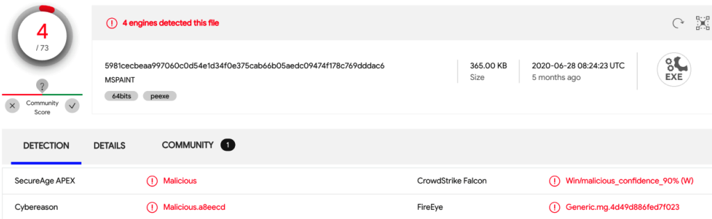
Figure 5.44 – VirusTotal's results of the original mspaint.exe file after packing with UPX
