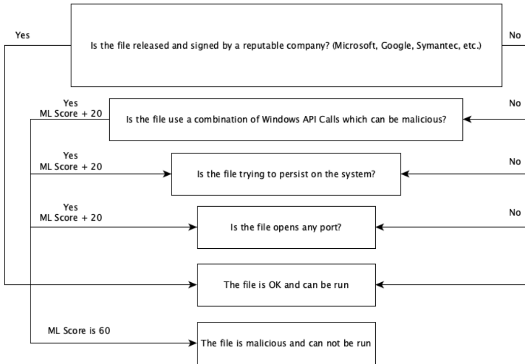
Figure 6.17 – "ML" diagram
