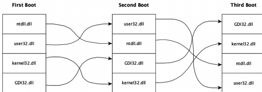
Figure 3.2 – ASLR illustration
