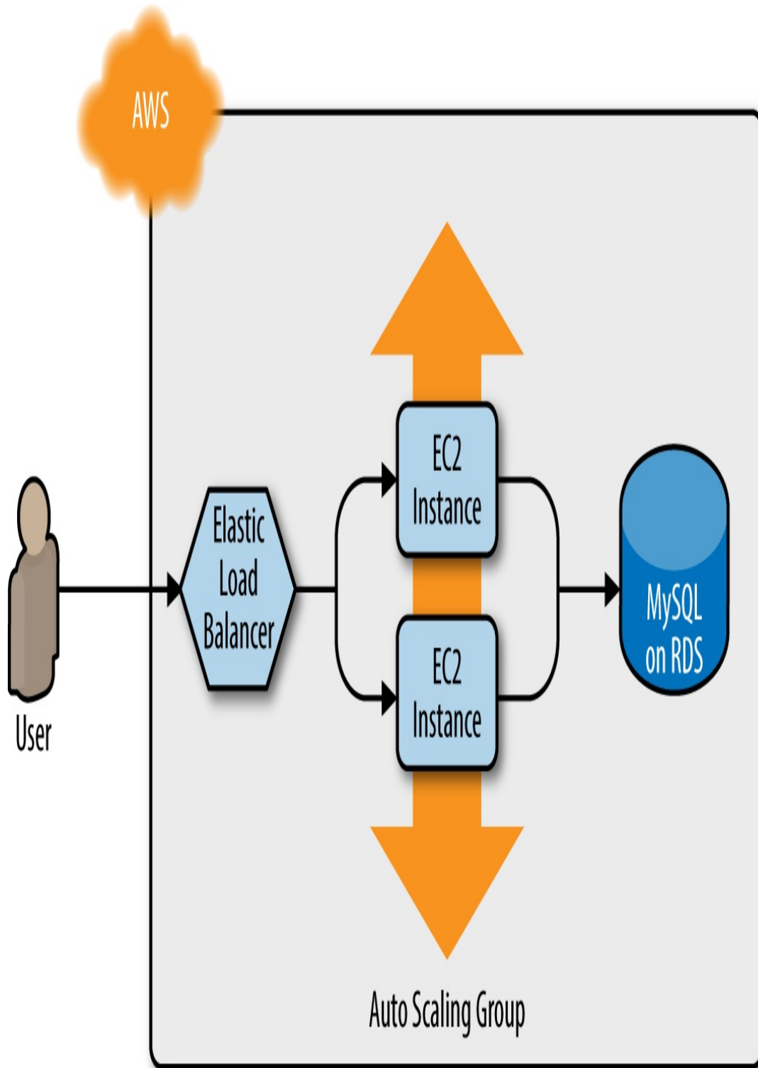
Figure 3-9. The web server cluster communicates with MySQL, which is deployed on top of Amazon RDS
