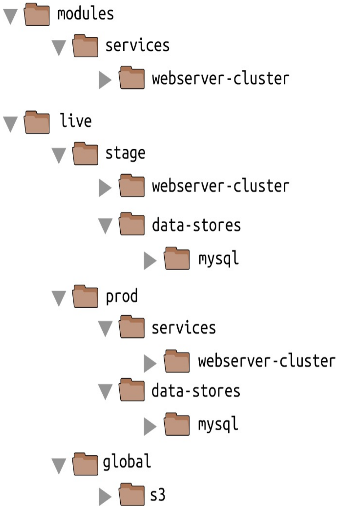
Figure 4-6. File layout with multiple repositories
