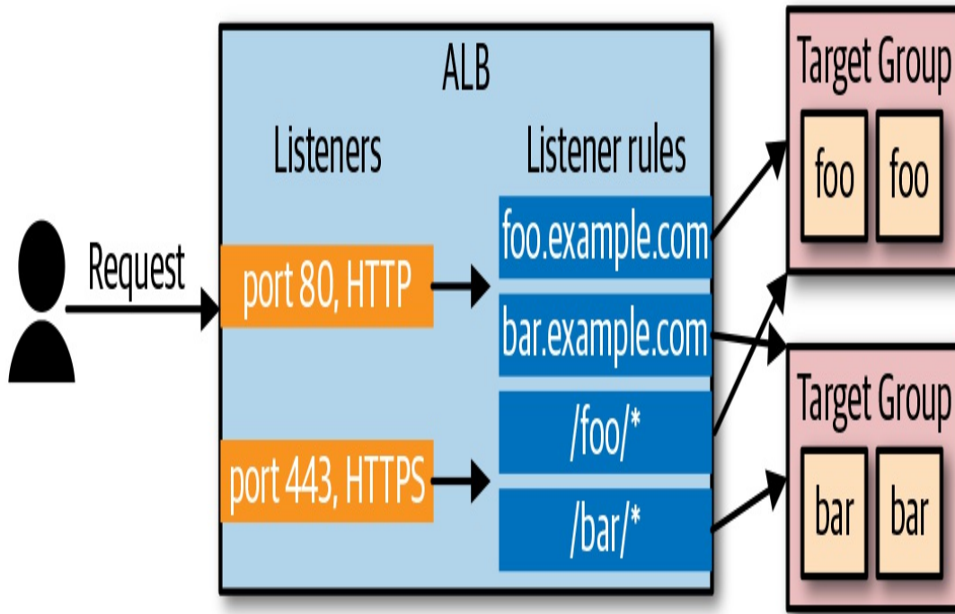
Figure 2-11. Application Load Balancer (ALB) overview
