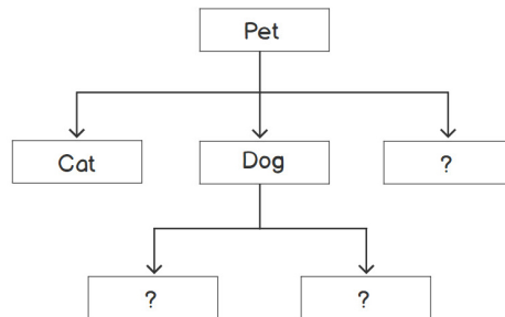
Figure 5.12 – Class inheritance
