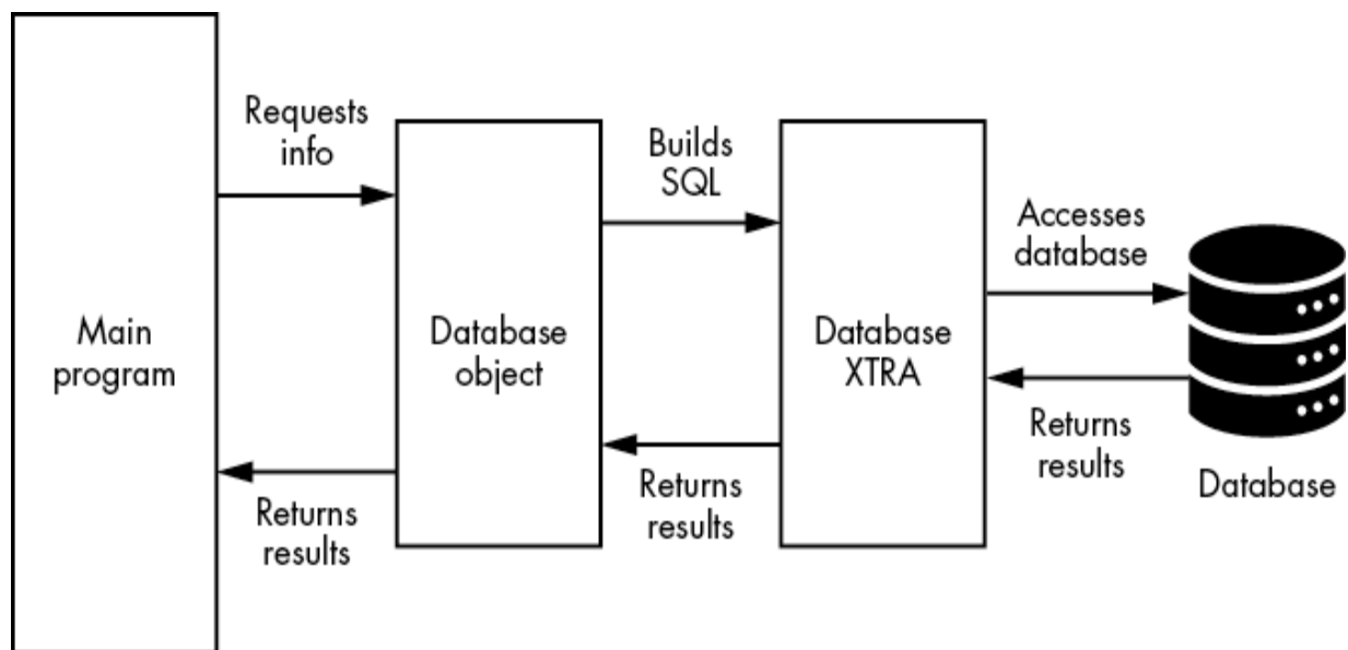
Figure 8-1 : The architecture of accessing a database using an object and an XTRA
