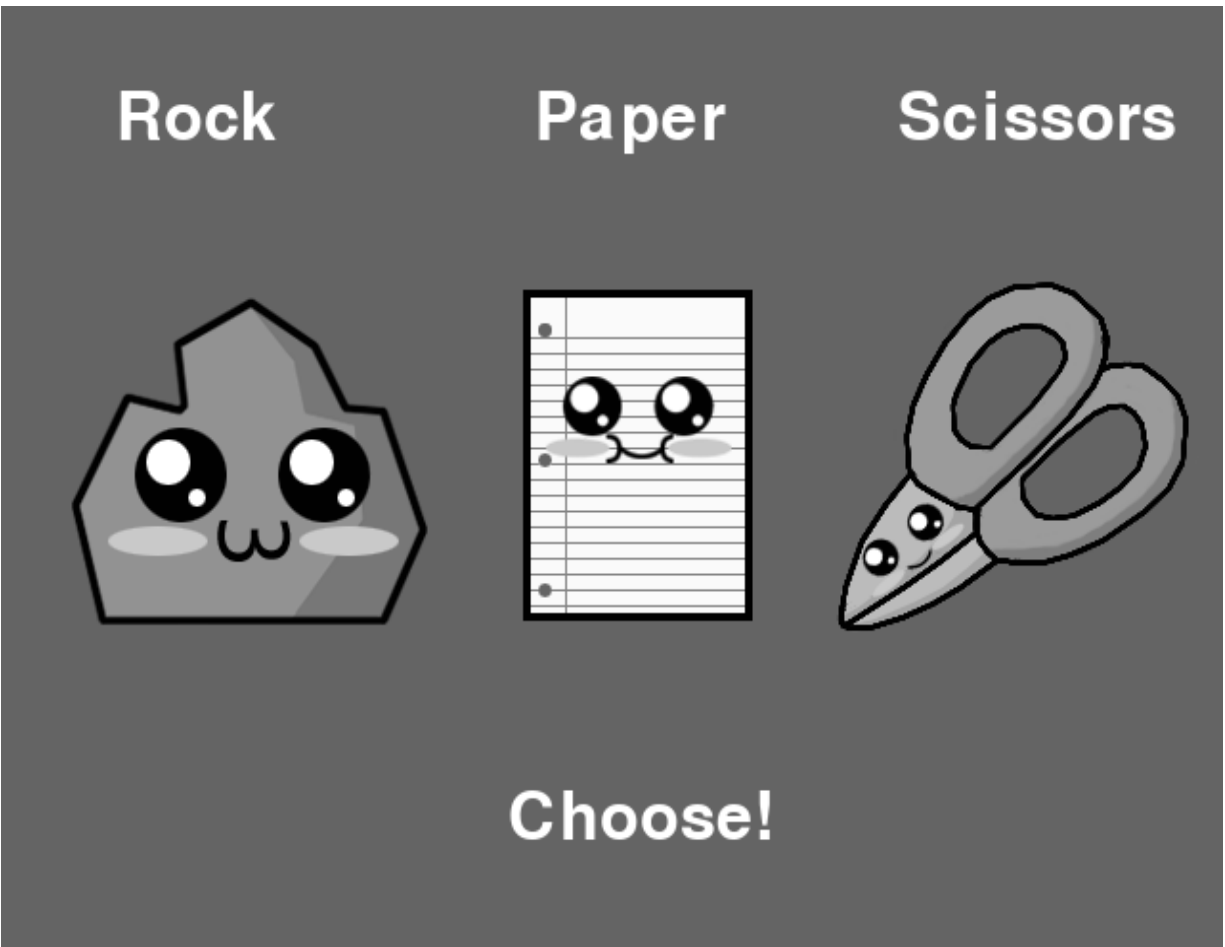
Figure 15-2: The Rock, Paper, Scissors Play scene
