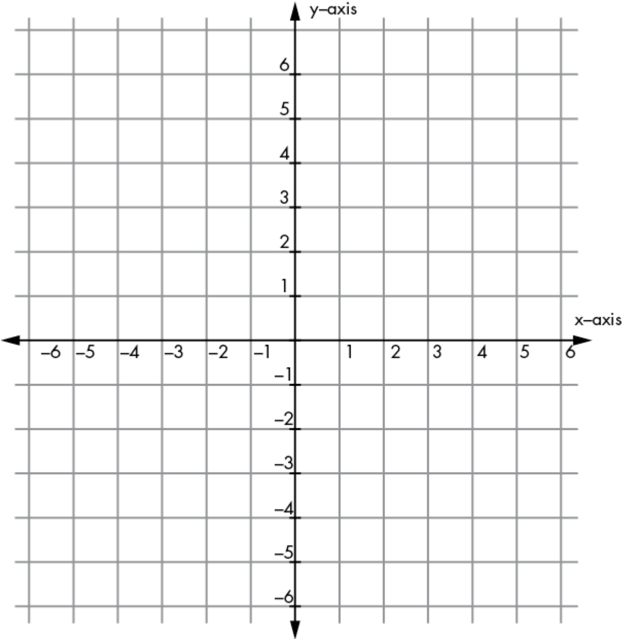
Figure 5-1: The standard Cartesian coordinate system
