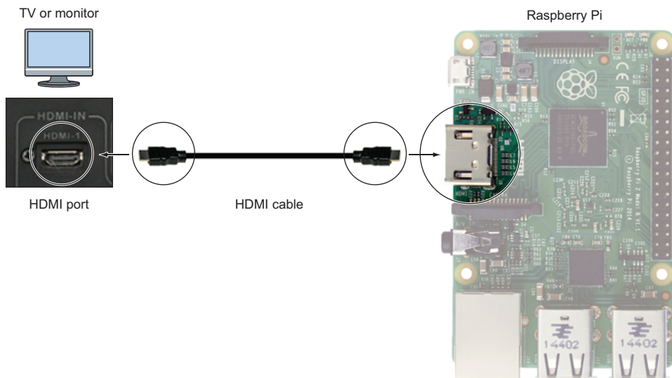
Figure 1.9 A Raspberry Pi can be connected to a TV or monitor using an HDMI cable. Connect the cable from the Pi's HDMI port to the TV's or monitor's HDMI input. In addition to video, the HDMI cable also contains the Pi's audio output, which can be played through the TV's or monitor's speakers.
