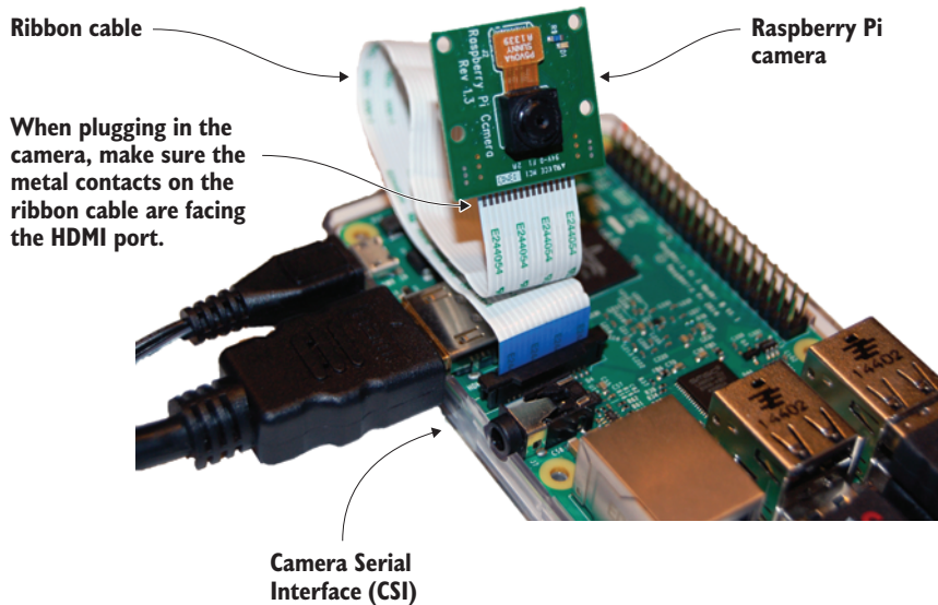
Figure B.6 The Raspberry Pi camera can connect to the CSI port, which is located between the HDMI port and the 3.5 mm audio/video port. To connect a camera, you need to lift up the black connector, insert the ribbon cable (metal contact toward the HDMI port), and push down on the black connector again.
