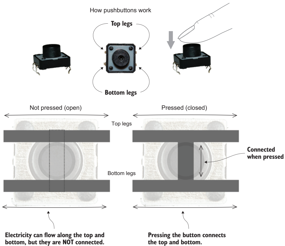
Figure 8.6 In a button, the legs are connected along the top and are separately connected along the bottom. When the button is pressed, the top and bottom are connected by a small metal bar.
