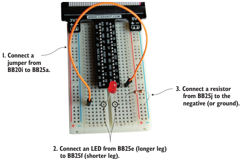
Figure 6.10 LED circuit built on the breadboard. You're using GPIO pin 21 as the power source. The light won't turn on until you program the voltage to come out of the pin.
