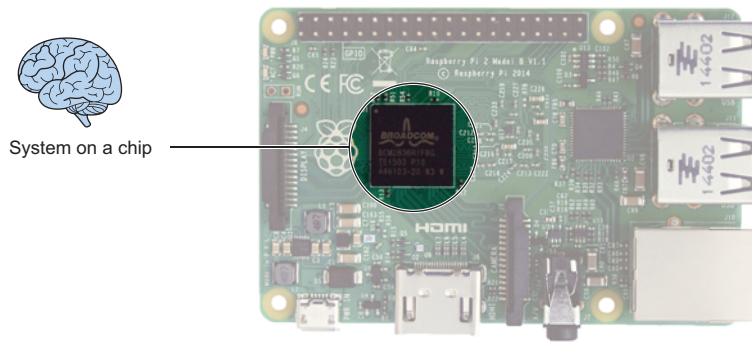
Figure 1.3 The Raspberry Pi's system on a chip (SoC) contains its computing and graphics processing power and working memory. The Pi uses the ARM11 microprocessor as its CPU and the VideoCore IV for its GPU. The ARM11 microprocessor is found in handheld electronics such as smart phones and gaming systems. The SoC in the Raspberry Pi 2 Model B comes with 1 GB of RAM.
