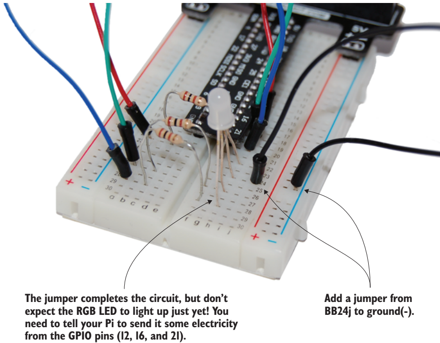
Figure 7.11 The jumper is added to connect the ground of the RGB LED to the ground of the Raspberry Pi. The jumper can connect anywhere along the ground rail (it usually has a blue stripe running next to it).
