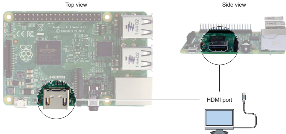
Figure 1.7 The HDMI port on the Raspberry Pi provides a high-definition audio and video signal that can be connected to a TV or monitor. Use an HDMI cable to connect your Pi to your TV or monitor. Depending on the connectors available on the TV or monitor, you may need an adapter.
