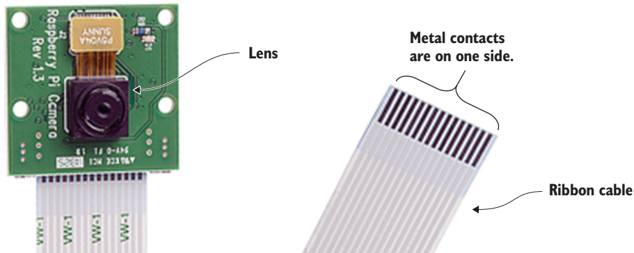
Figure B.5 The Raspberry Pi camera module was created by the Raspberry Pi Foundation to take high-def digital photographs and video. The camera attaches to the Pi using a ribbon cable that connects to the Camera Serial Interface port. The camera module can be programmed using Python and used for nature photography or creating your own home-surveillance system.
