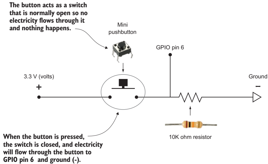
Figure 8.4 The circuit diagram for the first button in the DJ Raspi project shows how electricity will flow through the circuit. The button is a switch that allows electricity to flow to GP06 and ground (-) when it's pressed or closed.
