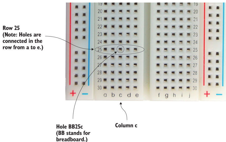
Figure 6.8 To find a specific hole on a breadboard, use the row and column labels. This is a close-up of a breadboard, showing how you can find the location of hole 25c (we’ll refer to the hole as BB25c, where BB stands for breadboard ).
