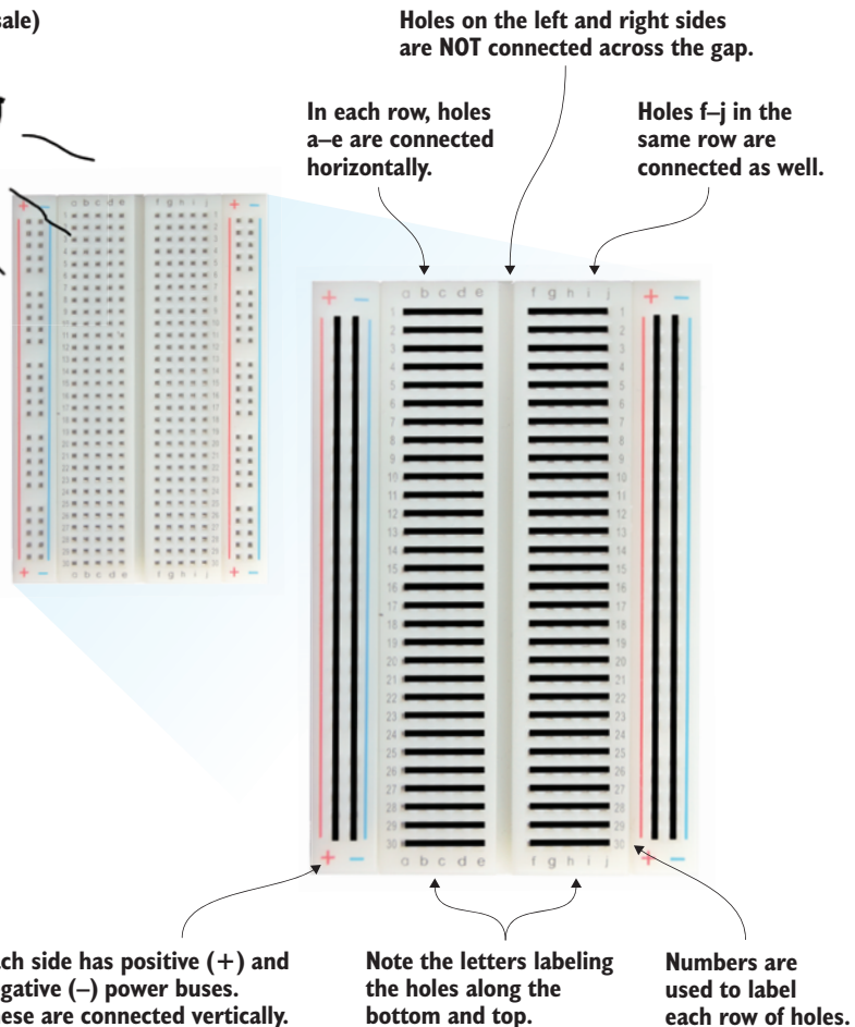
Figure 6.7 Breadboards have internal connections. You need to know about them in order to build circuits. Rows of pins are connected horizontally, but not across the gap in the middle. Long rails called power buses run vertically along the sides of the board.
