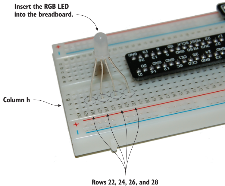
Figure 7.7 Bend the legs of the RGB LED, and insert it into the breadboard at BB22h, BB24h, BB26h, and BB28h. The longest leg goes into hole BB24h.
