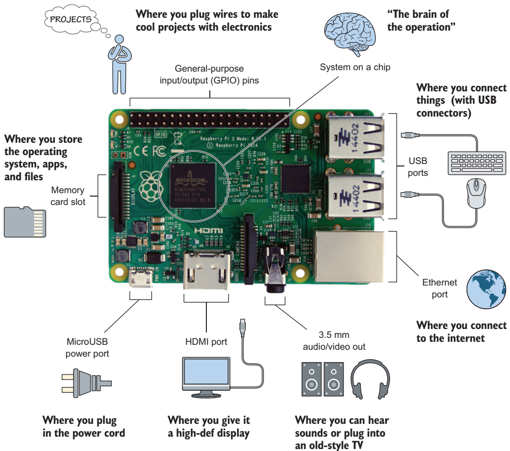
Figure 1.1 The Raspberry Pi provides an excellent platform for learning to program in Python. It includes many input and output ports to give you flexibility in how you connect it. As you would with a desktop computer, you need to connect a keyboard, mouse, monitor, and power cable before you can start using your Pi.
