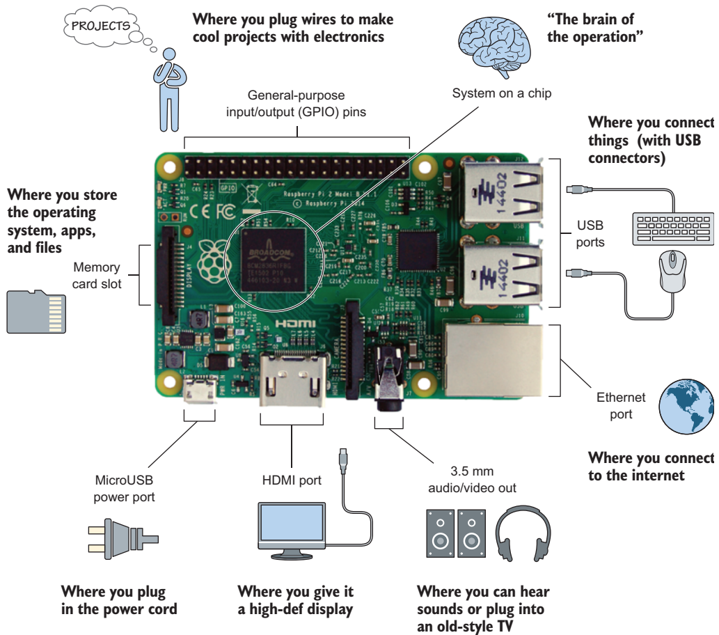
Figure B.1 The Raspberry Pi 2 Model B has many different input and output ports that allow you to connect a keyboard or mouse, monitor, and even high-definition cameras.
