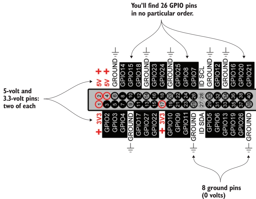
Figure 6.3 The Raspberry Pi B+ has 40 pins. They do different things: some provide 5 volts or 3.3 volts, some are ground pins (0 volts), and many of them are input and output pins that you can program.
