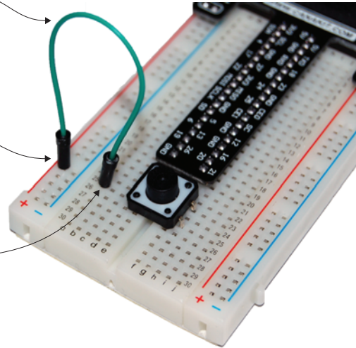
Figure 8.8 The jumper connects power (3.3 volts) to the bottom of the button.
