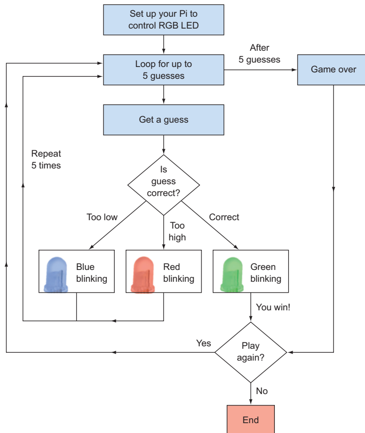
Figure 7.12 Flow diagram showing how the guessing game should work. Notice how you're blinking LEDs if the guess is too low, too high, or correct. You also give the player the choice of whether they'd like to play again.
