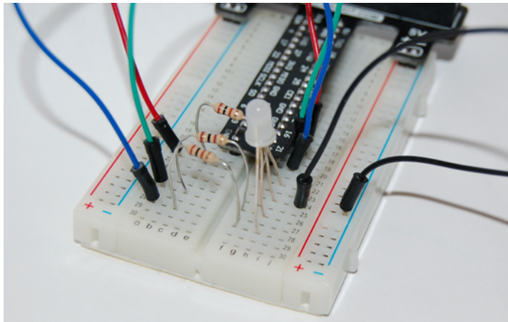
Figure 7.5 The RGB LED circuit you're building on the breadboard uses GPIO pins 12, 16, and 21 to power the LEDs. The light won't turn on until you program the voltage to come out of the pins.
