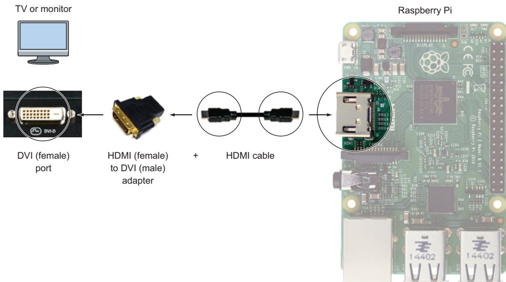
Figure 1.10 The Raspberry Pi can be connected to a TV or monitor with a DVI port using an HDMI-to-DVI adapter and an HDMI cable. One end of the HDMI cable plugs into the Pi's HDMI port. The other is connected to the adapter, and the adapter is connected to the TV or monitor. Adapters are available through online retailers or local computer stores.
