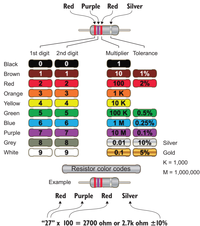
Figure 7.9 The colored bands on a resistor tell you how much resistance the resistor has. For this project, you want a brown (1), grey (8), brown ( \times 10 ) resistor, or 18 \times 10 = 180 ohm resistor. Don't have one? Any resistor between about 100 and 300 ohms should work well.
