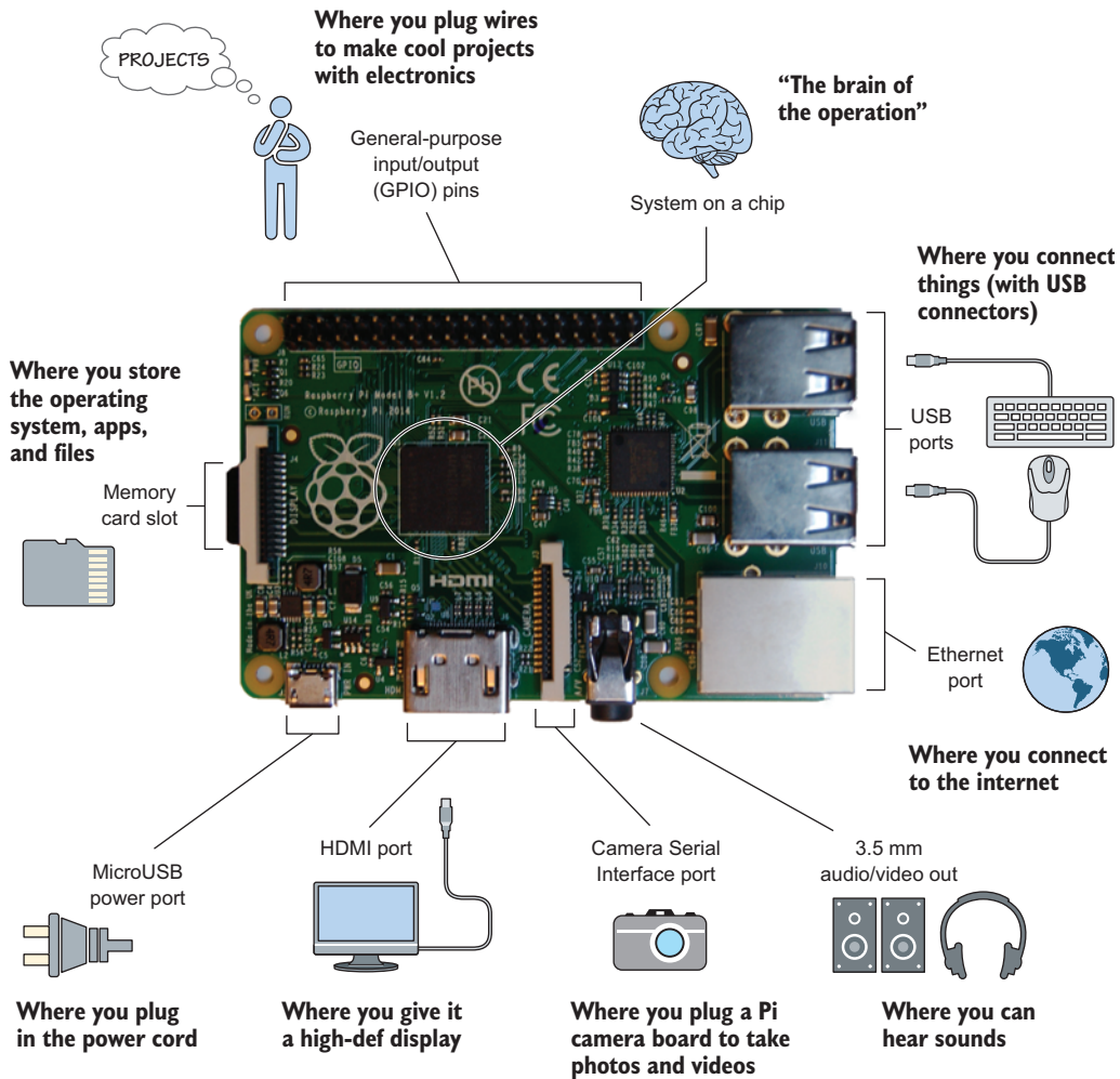
Figure B.11 The Raspberry Pi 1 Model B+ was a major revision of the Raspberry Pi 1 Model B. It increased the number of USB ports from two to four, added more pins for GPIO, and changed to a microSD memory card slot. The ports on the Raspberry Pi 1 Model B+ are the same as those on the Raspberry Pi 2 Model B.
