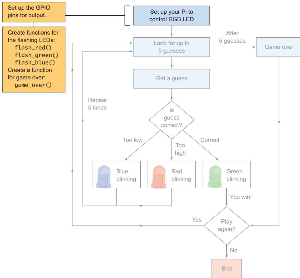
Figure 7.13 The program starts by importing the Python libraries you’ll need to use, setting up your Pi’s GPIO pins for lighting up the LEDs, and defining the functions you’ll need.
