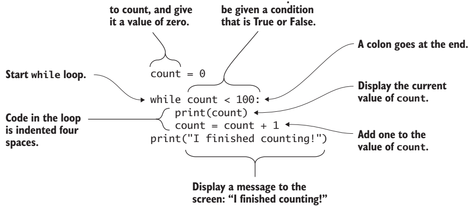
Figure 4.14 You can use a while loop to repeatedly perform a task. Code that is part of the loop is indented four spaces. In this case, this while loop displays the numbers from 0 to 99; when completed, it prints the message, "I finished counting!" Typically, the condition should be such that code in the loop can make it False and thus end the loop.
