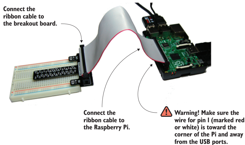
Figure 6.6 Connect one end of the ribbon cable to the breakout board. Connect the other end to your Raspberry Pi.
