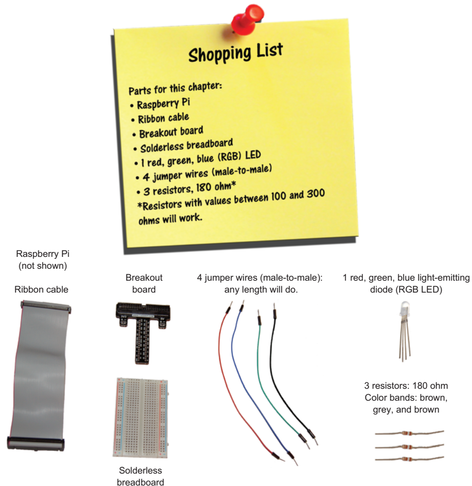
Figure 7.1 The Light Up Guessing Game uses a red, green, blue (RGB) LED. An RGB LED can produce many different colors because it has three LEDs (colored red, green, and blue) packed inside it.
