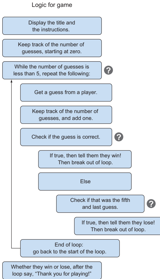
Figure 4.2 The game logic can be expressed in words. The question marks symbolize when the game needs logic to make a decision. This diagram also shows what code needs to be repeated because the player gets five guesses. Each decision has a simple True/False or Yes/No answer.
