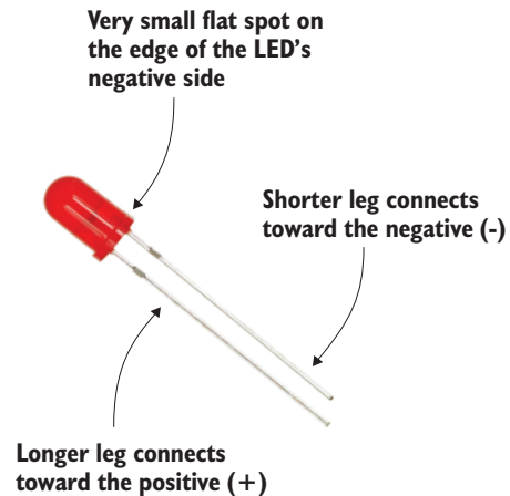
Figure 6.12 LEDs have two legs (wires) coming out of them. The longer leg is called the anode and connects to the positive side of the circuit. The shorter one is called the cathode and connects to the negative side of a circuit.
