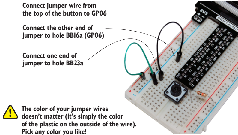
Figure 8.10 The jumper connects the top of the button to GP06. Later, you'll set your Pi to listen for electrical input on this GPIO pin.
