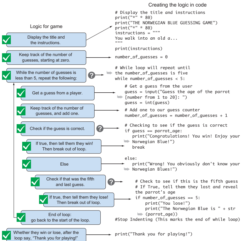
Figure 4.13 Think of the logic you're trying to create, and then translate it into your code. When you need to repeat something, you can use a while loop. When you need to check whether something is True or False, you can use an if statement.
