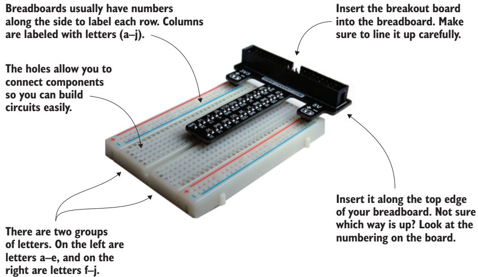
Figure 6.5 Carefully line up the breakout board, and then press it firmly into the breadboard. The two rows of pins on the breakout board should straddle the center gap.
