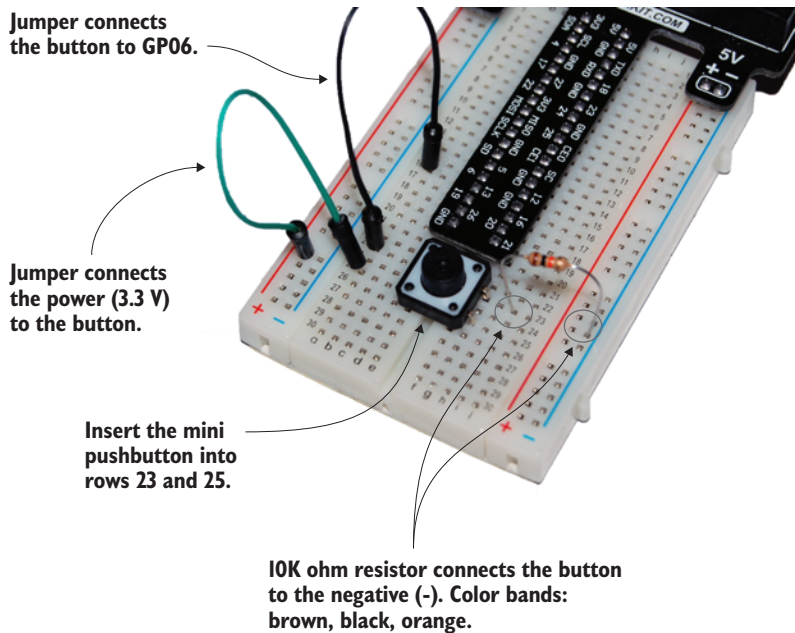
Figure 8.5 The mini pushbutton will have 3.3 volts connected to it from the positive power rail. When the button is pressed, power flows through the button and splits. Some electrical current goes to GP06 (GPIO pin 6), and the rest goes through the resistor and then to the negative power bus (-).
