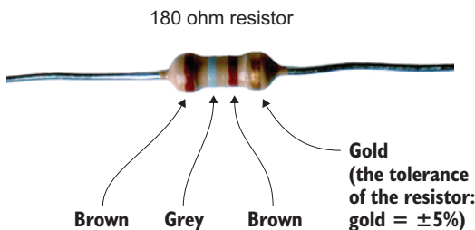
Figure 6.13 The value of a resistor is determined by its colored bands. See the sidebar "Resistor color codes" for a chart; there are also many online color-code charts.
