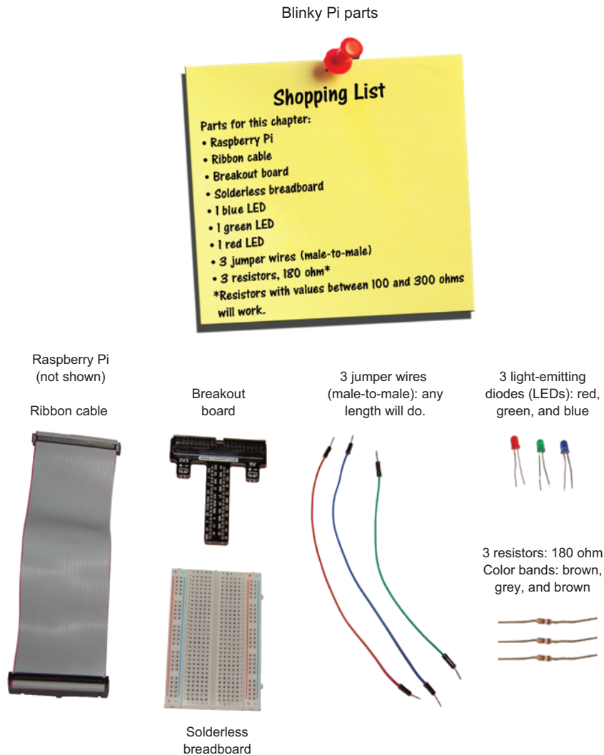
Figure 6.1 The Blinky Pi project requires parts that are commonly found in Raspberry Pi starter kits or that can be purchased online.
