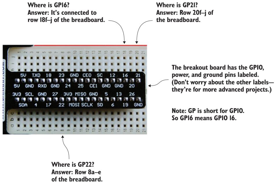
Figure 6.11 The breakout board has labels that correspond to the pins on your Pi. To connect a wire to GP16, you plug it into the breadboard in the hole labelled BB18f or BB18j.
