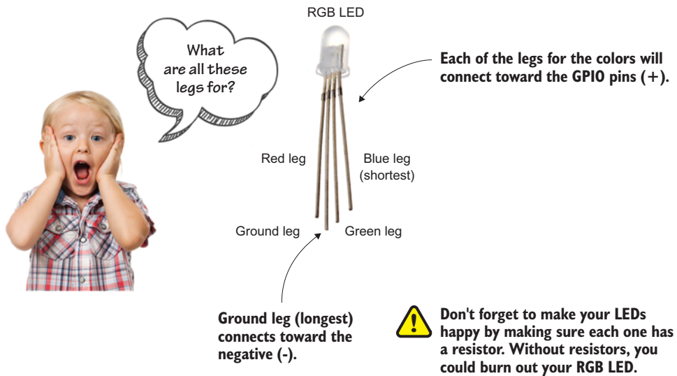
Figure 7.6 The RGB LED has lots of legs! The longest leg is the ground. The other ones are for red, green, and blue. This applies to what is called a common cathode RGB LED, which is what comes in Pi kits and what you'll find most commonly at electronics suppliers.
