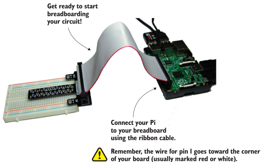
Figure 7.3 The Pi, breakout board, and breadboard setup. And you thought your desk was messy before!
