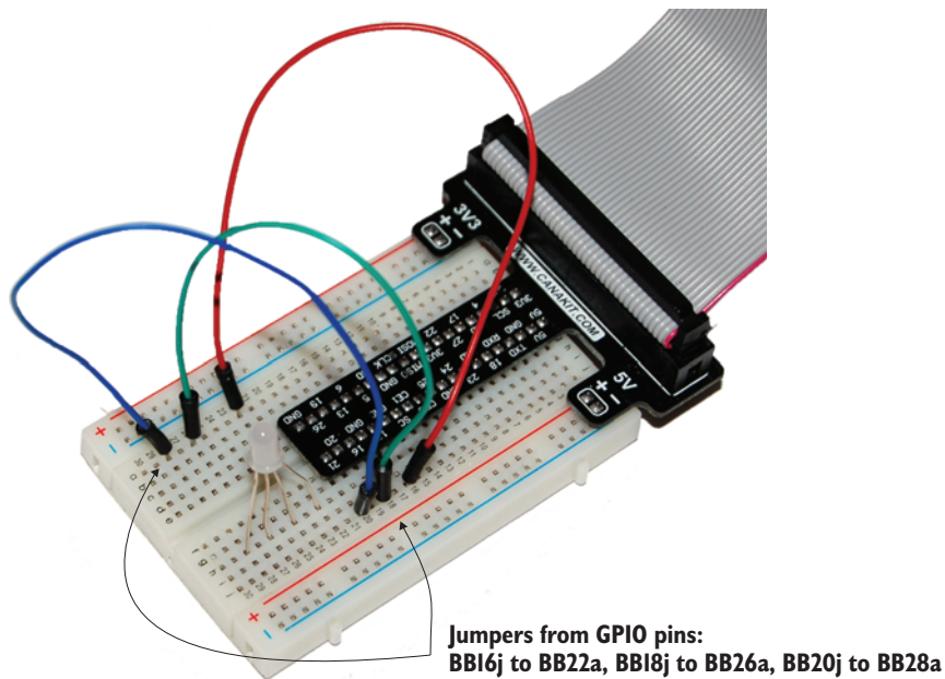
Figure 7.8 The jumpers connect the GPIO pins from your Pi to the RGB LED. If you have an earlier model Pi, you can use other GPIO pins. Just remember which ones you're using, and use these numbers when you program the Pi to turn the GPIO pins on and off.
