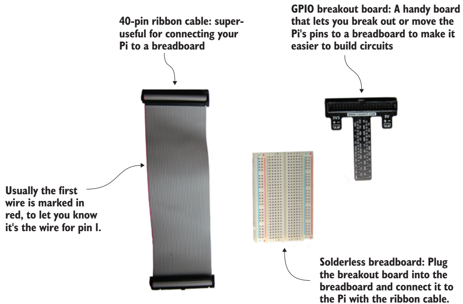
Figure 6.4 To easily create projects using your Pi's GPIO pins, you can connect the Pi to a breadboard using a ribbon cable and breakout board. The parts shown are examples of the ones commonly found in many Raspberry Pi kits.
