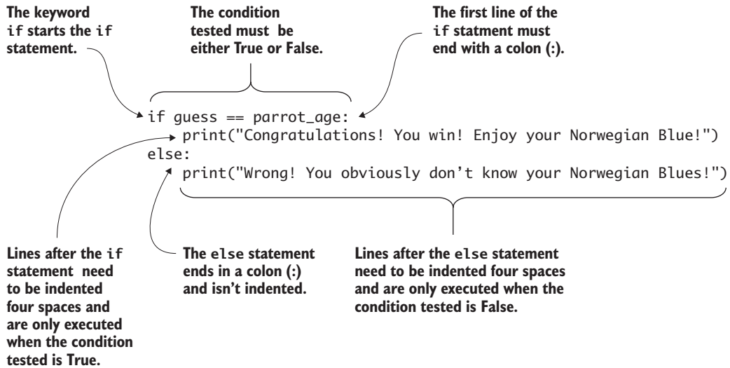
Figure 4.10 The if statement can control the flow of your programs. This example shows how an if statement can be used to display one message if guess is equal to the parrot's age or a different message if they aren't equal.
