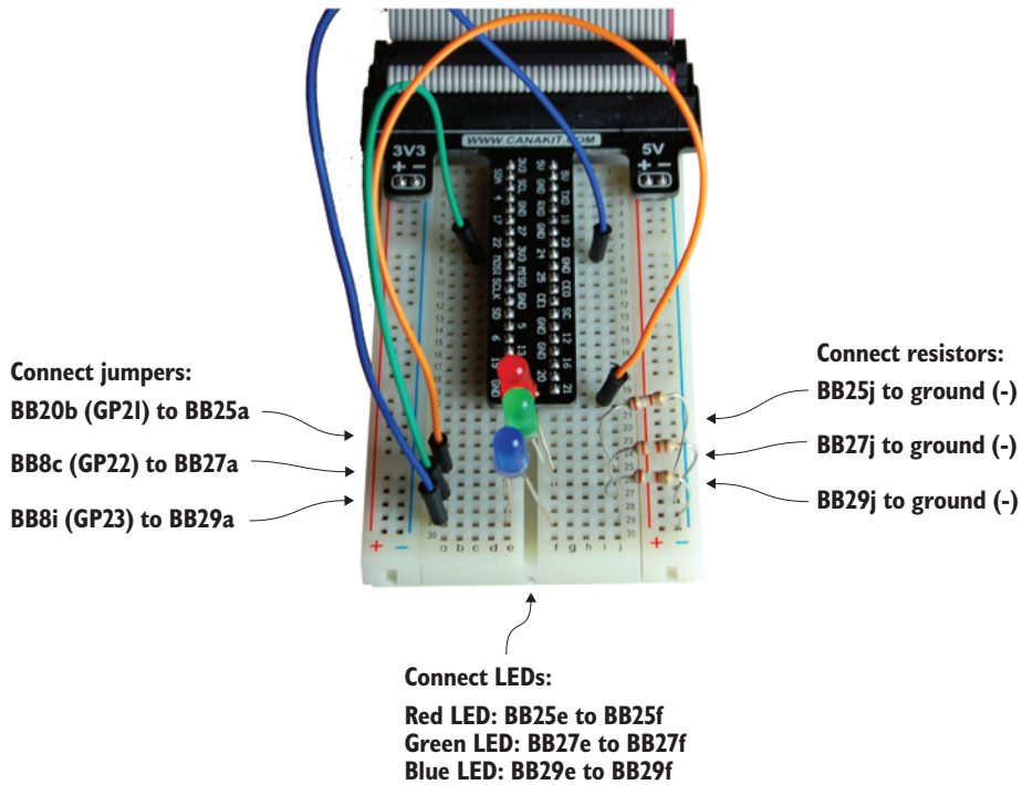
Figure 6.15 The three-LED circuit is built on the breadboard. Each LED and its corresponding resistor are placed in a row together. This example uses rows 25, 27, and 29.
