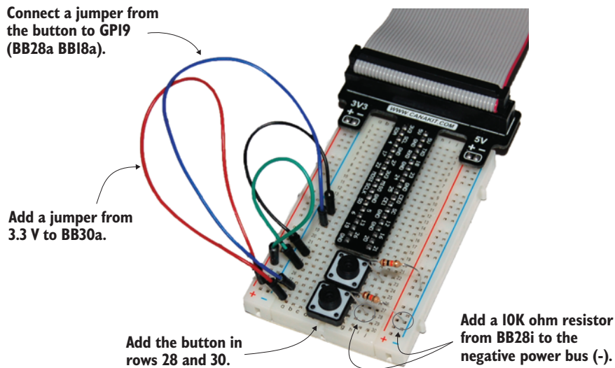
Figure 8.11 Add the second pushbutton just below the first one. The wiring is the same, but you'll connect it to GP19 (GPIO pin 19). Any available GPIO pin will work, but remember that your code will have to reflect the GPIO pins you select.
