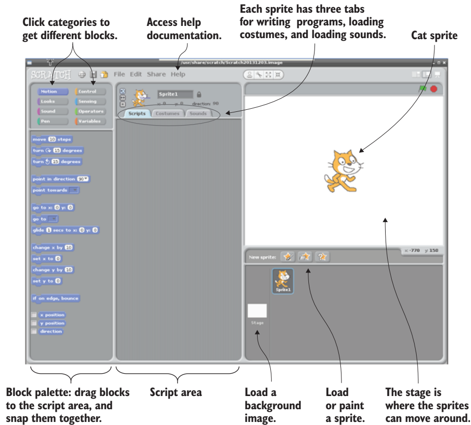
Figure 4.16 The Scratch interface is divided into an area for sprites to move around and a script area. You can create programs for your sprite by dragging blocks and connecting them in the script area.
