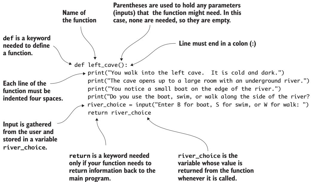
Figure 5.7 Functions simplify your code and can reduce repetition. Use the def keyword to create a new function, and indent the function code under it. If you need a function to return a value, include a return statement in the function.
