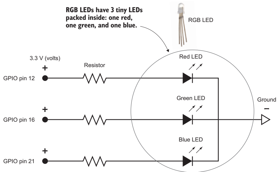
Figure 7.4 Circuit diagram for the Light Up Guessing Game project
