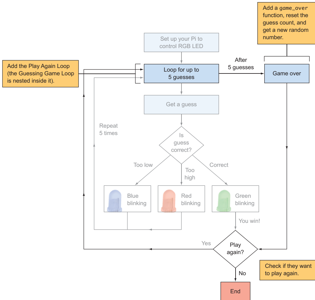
Figure 7.15 The Play Again Loop is wrapped around the Guessing Game Loop. After the player has exhausted their guesses or guessed the number correctly, they're asked if they want to play again. Depending on their answer, the game will either start over or end.
