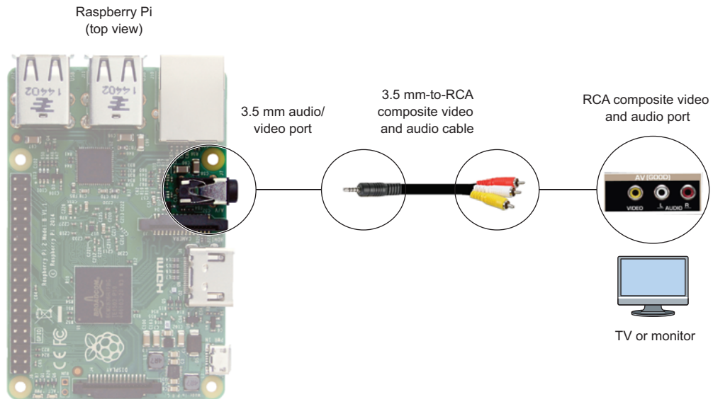
Figure B.9 The Raspberry Pi can be connected to a TV or monitor using an RCA video cable. The cable connects from the Pi's 3.5 mm audio/video port to the RCA video input port on the TV or monitor. Using the RCA connection produces a low-quality picture but can be a good option if you don't have a TV or monitor that supports HDMI.
