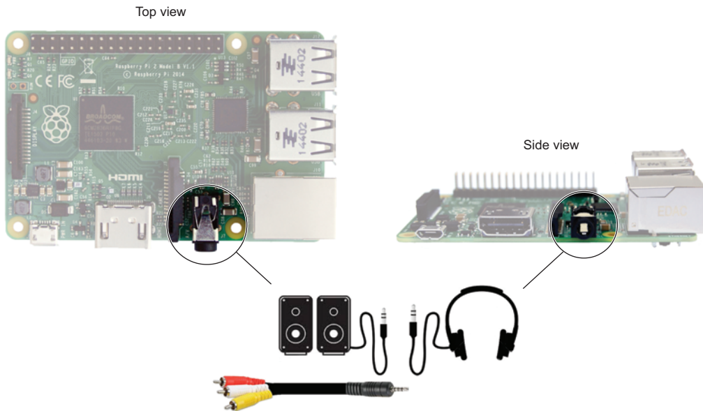
Figure B.4 The Raspberry Pi's 3.5 mm audio/video port is used to connect headphones or speakers for playing sounds. It can also function as a low-quality video output, if you purchase a 3.5 mm-to-RCA composite video adapter.
