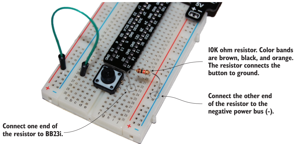
Figure 8.9 Add the resistor. Make sure its ends are pushed down into the breadboard holes.
