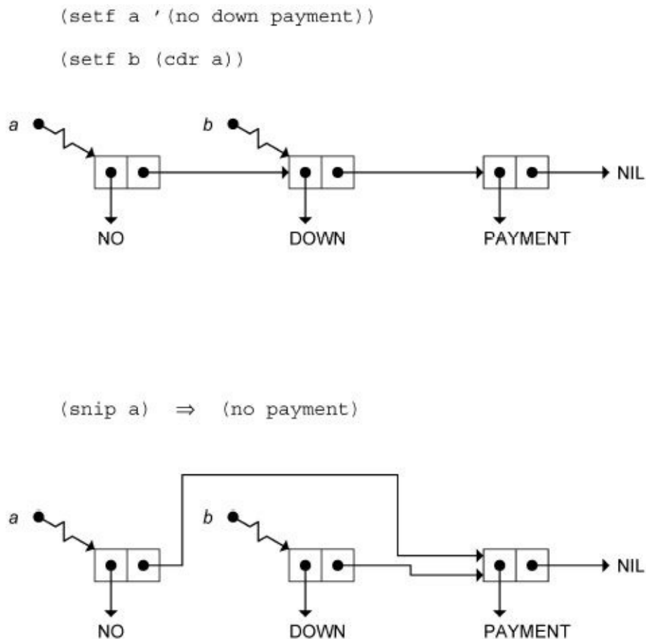
Figure 10-1 Effects of list surgery on the list (NO DOWN PAYMENT).
