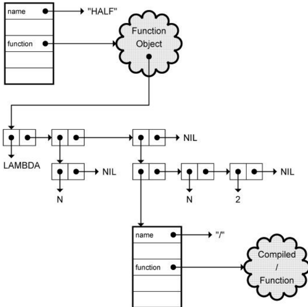
Figure 3-1 The internal representation of HALF.
