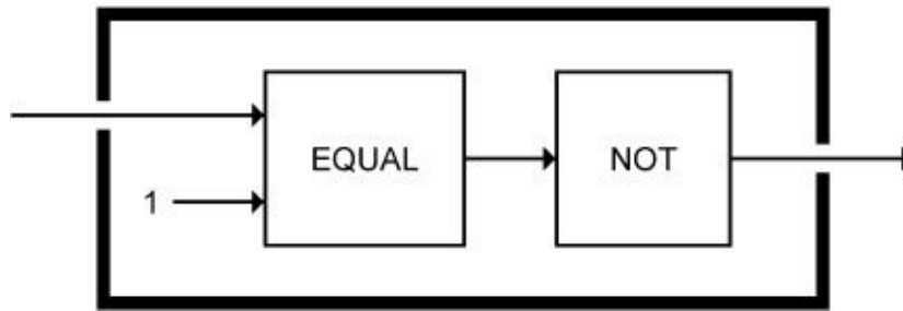
NOT-ONEP:
