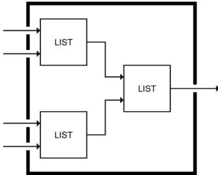
PAIR-OF-PAIRS:
