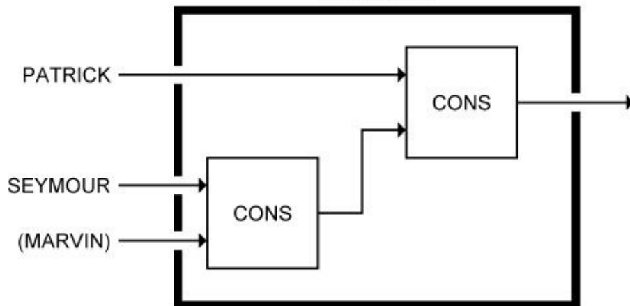
DUO-CONS:
