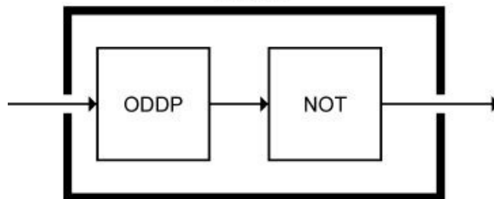
EVENP:
