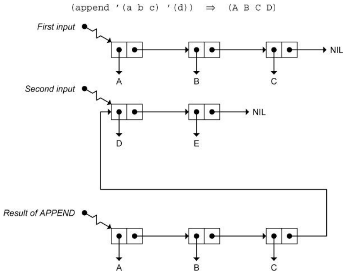
Figure 6-1 Result of appending (A B C) to (D E).
