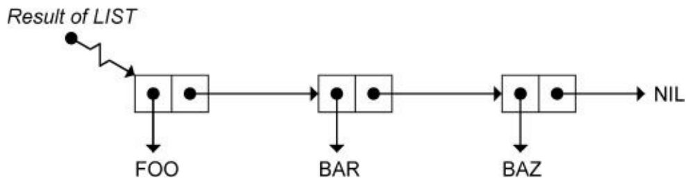
Figure 2-2 How LIST builds a new list.
