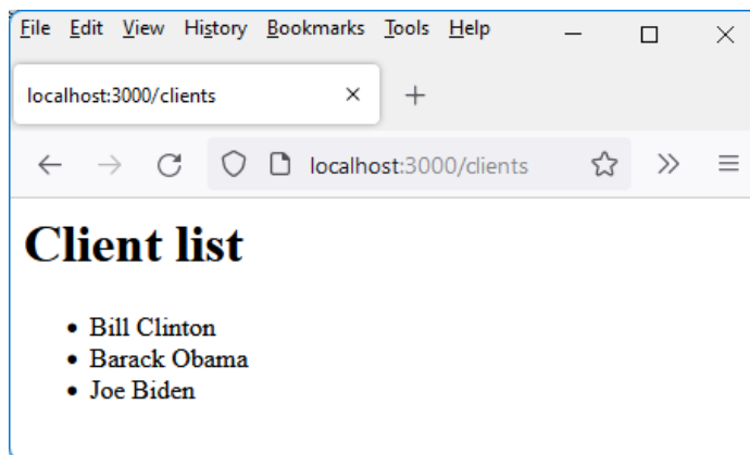
Figure 7.9 – View displayed using JADE syntax
