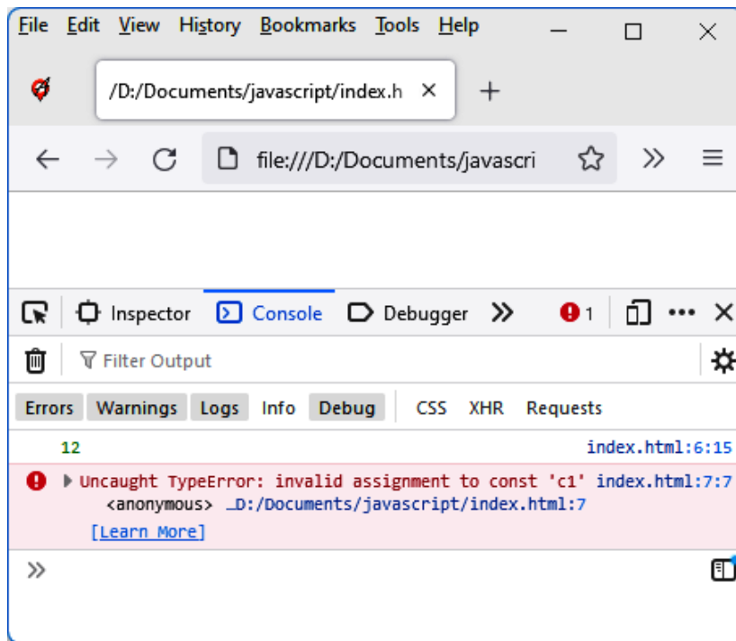
Figure 1.5 – Error when modifying a constant value
