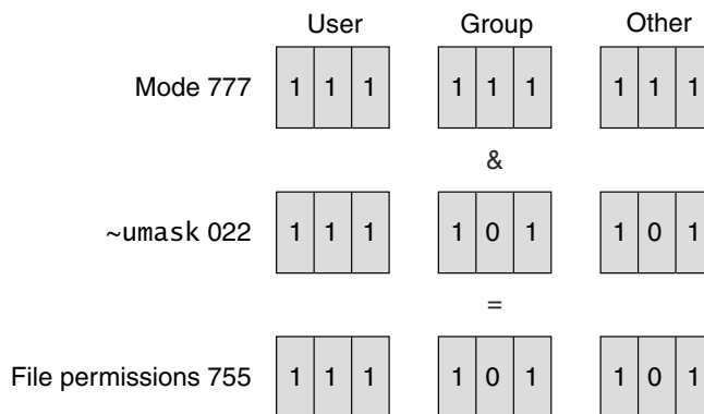
Figure 8.8 Restricting file permissions using umask
