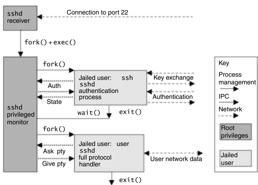
Figure 9.5 OpenSSH
