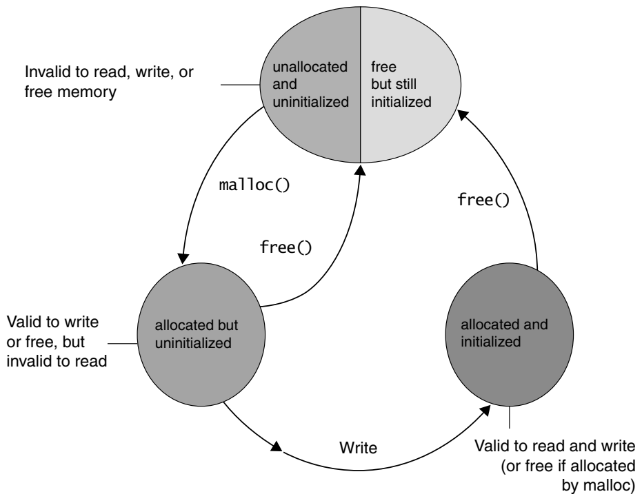
Figure 4.21 Memory access error checking (Source: [Rational 2003])
