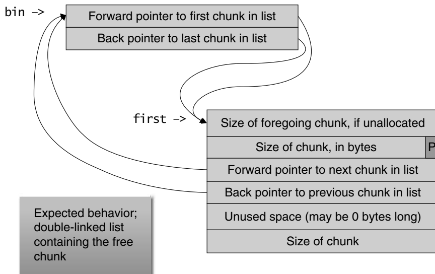
Figure 4.12 Bin with single free chunk
