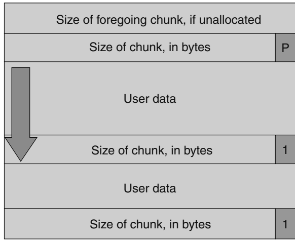
Figure 4.8 Buffer overflow overwriting boundary tag
