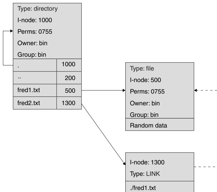
Figure 8.9 Symbolic link
