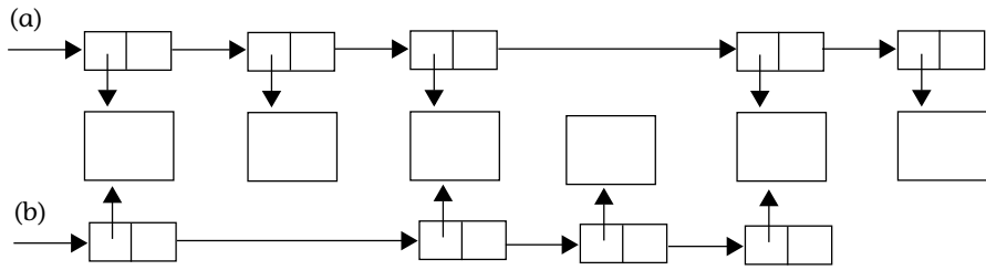
Figure 4.1 Linked-list data structures that share common elements
