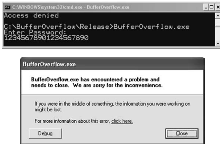
Figure 2.11 An improperly bounded Password array crashes the program if its character limit is exceeded.
