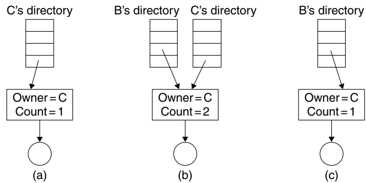
Figure 8.11 Shared file using hard links
