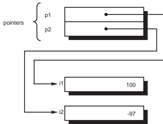
Figure 11.3 Structure containing pointers.
