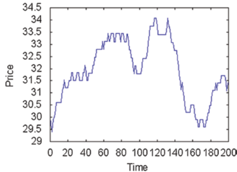
Figure 13-6. A random walk generated by the RandomWalkModel class with a starting price of $30
