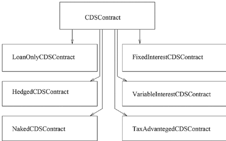
Figure 4-3. A class hierarchy rooted on the base class CDSContract
