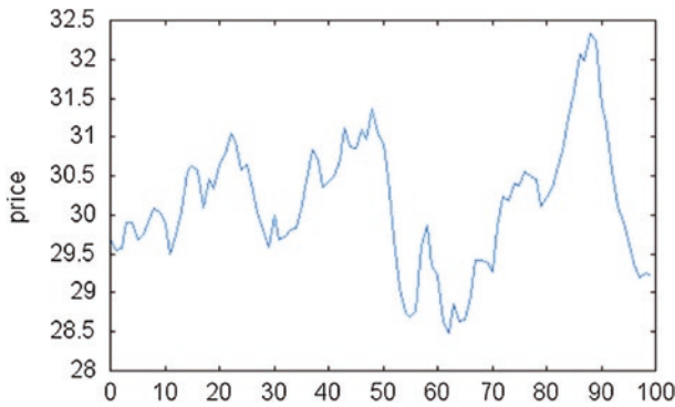
Figure 2-1. An example of random walk
