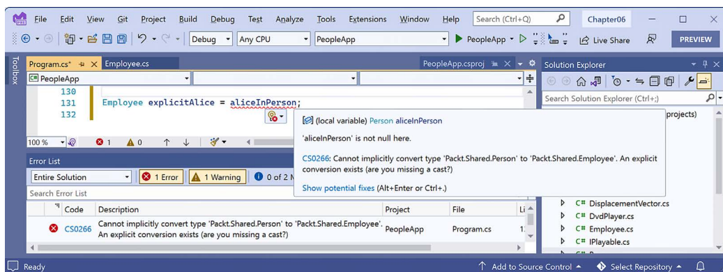
Figure 6.5: A missing explicit cast compile error
