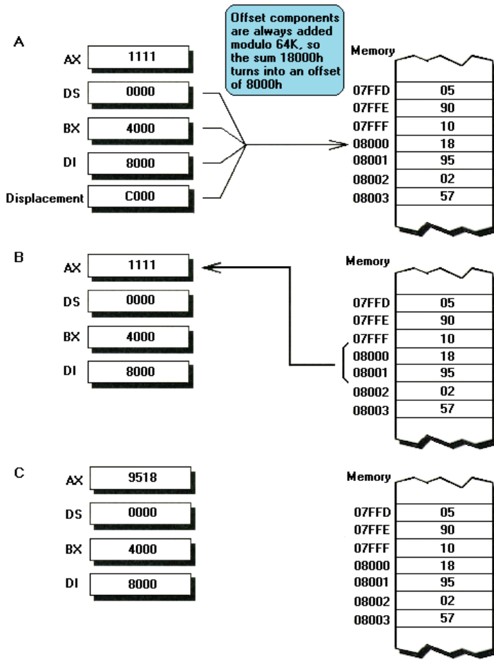
FIGURE 7.11 Offset components are added modulo 64K, with any carry out of bit 15 ignored, as illustrated by the execution of
