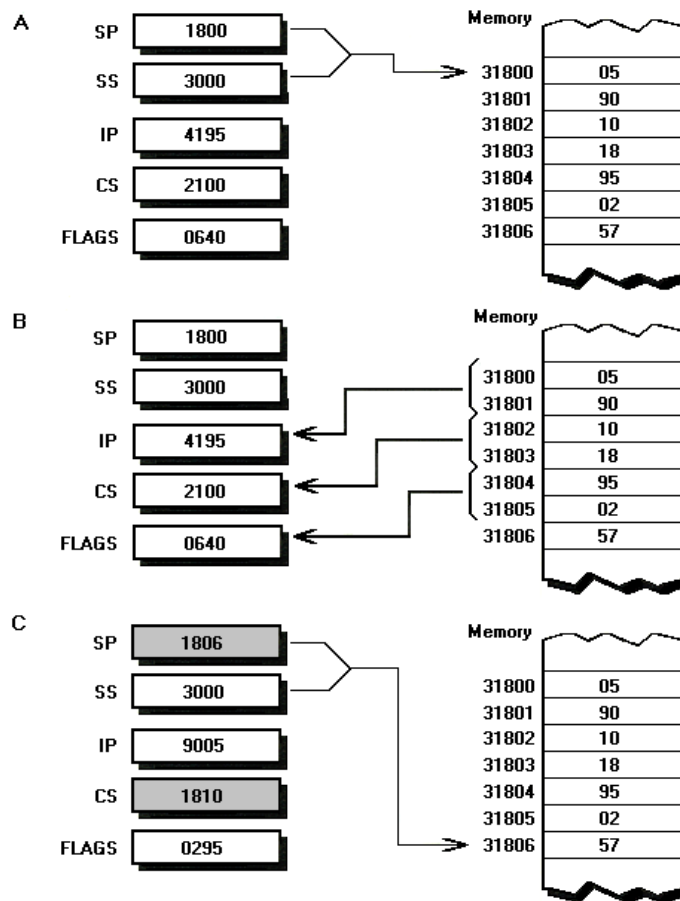
FIGURE 15.5 An example of the operation of iret . (A) The state of the PC before iret is executed. (B) The state of the PC as iret executes. (C) The state of the PC after iret is finished.
