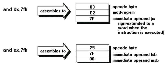
FIGURE 8.10 The word-sized mod-reg-rm immediate-addressing versions of adc , add , and , cmp , or , sub , sbb , and xor , when used with a register as the destination operand, can store values in the range -128 to +127 (inclusive) as bytes, then sign-extended them to words at run time, while the accumulator-specific immediate-addressing versions of those instructions cannot. Consequently, there's no advantage or disadvantage to using the accumulator-specific versions with operands in the range -128 to +127.
