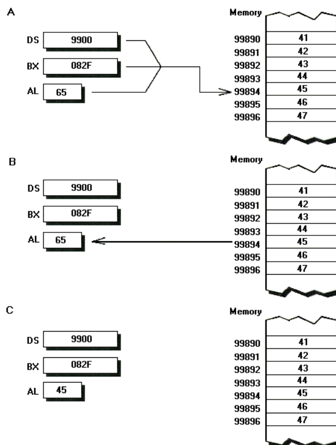
FIGURE 7.14 The operation of xlat . (A) xlat addresses memory by using the sum of BX and AL to form an offset, which points into the DS segment by default. (B) The addressed byte being read ( xlat works only with byte sized operands). (C) The addressed byte was read into AL, as is always the case with xlat .
