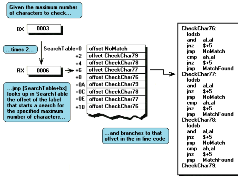
FIGURE 14.10 Listing 14-14 in action. Here a maximum search length of 3 is passed to SearchNBytes . That value is multiplied by 2 in order to look up the corresponding entry in the word-sized table SearchTable . A branch is then performed to the offset stored in the entry looked up; in this case, the entry contains the offset of CheckChar77 .
