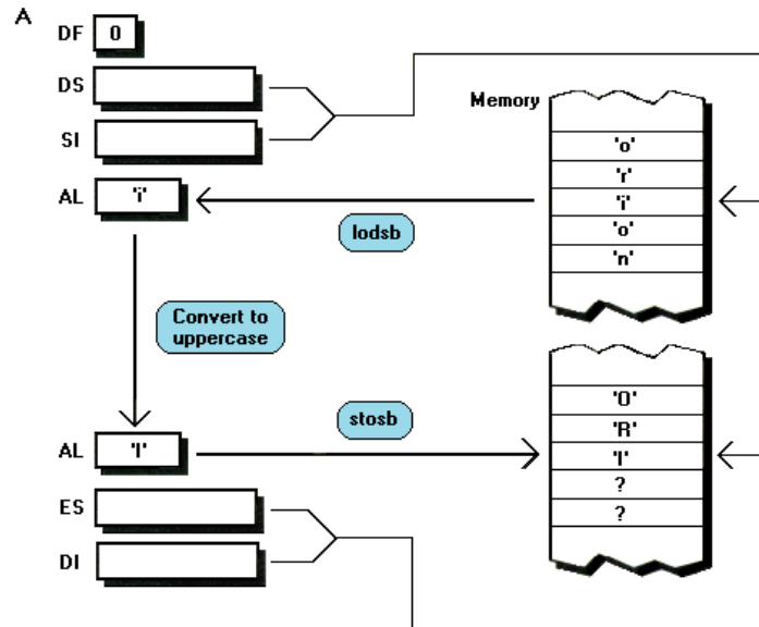
FIGURE 11.1 Together, lods and stos provide fast, flexible array and string handling. This figure illustrates that principle by showing the use of lods b and stos b to copy an array, converting all lower case characters to upper case in the process, with the following code:
