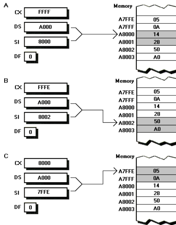
FIGURE 10.14 It is pointless to repeat a word-sized string instruction more than 8000h times, because the pointers will simply wrap back to addresses that were accessed earlier. (A) The first of 64K-1 repetitions of rep lodsw , which accesses address A000:8000. (In this and all other parts of this figure, the memory location being accessed is shaded.) (B) The second repetition, which accesses address A000:8002. (C) Repetition 8001h, which accesses address A000:7FFE. (D) Repetition 8001h, which accesses address A000:8000 for the second time. There's not much point in accessing a memory location twice with a single repeated string instruction! (Yes, I know—There's also not much point to repeating lodsw 8000h times, or even twice. I'm doing it here only to illustrate a point, which I'll state again: word-sized string instructions repeated more than 8000h times do double duty for no good reason.)
