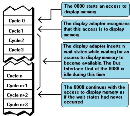
FIGURE 4.6 Both the video circuitry and the 8088 often try to access display memory at the same time. Display adapters resolve such conflicts by holding up 8088 accesses with wait states until the video circuitry no longer needs to access display memory. This figure is for illustrative purposes only, and is not intended to show the exact timings of 8088 operations.
