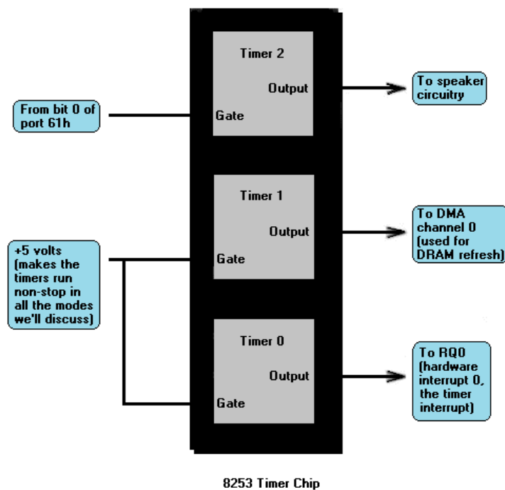
FIGURE 2.1 The configuration of the 8253 timer chip in the PC. Of the 8253's three timers, only timer 2 is wired so that its gate input is under program control; the gate inputs of timers 0 and 1 are always enabled, so there is no documented way to get either timer 0 or timer 1 to stop counting. Only timer 0 is connected so that it is capable of generating an interrupt.
