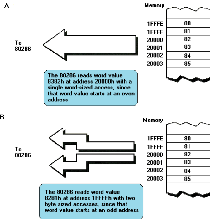
FIGURE 15.1 The data alignment cycle eater. (A) the 80286 needs just one word-sized memory access to read or write a word of memory that starts at an even address. (B) However, the 80286 must perform two byte-sized memory accesses—which together take twice as long as one word-sized access—when asked to read or write a word of memory that starts at an odd address. Apart from execution time, the whole process is transparent to instructions that access memory, which know only that a word of memory has been accessed in either case.
