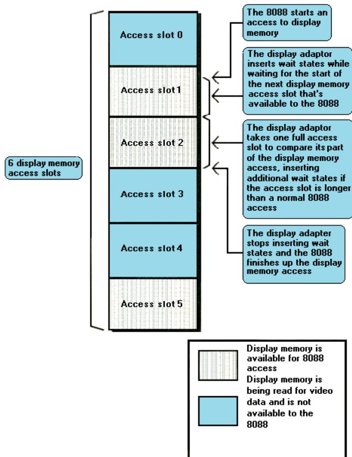
FIGURE 4.8 Accesses to display memory are available only at fixed intervals and are of fixed lengths. both the intervals and the lengths are controlled by the display adapter, and are the same regardless of the speed of the computer in which the display adapter is installed. This figure is for illustrative purposes only, and is not intended to show the exact timings of 8088 operations.
