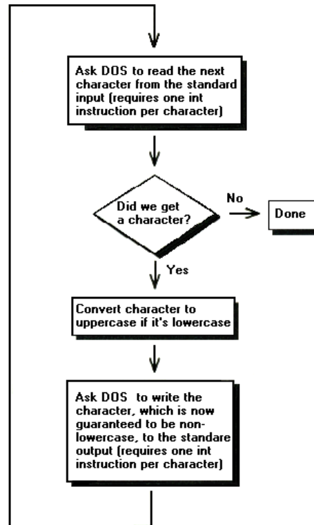
FIGURE 14.3 It's easiest—but not fastest—to communicate with DOS one character at a time, letting DOS handle the details of buffering data.
