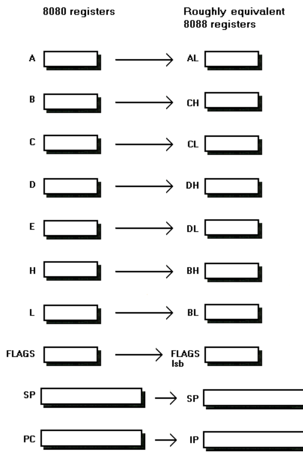
FIGURE 8.1 The general correspondence of 8080 registers to 8088 registers indicates the strong influence of the 8080 on the design of the 8088.
