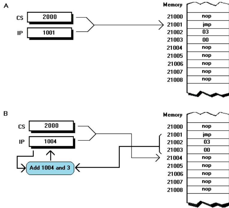
FIGURE 12.2 Most of the 8088's jump instructions use relative branching, where the destination address is specified as a displacement from the offset pointed to by the current instruction pointer. This figure shows the steps that occur as a jmp , which performs a relative branch to offset 1007h executes, with the thin lines showing how IP advances as the execution of the jmp progresses. (A) Here, jmp is just starting. (B) The branch is taking place, with IP having advanced past the opcode and displacement bytes as they're fetched; the displacement is added to IP after IP has advanced past the last byte of the instruction. (C) The branch is complete, with IP pointing to the branched to instruction.
