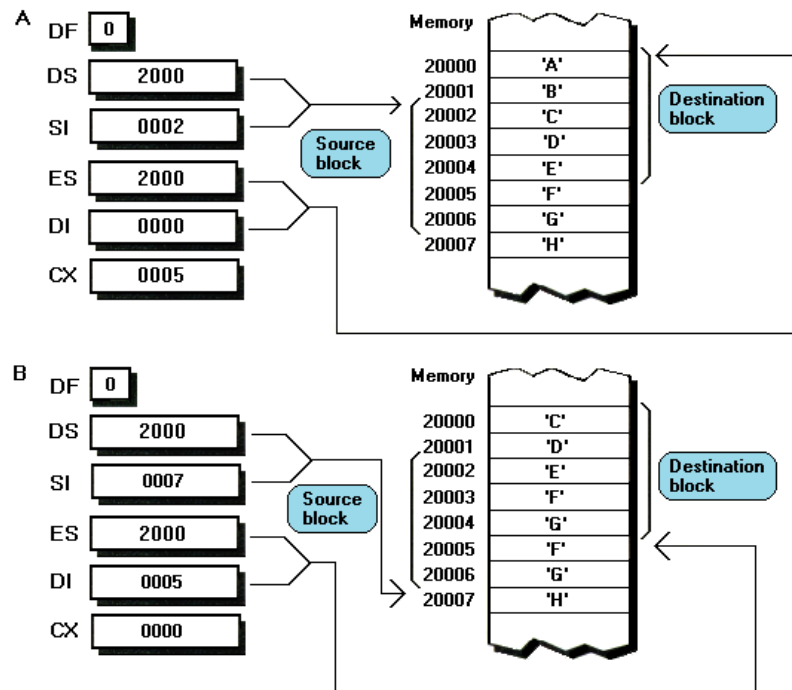
FIGURE 11.2 When overlapping blocks are the source and destination for rep movsb , the direction in which the copy must proceed depends on the direction of overlap. In this figure the source block starts at a higher address than the destination block, so the copy must proceed from lower addresses to higher addresses. This is the mode of operation of the string instructions when DF is equal to 0, as it normally is. (A) The state of the PC before rep movsb is executed to copy such an overlapping block. (B) The state of the PC after the copy is completed.
