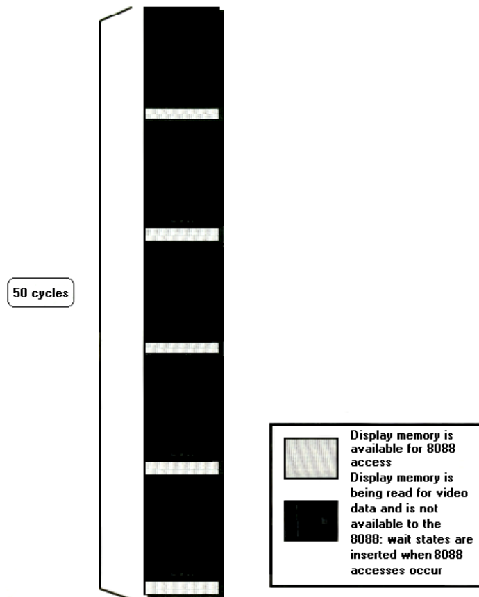
FIGURE 4.7 The video circuitry, which scans display memory for pixel data, can take as much as about 90 percent of available display memory access time, leaving as little as about 10 percent of all display memory access free for the use of the 8088.
