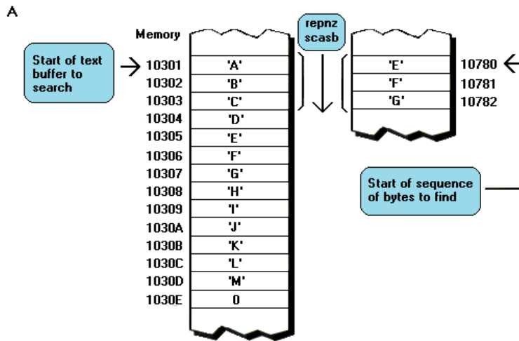
FIGURE 11.15 We can speed up the search for a fixed-length sequence of bytes in a text buffer considerably by using repnz scasb to eliminate many buffer locations as potential sequence-starting locations. This is accomplished by using repnz scasb to search the text buffer for the first character of the sequence, and the using repz cmps to check only those potential sequences that have been prequalified by repnz scasb . (A) The use of repnz scasb to eliminate the first 4 bytes of the buffer as potential sequence-start bytes. (B) The single repz cmps needed to compare the remainder of the match found by repnz scasb . This approach eliminates the need to expand loops and executions of repz cmps on those buffer locations that don't begin with the sequence-starting byte and therefore can't possibly start the desired sequence. In this figure, just one repnz scasb and one repz cmps would be required to find the matching sequence starting at 10305.
