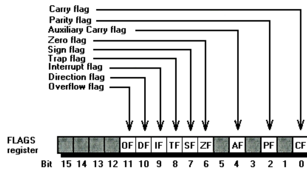
FIGURE 6.2 The 8088's flags
