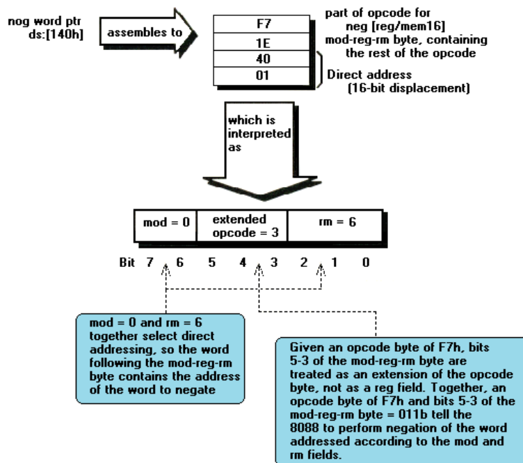
FIGURE 7.9 The interpretation of the bytes assembled for instruction neg word ptr ds:[140h] , illustrating that in single-operand mod-reg-rm instructions. Bits 5 to 3 of the mod-reg-rm byte serve as an extension of the opcode byte rather than as the reg field.
