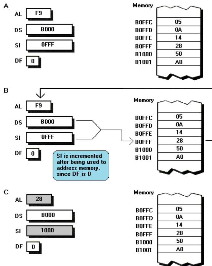
FIGURE 10.1 The operation of lodsb with DF set to 0. (A) The state of the PC before lodsb is executed. (B) The data and addressing paths as lodsb executes. (As usual, data movement is shown with heavy lines, while addressing is shown with light lines.) (C) The state of the PC after lodsb is finished, with altered registers shaded. Note that SI is determined when DF is 1. The instructions lodsw and lodsb are identical, except that with lodsw AX, rather than AL, is loaded and SI is incremented or decremented by 2 rather than by 1.
