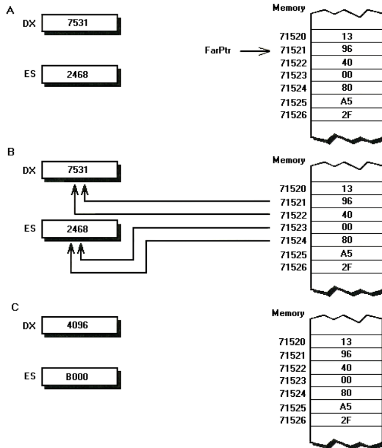
FIGURE 7.5 The 8088 always considers the least significant word of doubleword sized memory access to be at the lower memory address. (A) The state of the PC as les dx,dword ptr [FarPtr] begins. (B) Memory being accessed with the least significant word at the lower memory address. (C) The data from the least significant word is indeed loaded into DX and the data from the most significant word is loaded into ES.
