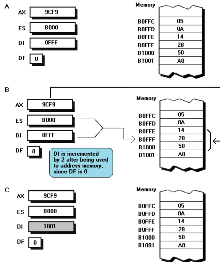
FIGURE 10.2 The operation of stosw with DF set to 0. (A) The state of the PC before stosw is executed. (B) The data and addressing paths as stosw executes. (C) The state of the PC after stosw is finished, with altered registers and memory locations shaded. Note that DI is decremented when DF is 1. The instruction stosb is identical to stosw , except that AL rather than AX is written to memory and DI is incremented or decremented by 1 rather than 2.
