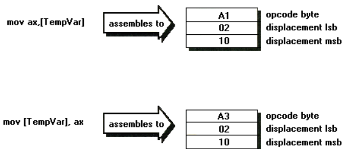
FIGURE 8.3 The accumulator specific direct addressing instructions are each only 3 bytes long, 1 byte shorter (and 4 to 5 cycles faster) than the equivalent instructions that use mod-reg-rm direct addressing.
