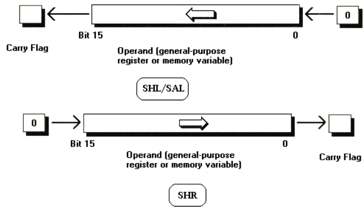
FIGURE 9.4 The shl (also known as sal ) and shr instructions shift the bits in the operand to the left and right, respectively, copying the bit shifted out to CF and shifting a 0 bit into the operand. This figure illustrates a 16-bit operation; 8-bit operands can be shifted as well.
