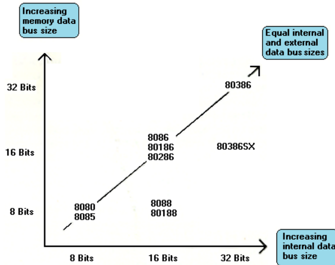
FIGURE 3.5 Most of the processors in the 8086's extended family have identical internal and external data bus sizes. The 8088 is unusual in that it has a 16 bit internal data bus but an 8 bit external data bus, a mismatch that makes the 8088 a significantly slower processor than the 8086, especially when running high performance assembler code. Under certain circumstances, code can run as much as four times more slowly on an 8088 than on an 8086.
