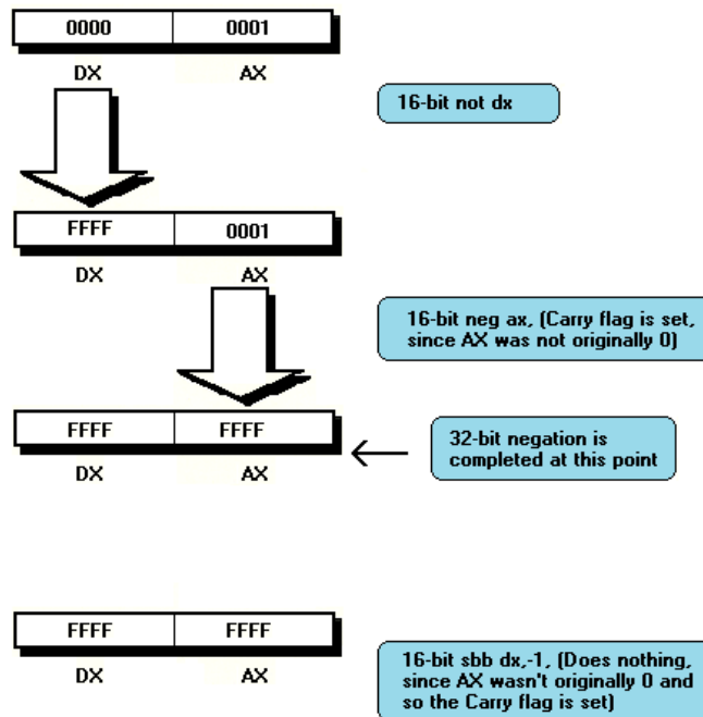
FIGURE 13.4 When performing a 32-bit negate with not dx neg ax sbb dx,-1 sbb dx,-1 does nothing when AX is not initially 0.
