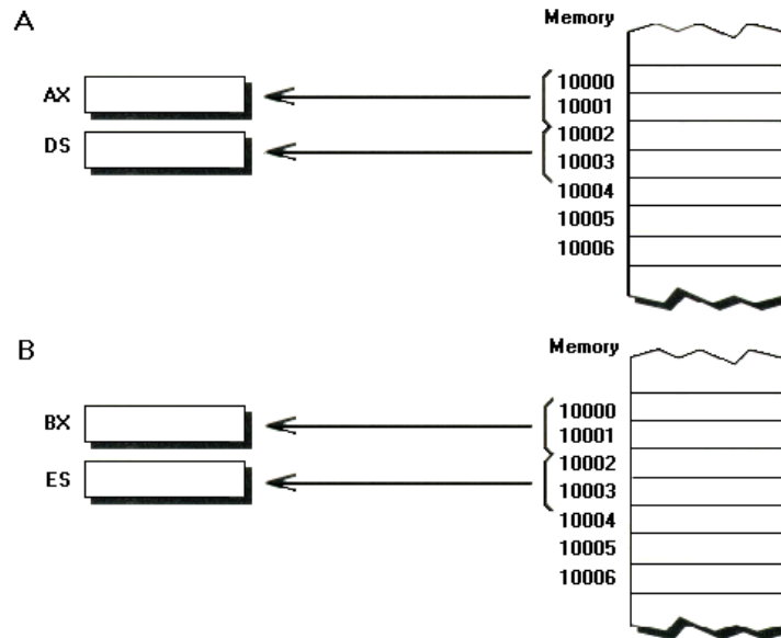
FIGURE 7.3 (A) The operation of lds , which loads both DS and a general purpose register (AX in this case) at once from a doubleword of memory. (B) The operation of les , which loads both ES and a general purpose register (BX in this case) at once.
