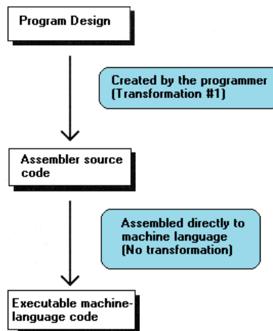
FIGURE 1.2 Only one transformation is required when creating an assembler program, and that single transformation is completely under the programmer's control. Assemblers perform no transformation from source code to machine language; instead, they merely map assembler instructions to machine language instructions on a one-to-one basis. As a result, the programmer is able to produce machine language code that's precisely tailored to the needs of each task a given application requires.
