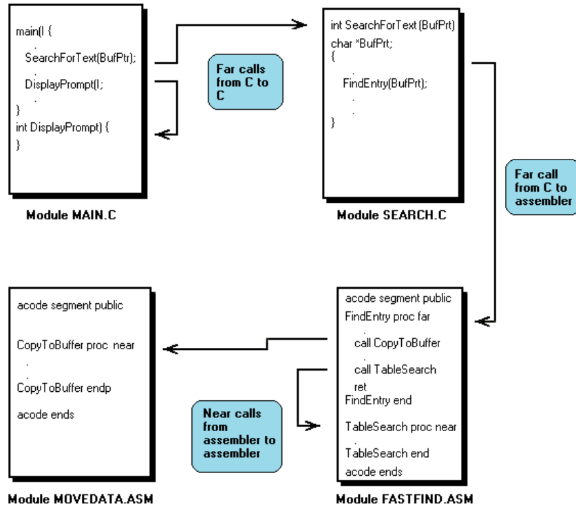
FIGURE 14.1 In large-model programs written primarily in C or Pascal, all the assembler code can be placed in a single segment, allowing near branches to be used within the assembler or Pascal code is involved.
