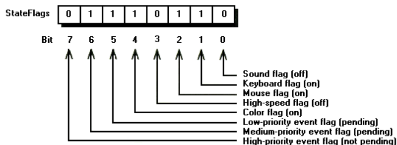
FIGURE 14.6 The byte sized variable StateFlags contains eight separate 1-bit flags. The interpretation of the current state of each flag is shown in parentheses.
