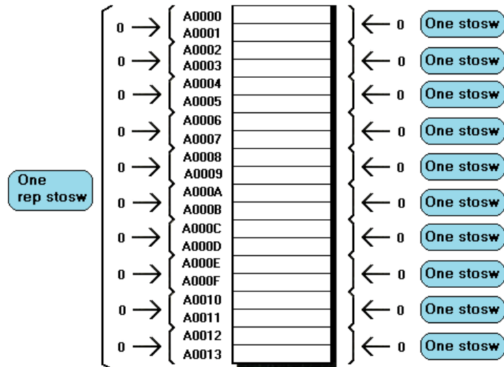
FIGURE 10.6 Here rep stosw clears 10 words of memory, with one 2-byte prefix/instruction pair doing what would otherwise take ten 1-byte stosw instructions. The rep prefix is capable of much more; a single repeated string instruction can be executed up to 64K-1 times.
