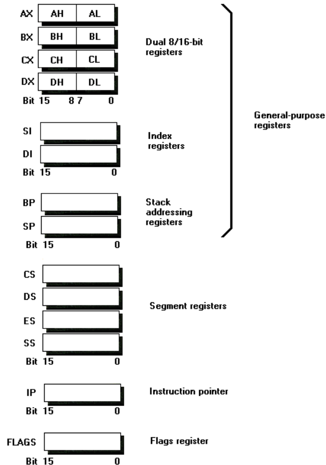
FIGURE 6.1 The 8088's register set
