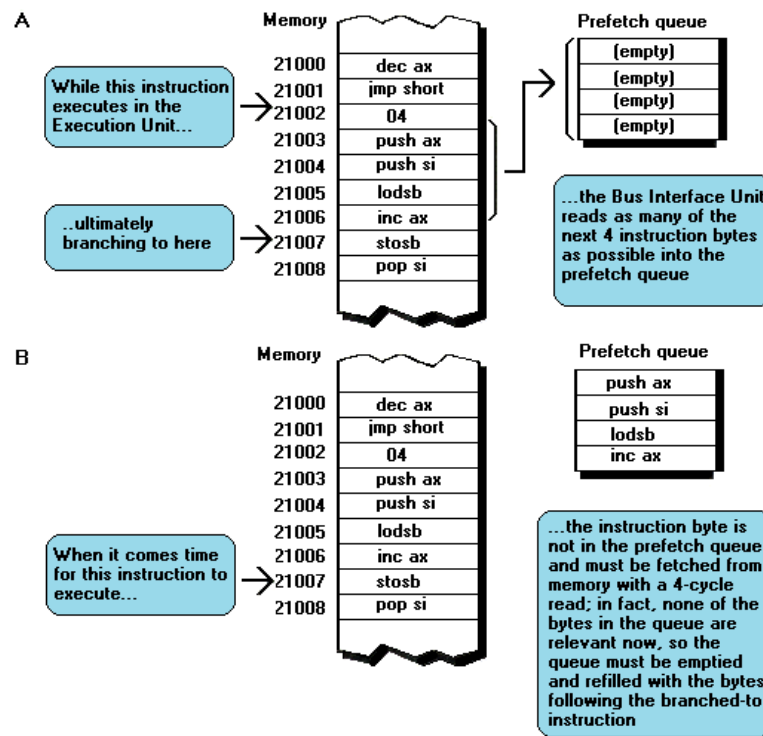
FIGURE 12.5 When the EU performs a branch the prefetch queue is always emptied.
