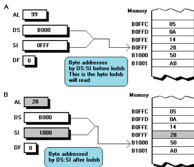
FIGURE 10.9 String instructions leave their pointers pointing one location past the last byte or word accessed. (A) The state of the PC before lods executes. (B) The state of the PC after lods executes. The byte read by lods is shaded. It's clear that lods advances SI to the point 1 byte past the location read, because DS:SI does not point to the shaded location but rather to the adjacent memory address.
