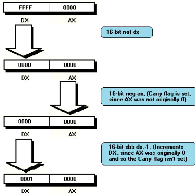
FIGURE 13.5 When performing a 32-bit negate with not dx , neg ax , and sbb dx,-1 , sbb dx,-1 increments DX if and only if AX is initially 0.
