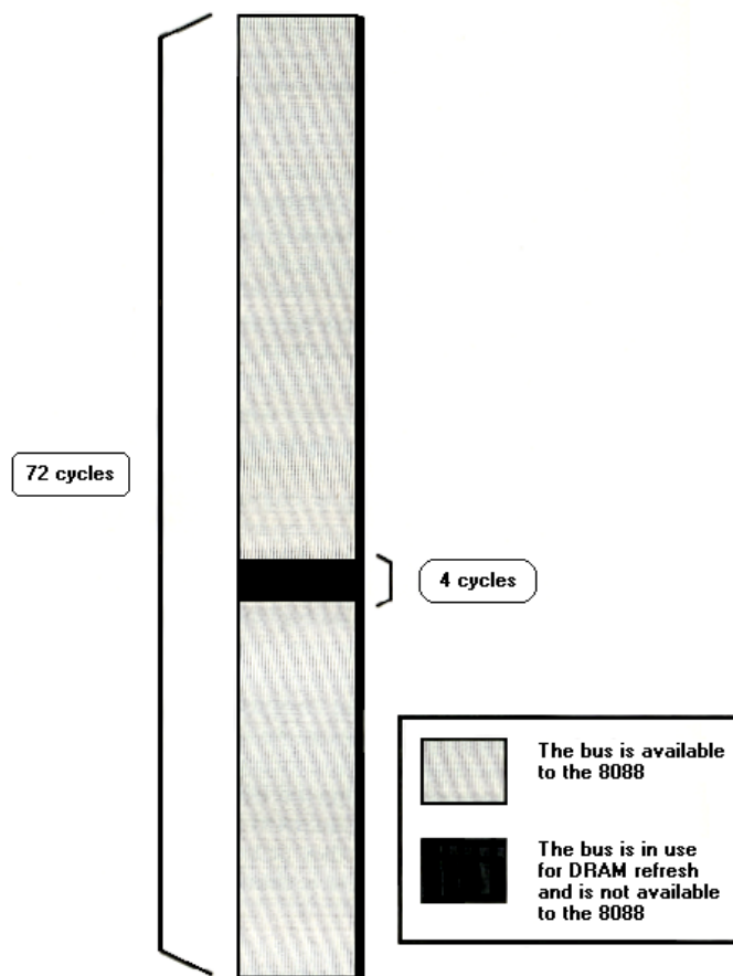
FIGURE 4.5 The PC's bus is given over to providing dynamic RAM (DRAM) refresh for at least 4 cycles out of every 72 cycles.
