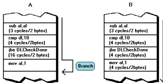
FIGURE 13.7 The two possible instruction sequences that can be executed by sub al,al cmp dl,10 jbe DLCheckDone DLGreaterThanOrEqualTo10: mov al,1 DLCheckDone: (A) The instructions executed when DL is less than or equal to 10. (B) The instructions executed when DL is greater than 10.
