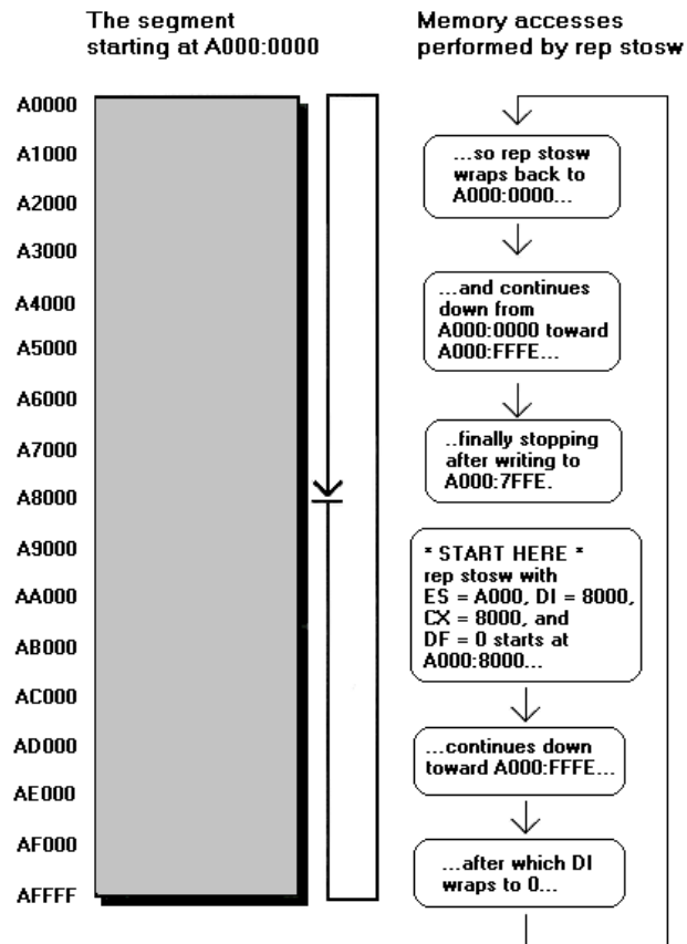
FIGURE 10.13 Regardless of the offset within a segment at which a repeated string instruction starts, only the 64K bytes starting at offset 0 within that segment can be accessed by that string instruction. Here stosw is repeated 8000h times starting at offset 8000h. After 4000h repetitions, DI reaches the end of the segment pointed to by ES and wraps back to the start of the segment. DI ultimately winds up right back at the same offset—8000h—at which it started, and it is the 64Kb block starting at ES:0 that is accessed by rep stosw , rather than the 64Kb block starting at A000:8000, the address to which ES:DI initially pointed.
