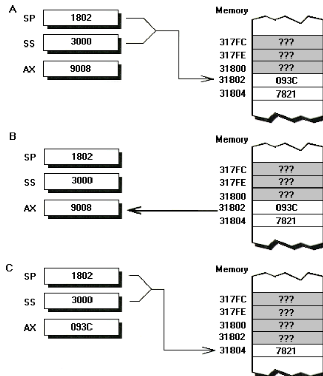
FIGURE 7.13 It might appear that popped data still exists in memory, since pop merely adds 2 to the stack pointer without altering memory in any way, but that's not the case. When a value is popped off the stack, it can no longer be relied on to exist in memory, because interrupts may occur any time, expanding the stack and wiping out any data lying around the area of memory just past the top of the stack. (A) The stack just before a pop , with the value 93Ch stored at address 31802, the top of the stack. (B) The value on top of the stack being popped into AX. (C) The completed pop , with SP pointing 2 bytes higher in memory and with the value 93Ch no longer shown at 31802. In truth, that value may still be there – but it may also have been wiped out by an interrupt, and there's no way to show which is the case at any given time. Note that all data past the top of the stack is shaded in all three figures, indicating that such data may change at any time.
