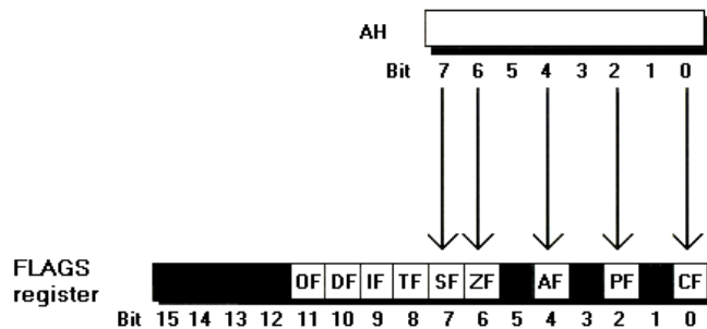
FIGURE 8.13 The sahf instruction copies the AH register to the lower byte of the 8088's flags register, reversing the action of lahf .
