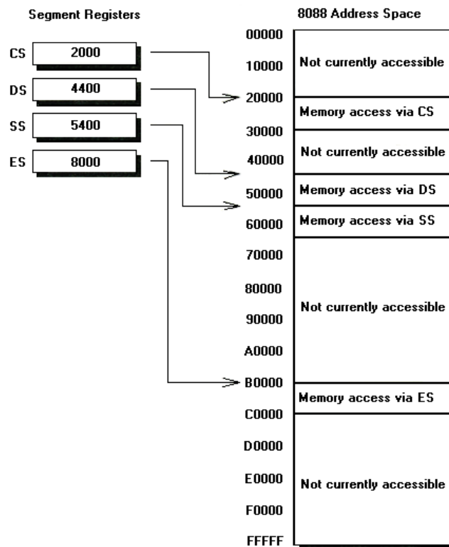
FIGURE 7.2 Out of the one-million-plus bytes that the 8088 can address, only the data in the four 64-Kb blocks pointed to currently by the segment registers can be accessed without reloading a segment register.
