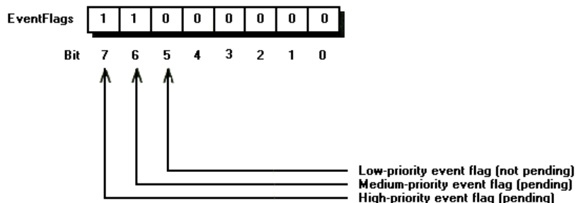
FIGURE 14.7 The byte sized variable EventFlags contains three separate 1-bit flags in bits 7 to 5, with bits 4 to 0 always set to 0. The interpretation of the current state of each flag is shown in parentheses.
