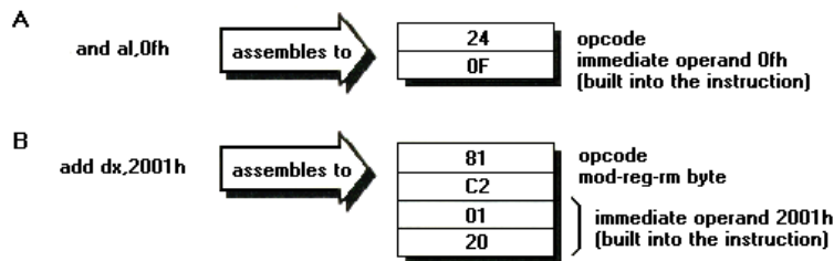
FIGURE 7.12 Immediate operands are built right in to instructions coming immediately after opcode bytes or mod-reg-rm bytes (A) The immediate operand 0Fh follows the opcode byte in and al,0fh . (B) The immediate operand 2001h follows the mod-reg-rm byte in add dx,2001h
