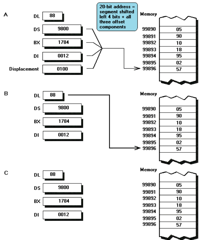
FIGURE 7.7 The operation of the instruction mov [bx-di+100h], dl , which uses base+index+displacement addressing ( A ) The three offset components, BX, DI, and the displacement of 100h, are added together, and the resulting offset is added to DS shifted left 4 bits. The 20 bit result is used to address the byte of memory written to in ( B ). ( C ) The completed operation, with the value in DL written to the addressed byte. Note that displacements are built in to instructions, coming immediately after mod-reg-rm bytes.
