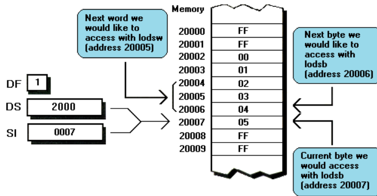
FIGURE 11.6 After lodsb is executed with DF set to 1 (causing SI to decrement), the address of the next byte we would want to access with lodsb and the address of the next word we would want to access with lodsw are not the same. This figure shows that after reading the byte at 2000:0007, the next byte we would want to access is at 2000:0006, whereas the next word we would want to access is at 2000:0005. (Reading the word at 2000:0006 gets the byte read by the initial lodsb —the byte at 2000:0007—again, along with the byte at 2000:0006. What we want are the bytes at 2000:0005 and 2000:0006, which form the word immediately preceding the byte at 2000:0007 that was read with the initial lodsb .) This can cause problems when byte- and word-sized string instructions are mixed when DF is set to 1.
