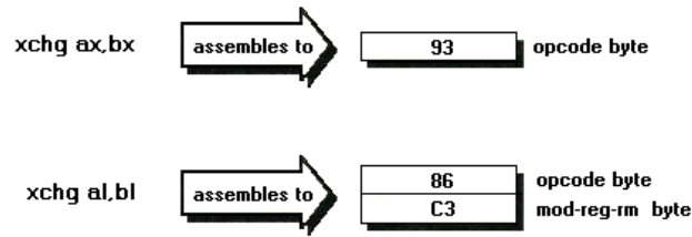
FIGURE 8.11 The AX specific form of xchg is 1 byte shorter and 1 cycle faster than the mod-reg-rm form.
