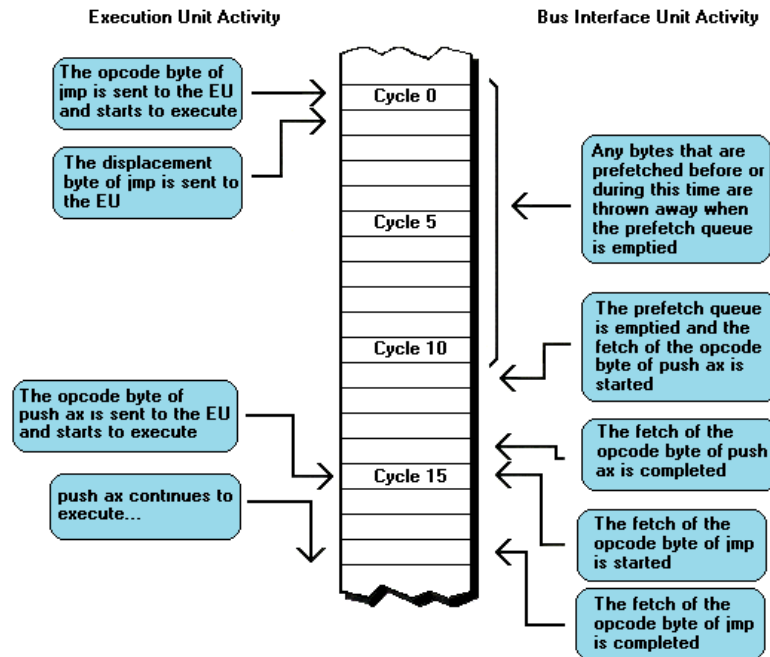
FIGURE 12.7 Under the right circumstances, the prefetch queue cycle eater doesn't take any cycles after a branch. In this figure, the jmp instruction ends by fetching the opcode byte of push ax , which immediately starts to execute. The instruction push ax takes 15 cycles to execute but uses only 8 of those cycles to access memory, leaving 7 cycles free for instruction prefetching. As a result, the BIU is able to prefetch at least the opcode byte of the following jmp instruction, allowing that instruction to start without any instruction-fetch delay. This figure is for illustrative purposes only and is not intended to show the exact timings of 8088 operations.
