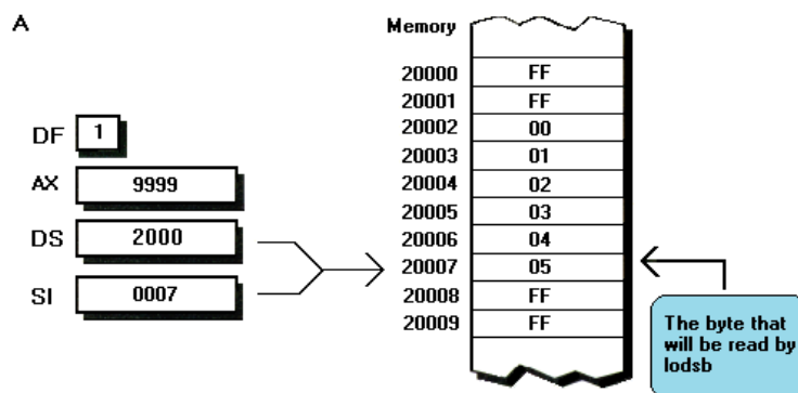
FIGURE 11.7 When DF is 1, problems can occur when byte- and word-sized string instructions are mixed, since the address of the next byte is not the same as the address of the next word. This figure showed that the last 3 bytes of a memory block are read incorrectly with the following code:
