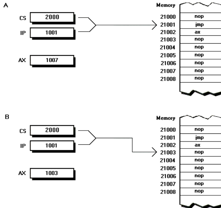
FIGURE 12.1 The jmp reg16 instruction is one of the few jump instructions that performs an absolute branch, that is a branch to a specific offset in the code segment. Instead, most of the 8088's jump instructions use relative branching (as shown in Figure 12.2). This figure shows the steps that occur as jmp ax branches, with the thin lines showing how IP advances as the execution of jmp ax progresses. (A) Here, jmp ax is just starting. (B) AX is copied into IP after IP has advanced past (and allowed the fetching of) the last byte of the jmp instruction, the mod-reg-rm byte that specifies AX as the source register. (C) The branch is complete, with IP pointing to the branched-to instruction.
