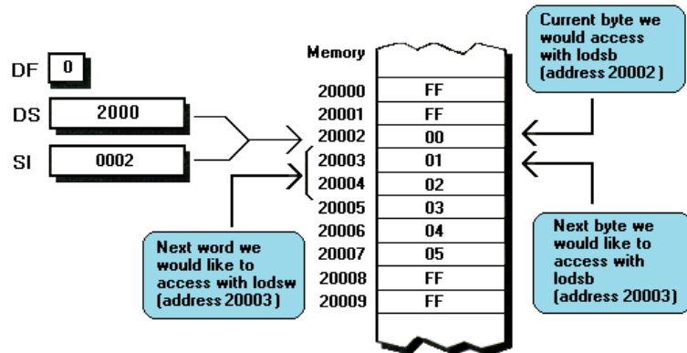
FIGURE 11.9 After lodsb is executed with DF set to 0 (causing SI to increment), the address of the next byte we would want to access with lodsb and the address of the next word we would want to access with lodsw are exactly the same. In this figure, after the byte at 2000:0002 is read, both the next byte and the next word are at 2000:0003. (Reading the word at 2000:0003 gets the bytes at 2000:0003 and 2000:0004, which are the bytes immediately following the byte at 2000:0002 that was read with the initial lodsb .) As a result, no nasty problems result from mixing byte- and word-sized string instructions when DF is 0. As we've seen over the last few figures, the same is most decidedly not true when DF is 1.
