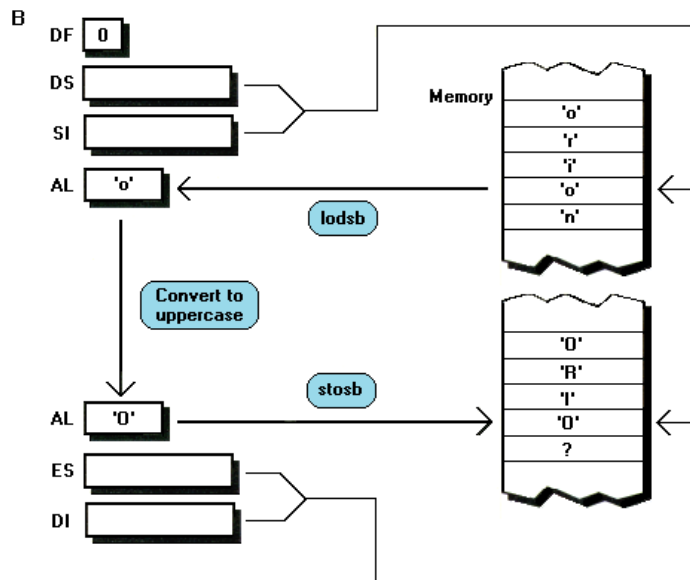
FIGURE 11.1 (continued) (A) The copying and conversion of the third character in the array. (B) The copying and conversion of the fourth character. These two figures illustrate a significant advantage of using lods/stos for array and string processing, which is that, like all string instructions, lods and stos automatically advance their pointers.
