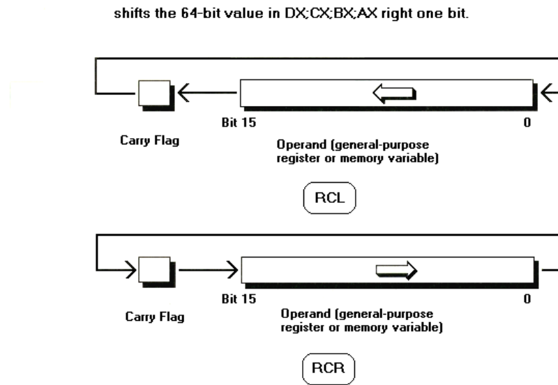
FIGURE 9.3 The instructions rcl and rcr shift the bits in the operand to the left and right, copying the bit shifted out to CF and shifting CF into the operand. This figure illustrates a 16-bit operation; 8-bit operands can be rotated as well.
