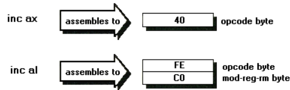
FIGURE 9.1 The 16-bit register-only versions of inc and dec are only 1 byte long and execute in just 2 cycles. By contrast, the mod-reg-rm versions of inc reg and dec reg are 2 bytes long and execute in 3 cycles.
