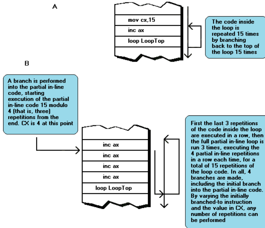
FIGURE 13.12 Branched-to partial in-line code can handle any number of repetitions. The trick with branched-to partial in-line code is that any odd portion of the desired repetition count—any portion that is not an even multiple of the number of repetitions per partial in-line loop—is handled by initially branching to perform that odd number of repetitions. All succeeding repetitions are handled by full passes through the partial in-line loop. (A) A loop that repeats 15 times. (B) A branched-to partial in-line version of that loop.
