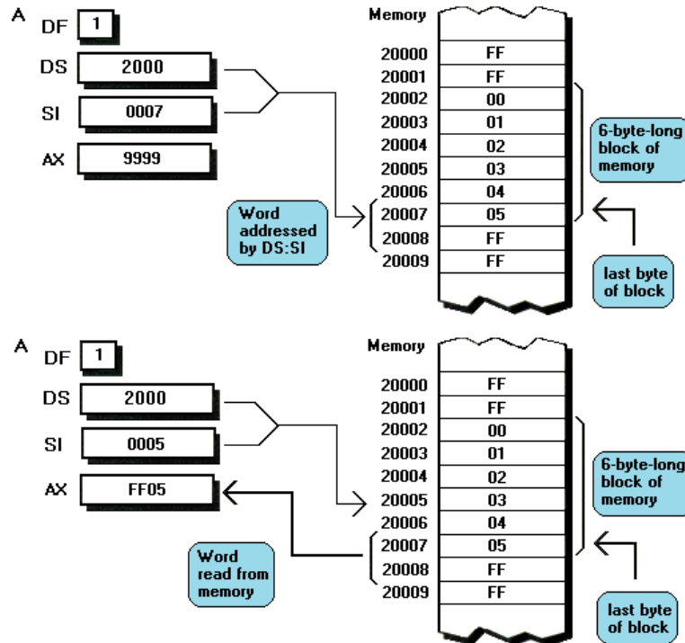
FIGURE 11.5 When a pointer is set to point to the last byte of a memory block and a word-sized access to that address is performed, the last word of the block is not read. Rather, the last byte of the block is read, along with the byte immediately following the block.
