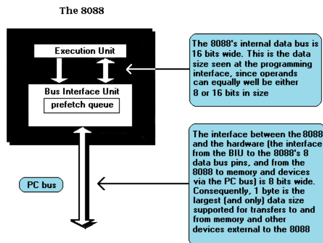
FIGURE 4.2 Internally the 8088 is a 16-bit microprocessor, but externally the 8088 is only an 8-bit microprocessor.
