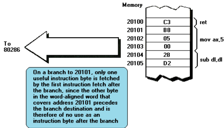
FIGURE 15.3 On the 80286, only one useful instruction byte is obtained by the first instruction fetch after a branch to an odd address. The reason: a single word-sized, word-aligned instruction fetch that includes the byte at the branch target address would also fetch the byte before the branch target address. That preceding byte is useless, as it isn't part of the code that's about to be executed.
