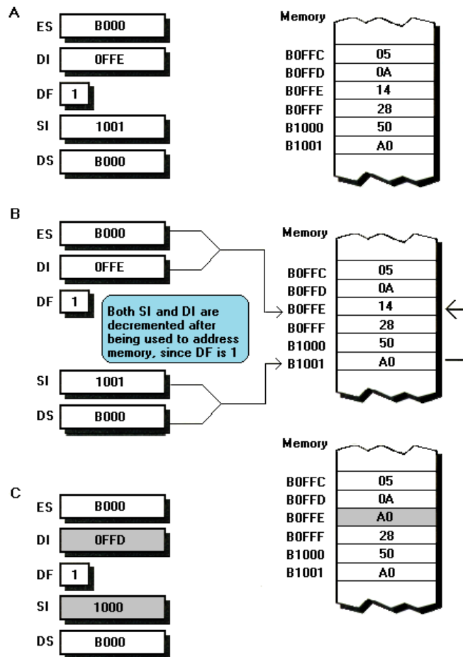
FIGURE 10.3 The operation of movsb with DF set to 1. (A) The state of the PC before movsb is executed. (B) The data and addressing paths as movsb executes. (C) The state of the PC after movsb is finished, with altered registers and memory locations shaded. Note that SI and DI are incremented when DF is 0. The instruction movsw is identical to movsb , except that a word rather than a byte of memory is copied and SI and DI are incremented or decremented by 2 rather than 1.
