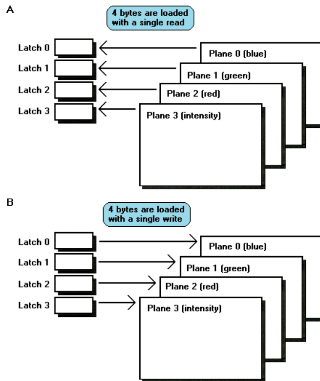
FIGURE 10.15 The internal latches of the EGA and VGA can be used to copy 4 bytes from one display memory location to another with a single byte size read followed by a single byte-sized write, effectively quadrupling the speed at which blocks of display memory copy be copies. (A) A single byte-sized read can load all four latches at once, with each latch receiving 1 byte from the corresponding plane. (B) A single byte sized write can then store the contents of all four latches back to the corresponding planes. Unfortunately, each latch can only store a byte, so word sized string instructions (or, for that matter, word-sized memory accesses of any sort) don't work properly when the latches are used
