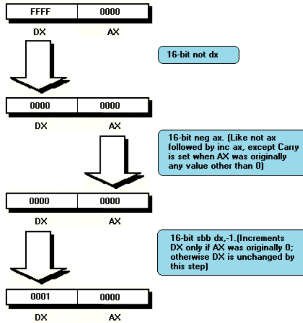
FIGURE 13.2 The 8088 has no 32-bit instructions, so 32-bit negates must be performed as a series of 16-bit operations. This figure illustrates the operation of a 32-bit negate performed with not dx neg ax sbb dx,-1
