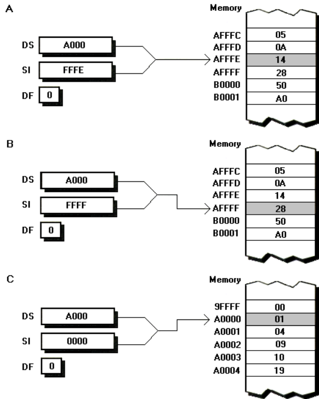
FIGURE 10.12 As a string instruction accesses memory at the end of a segment with a pointer register, it wraps that register to point back to the start of the segment. (A) A lodsb instruction accessing memory 1 byte from the end of the segment pointed to by DS. (In this and all other parts of this figure, the memory location being accessed is shaded.) (B) The next lodsb accessing the last byte in the segment. (C) SI has advanced from 0FFFFh to 0, wrapping back to the start of the segment, with the third lodsb accessing the second byte at offset 0. (D) The fourth lodsb accessing the second byte in the segment, continuing on normally from the start of the segment after the wrap.
