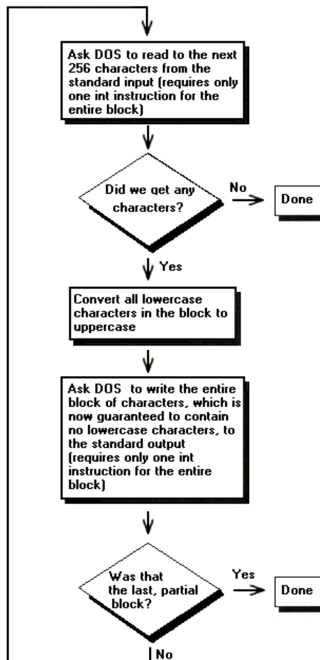
FIGURE 14.5 It's fastest to transfer characters to and from DOS in sizable blocks, avoiding the overhead of invoking DOS functions by performing data buffering within your own code.
