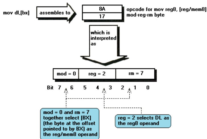
FIGURE 7.8 The interpretation of the bytes assembled for the instruction mov dl,[bx] , illustrating the encoding of mod-reg-rm bytes.
