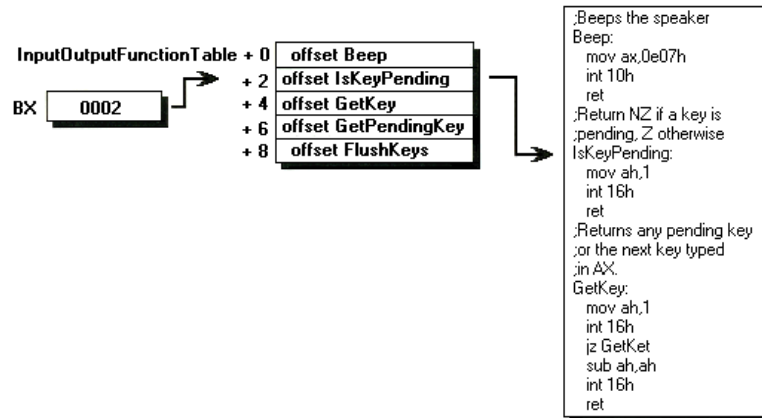
FIGURE 14.8 The operation of a sample jump table. Here the function JumpToInputOutputFunction in the code
