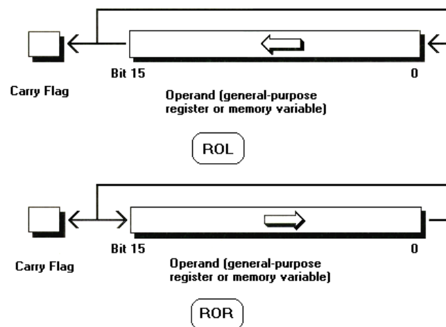
FIGURE 9.2 The instructions rol and ror shift the bits in the operand to the left and right, respectively, wrapping the bit shifted out around to the other end of the operand. The bit shifted out is copied to CF as well. This figure illustrates a 16-bit operation; 8-bit operands can be rotated as well.
