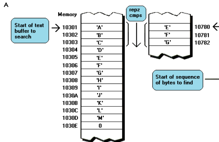
FIGURE 11.14 One way to search for a fixed length sequence of bytes in a text buffer is by starting repz cmps at each byte of the buffer that is at least sequence-length number of bytes away from the end of the buffer. In other words, we could conceivably start the sequence. (A) The check of the first byte of the buffer. (B) The check of the second byte of the buffer. While this approach works, it requires one loop for each potential sequence-starting byte and also incurs the start-up overhead of repz cmps at each character. In this figure, five loops, each starting a new repz cmps , would be required to find the matching sequence starting at 10305.
