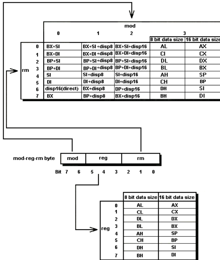
FIGURE 7.6 The interpretation of mod-reg-rm byte. The mod-reg-rm byte specifies two operands. One may reside either in a register or in memory, while the other must reside in a register. The mod and rm fields together specify the register/memory operand, while the reg field specifies the register operand.
