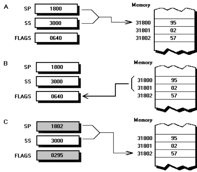
FIGURE 15.4 An example of the operation of popf . (A) The state of the PC before popf is executed. (B) The state of the PC as popf executes. (C) The state of the PC after popf is finished.
