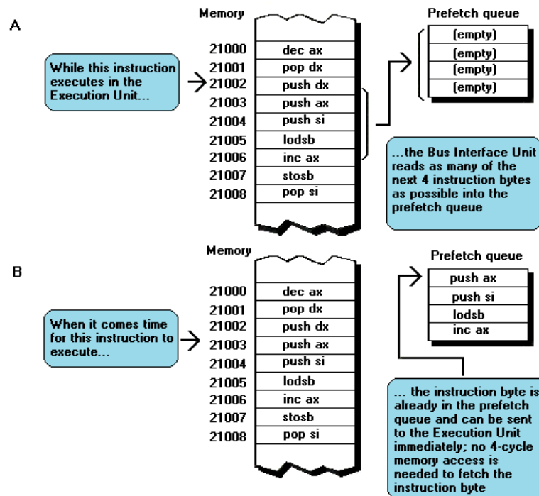
FIGURE 12.4 While the execution unit executes an instruction, the bus interface unit prefetches up to 4 of the instruction bytes immediately following the current instruction in memory. This often allows the BIU to have the next instruction byte immediately available when the EU requests it, thereby avoiding the 4 or more EU idle cycles that result when the BIU has to read memory in order to fill an EU request. (A) The instruction bytes that the 8088 tries to read into the prefetch queue while push dx executes. In reality, the 8088 couldn't fetch 4 bytes during one push dx , but for illustrative purposes we'll assume 4 bytes are prefetched.
