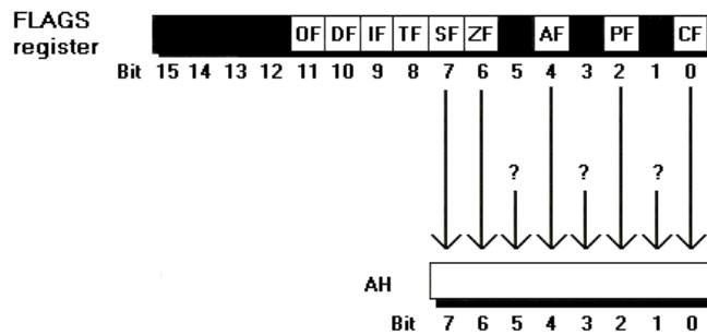
FIGURE 8.12 The lahf instruction copies the lower byte of the 8088's flags register to the AH register. This byte contains the 8088 equivalents of the 8080's flags, located in the same bit positions as in the 8080's flags register. Note that the values of the bits of AH copied from unused bits of the flags register (bits 5, 3, and 1) are unidentified, that is, those bits are not guaranteed to have any particular values.
