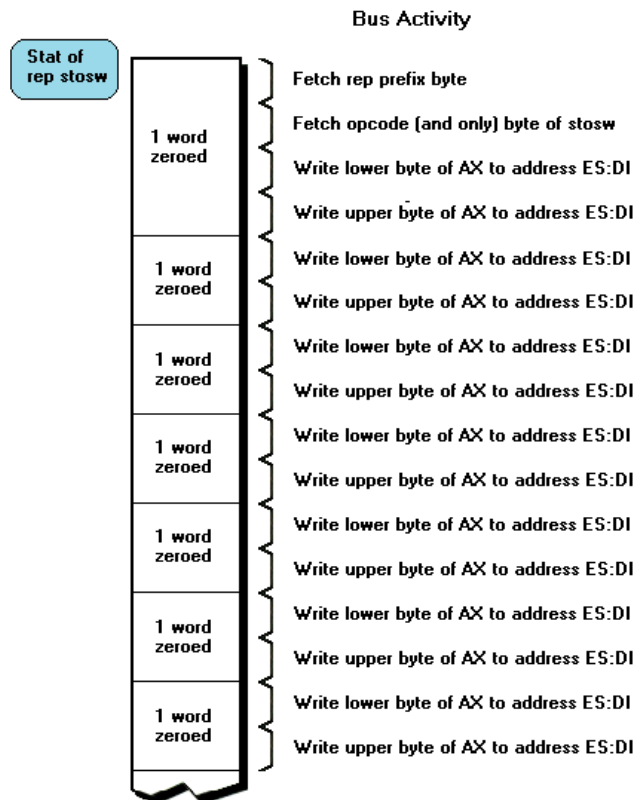
FIGURE 10.8 Bus activity as the rep stosw in Listing 10-8 executes. Instruction fetching is not required for the duration of rep stosw after the 2 bytes of that instruction are fetched, since the 8088 holds repeated string instructions internally and does not require them to be fetched again as they're repeated. (In fact, 4 instruction bytes will be prefetched as stosw repeats, giving the next few instructions a head start when rep stosw finishes.) The lack of instruction fetching means that only 8 cycles (2 bytes times 4 cycles) are required to complete the bus access for each stosw . This allows rep stosw to run at about its official speed of 14 cycles per repetition. Note that this figure is only an illustrative approximation of bus activity and does not necessarily represent the actual sequence of bus accesses as the code in Listing 10-8 executes.
