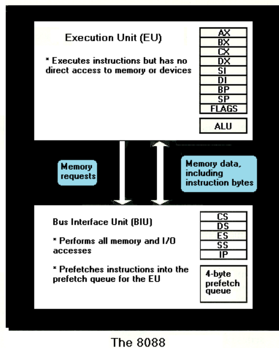
FIGURE 3.3 Internally, the 8088 consists of two separate processing sections operating in parallel. The execution unit (EU) contains the general purpose registers, the flags, and the ALU, and executes instructions, while the bus interface unit (BIU) contains the instruction pointer and the segment registers, and performs all memory accesses for the EU. The BIU not only performs all reads and writes of memory operands, but also prefetches the next few instruction bytes from memory during idle times, storing the bytes in a 4-byte internal instruction prefetch queue until the EU requests them. If a branch is performed, all instruction bytes in the prefetch queue are discarded.
