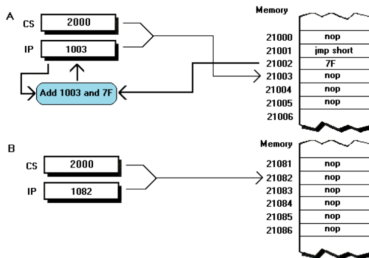
FIGURE 12.3 Relative branches within the range of -128 to +127 bytes of the current instruction pointer string can be specified with one byte rather than 1 word, saving code space.
