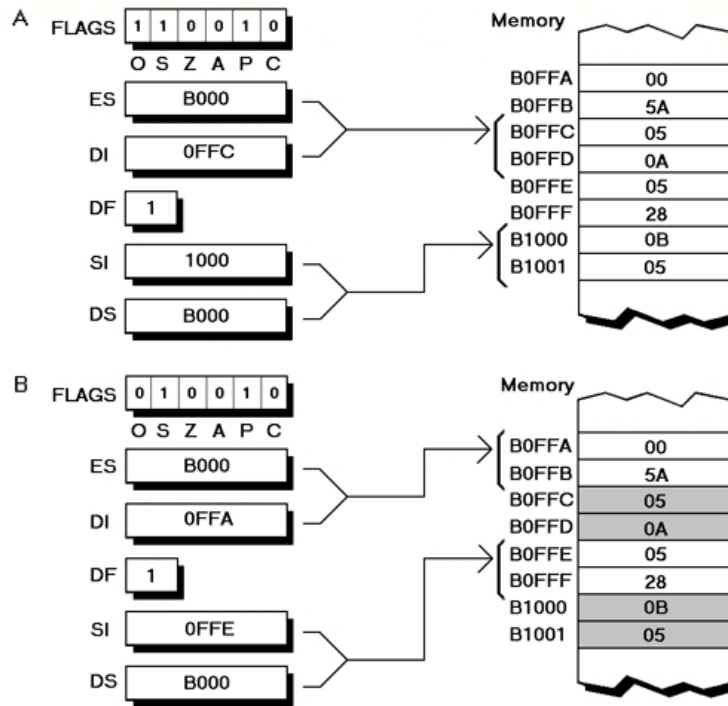
FIGURE 10.10 Another example of a string instruction advancing its pointers past the last location accessed. (A) The state of the PC before cmpsw executes. (B) The state of the PC after cmpsw executes. The words that are compared are shaded. You can see that cmpsw advances both SI and DI 1 word past the locations compared. Because DF is 1, SI and DI point to the start of the word preceding the words that were compared. When DF is 0, the pointers used by word-sized string instructions advance to the addresses immediately following (1 byte after) the words accessed. If DF had been 0 in this figure, DS:SI would have advanced to B0000:1002 and ES:DI would have advanced to B000:0FFE, as those are the locations immediately above the words accessed. However, when DF is 1, as in this figure, the pointers advance to the addresses 2 bytes before the words accessed. This is an inevitable result of the memory storage scheme of the 8088, whereby words are stored with the low byte at address n and the high byte at address n+1 , with pointers aimed at the low byte location but rather to the adjacent memory address.
