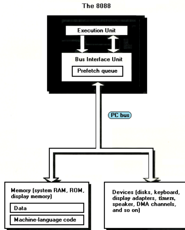
FIGURE 3.4 This view of the PC's resources reflects the true nature of code as data stored in system memory. Code is stored in memory, so it must be fetched by the bus interface unit (BIU) just as data must; consequently, any cycle eaters present between system memory and the BIU affect the 8088's code fetching speed as well as its data fetching speed. In addition, all memory access must pass through the BIU a byte at a time at a rate no faster than 1.2 bytes/microsecond (1 byte per 4 cycles), and serious bottlenecks can develop since code and data fetching can demand data transfer rates as high as 1 byte/209 nsec (1 byte per cycle).
