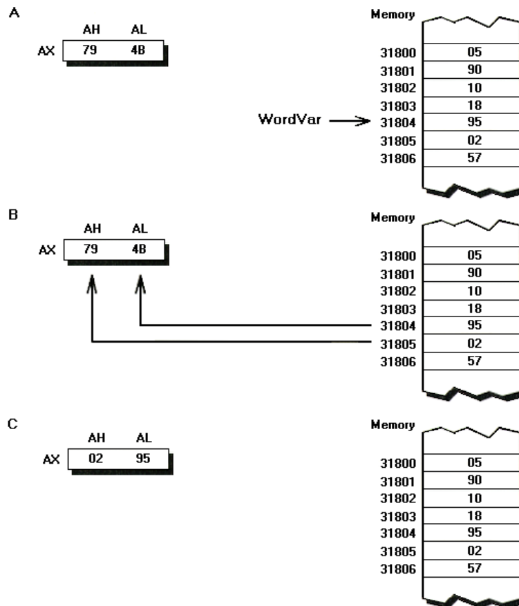
FIGURE 7.4 The 8088 always considers the least significant byte of word sized memory access to be at the lower memory address. (A) The state of the PC as mov ax,WordVar begins. (B) Memory being accessed, with the least significant byte at the lower memory address. (C) Data from the least significant byte is indeed loaded into AL, and data from the most significant byte is loaded into AH.
