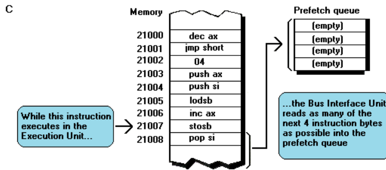
FIGURE 12.5 must be used to fetch the branched-to instruction, stosb , as it is not in the prefetch queue. (Actually, branched-to instructions must always be fetched, even when they're already in the prefetch queue, because branches always empty the prefetch queue.)
