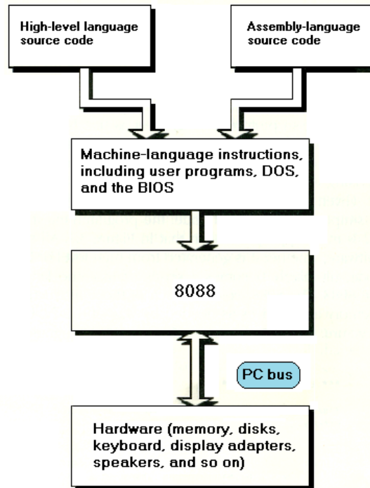
FIGURE 3.2 For high performance assembler programming, this view of the PC's resources is more useful than that of layered system software. Here the emphasis is on the interaction between machine language instructions, the 8088, and the hardware, with cycle eaters potentially present in the PC's hardware and bus.
