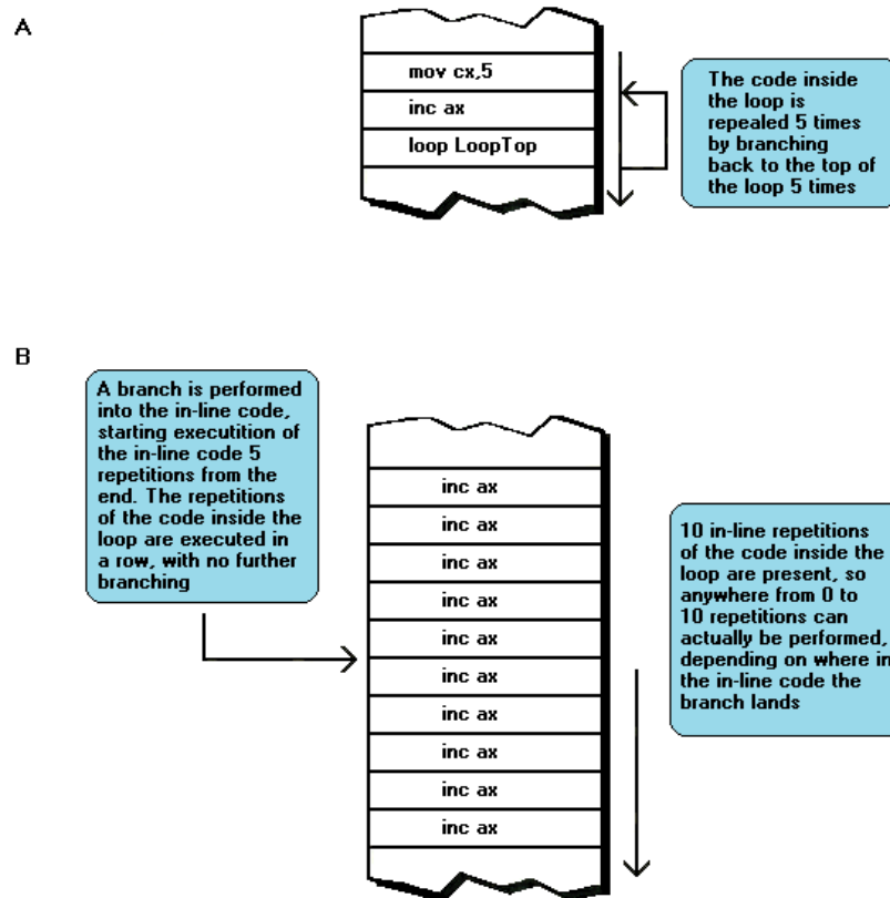
FIGURE 13.11 Branched in-line code is exactly like pure in-line code, except that the in-line code is not necessarily executed starting at the first in-line instruction. Instead, the in-line code is branched into at whatever location produces the desired number of repetitions. As a result, branched-to in-line code can handle variable repetition counts, unlike pure in-line code. (A) A loop that repeats five times. (B) A branched-to in-line version of that loop that repeats five times and is capable of handling up to 10 repetitions.
