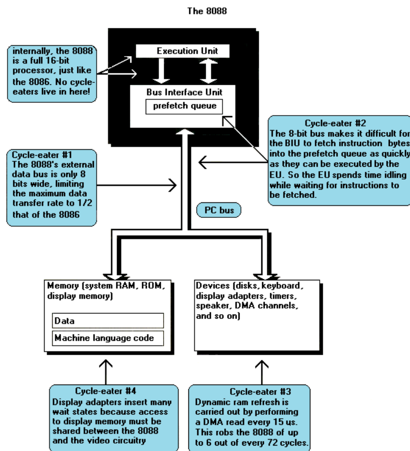
FIGURE 4.1 The locations of the major cycle eaters in the IBM PC. Note that all the cycle eaters are external to the execution unit of the 8088.
