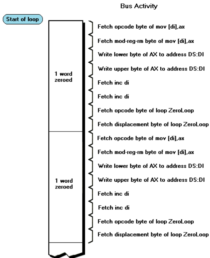
FIGURE 10.7 Bus activity as the loop in Listing 10-7 executes. Instruction prefetching dominates because the 6 bytes in the loop must be fetched once for each word written to memory. Given the eight memory accesses required each time through the loop, there is no way a pass through the loop can take less than 32 cycles (8 bytes at 4 cycles per byte). Note that this figure is only an illustrative approximation of bus activity and does not necessarily represent the actual sequence of bus accesses as the code in Listing 10-7 executes.
