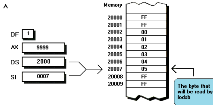
FIGURE 11.8 When DF is 1, adjustments must be made when switching between byte and word-sized string instructions. Since the address of the next byte is not the same as the address of the next word, incorrect data will be read if adjustments are not made, as illustrated by Figure 11.7. This figure shows that the last 3 bytes of a memory block are read correctly with the following code:
