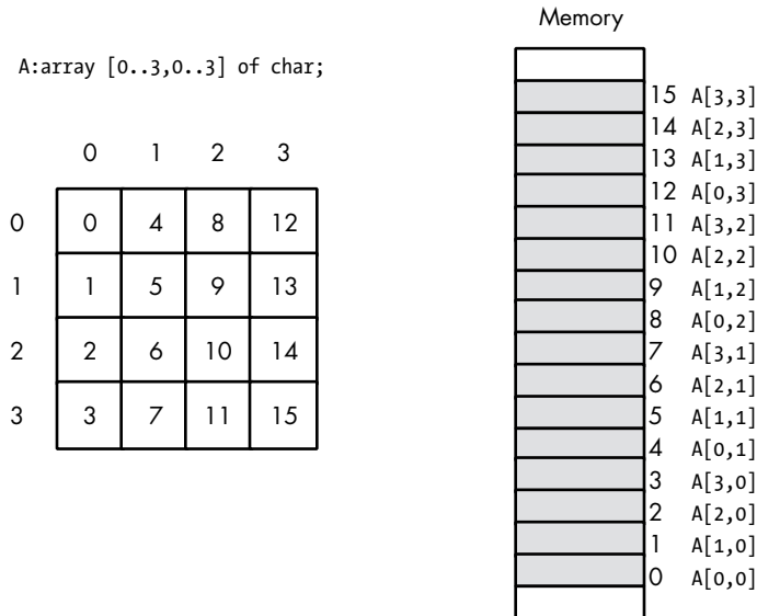
Figure 8-6: Column-major ordering
