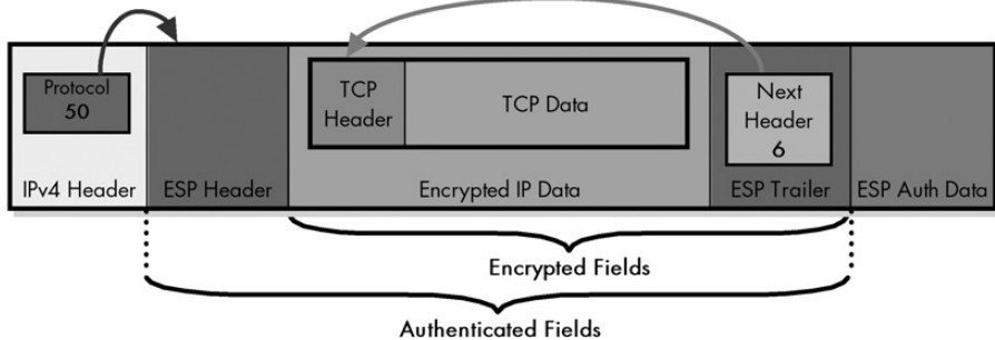
IPv4 ESP Datagram Format - IPsec Transport Mode
