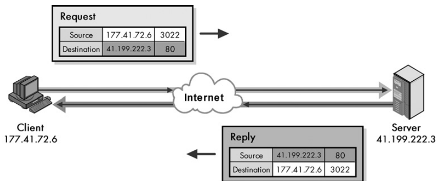
Figure 43-3: TCP/IP client/server application port mechanics This highly simplified example shows how clients and servers use port numbers for a request.reply exchange. The client is making an HTTP request and sends it to the server at HTTP’s well-known port number, 80. Its port number for this exchange is the pseudo-randomly selected port 3022. The server sends its reply back to that port number, which it reads from the request.
