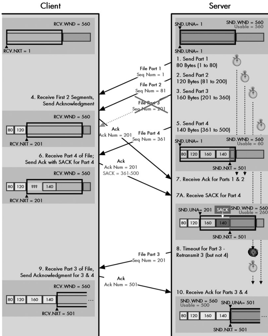
Figure 49-3: TCP retransmission with selective acknowledgment (SACK) This is the example from Figures 49-1 and 49-2, changed to use the optional selective acknowledge feature. After receiving Parts 1, 2, and 4 of the file, the client sends an acknowledgment for 1 and 2 that includes a SACK for Part 4. This tells the server not to resend Part 4 when Part 3's timer expires.
