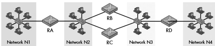
Figure 38-1: Sample RIP AS This is an example of a simple AS that contains four physical networks and four routers.
