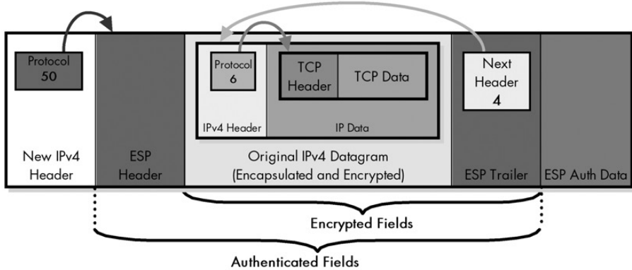
IPv4 ESP Datagram Format - IPsec Tunnel Mode
