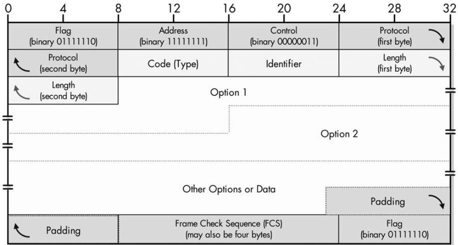
Figure 12-4: PPP control message carrying options
