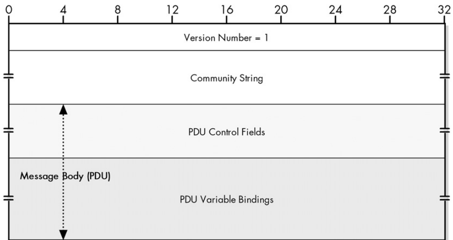
Figure 68-6: SNMPv2c general message format
