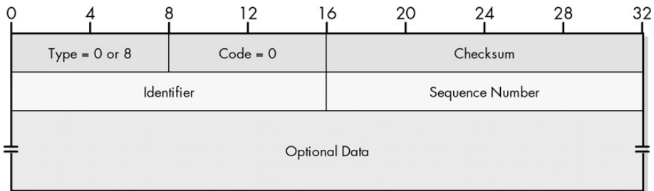
Figure 33-1: ICMPv4 Echo and Echo Reply message format Two special fields are used within the format of these messages. They allow devices to match Echo and Echo Reply messages together, and exchange a sequence of messages. The Identifier field was envisioned as being used as a higher-level label, like a session identifier, while the Sequence Number was seen as something to identify individual test messages within a series. However, the use of these fields is up to the particular implementation. In some cases, the Identifier field is filled in with the process number of the application that is using the Echo or Echo Reply message to allow several users to use utilities like ping without interference.
