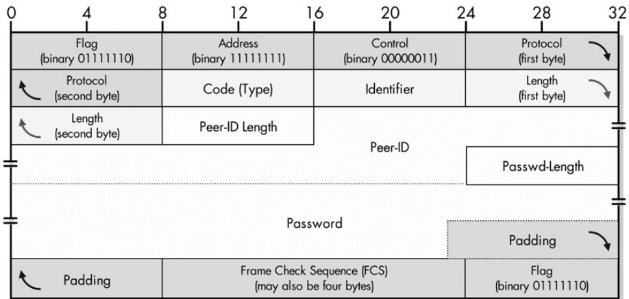
Figure 12-6: PPP PAP Authenticate-Request frame format
