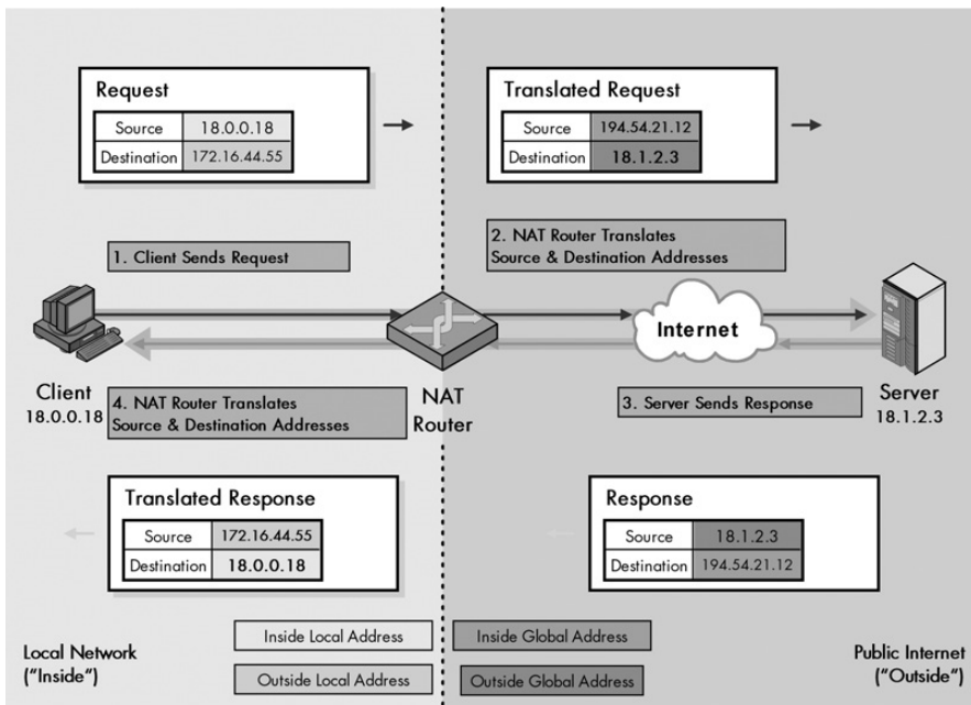
Figure 28-5: Operation of Overlapping NAT/twice NAT This figure is very similar to Figure 28-2, except that as you can see, the NAT router translates both source and destination addresses each time (shown in bold). Table 28-4 contains a complete explanation of the four steps in overlapping NAT. Refer to Figure 28-1 for an explanation of address types.
