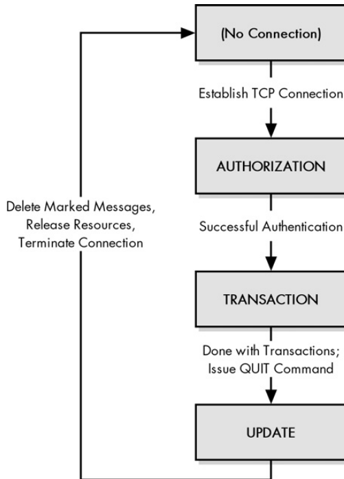
Figure 78-1: POP3 finite state machine POP uses a finite state machine (FSM) to describe its operation, but it is very simple because it is linear. Once a TCP connection is established between a POP3 client and POP3 server, the session proceeds through three states in sequence, after which the connection is terminated.
