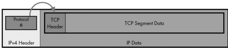
Original IPv4 Datagram Format
