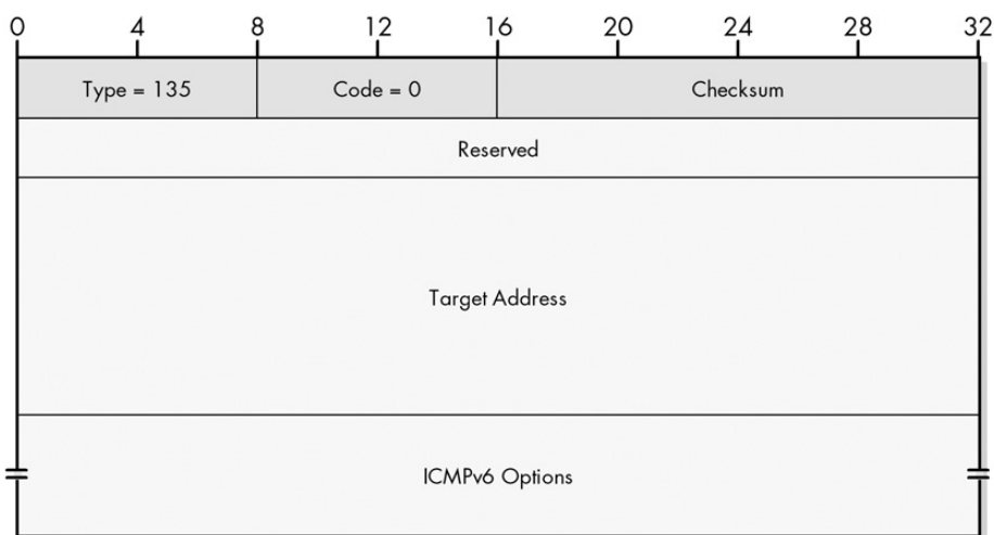
Figure 35-5: ICMPv6 Neighbor Solicitation message format
