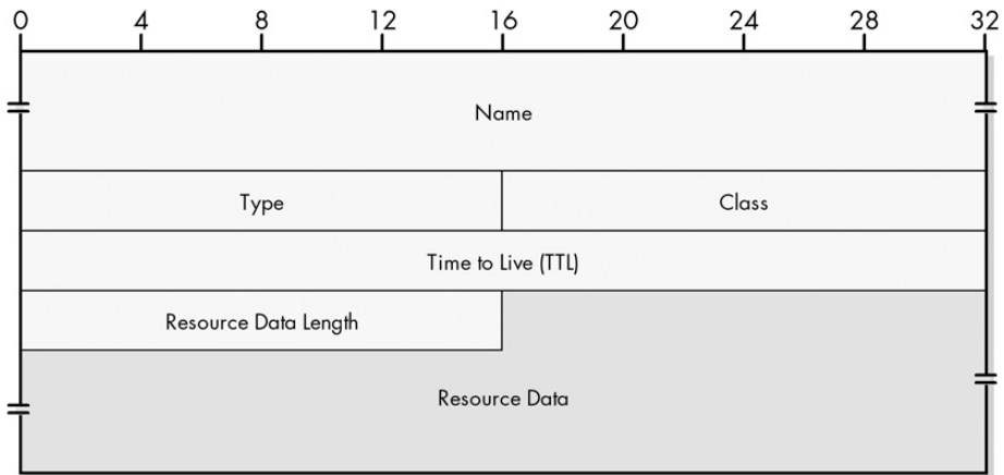
Figure 57-4: DNS common RR format
