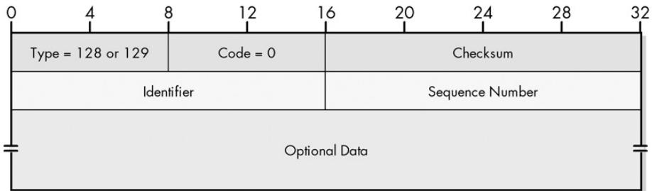
Figure 35-1: ICMPv6 Echo Request and Echo Reply message format
