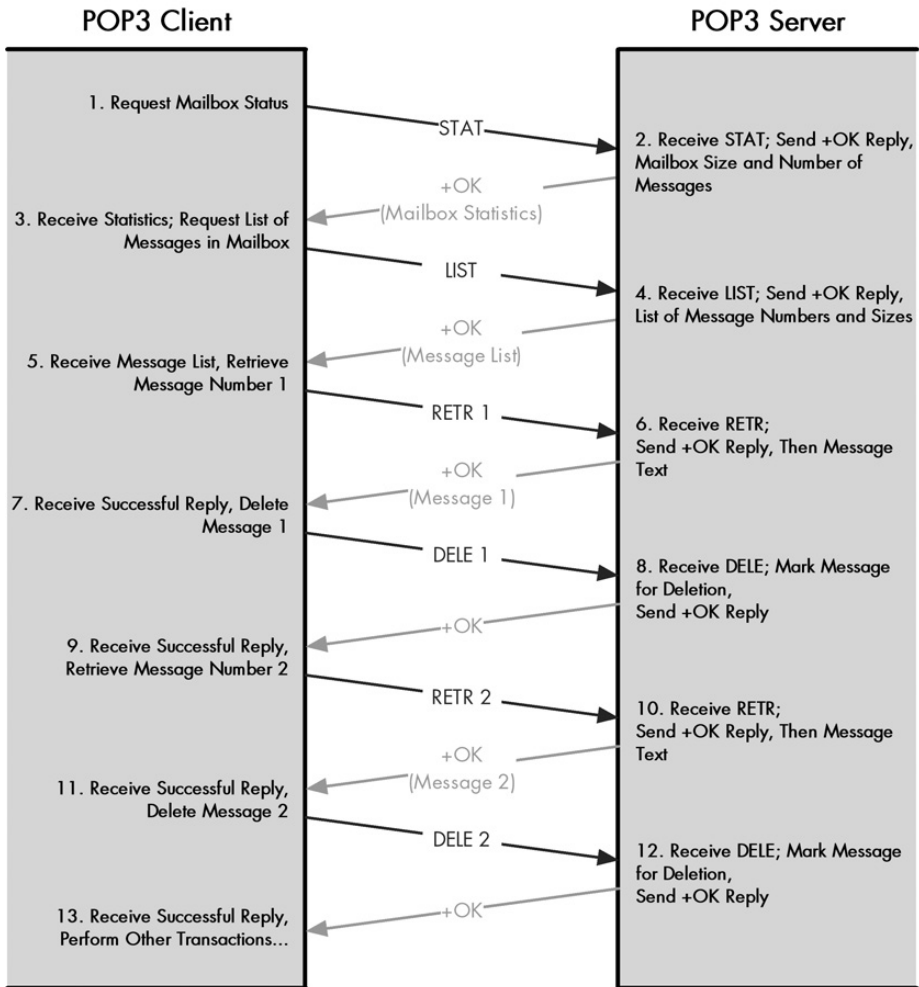
Figure 78-3: POP3 mail exchange process This diagram shows the typical exchange of commands and replies employed by a POP3 client to retrieve email from a POP3 server. The STAT command is used to get mailbox statistics, followed by the LIST command to obtain a list of message numbers. Each message in turn is then retrieved using RETR and marked for deletion by DELE . (Messages are not actually deleted until the Update state is entered.)
