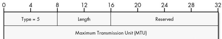
Figure 35-12: ICMPv6 MTU option format
