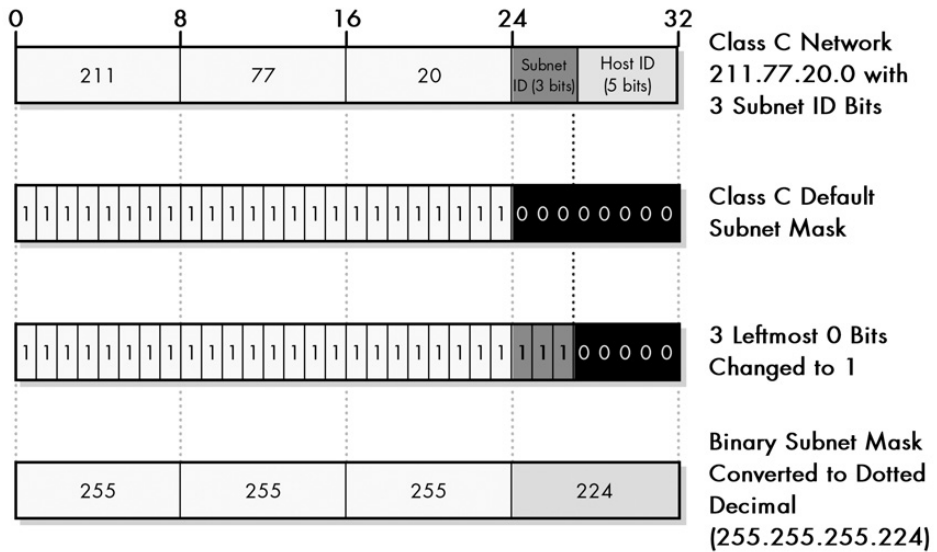
Figure 19-4: Determining the custom subnet mask for a Class C network
