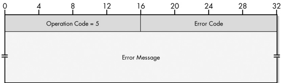
Figure 73-7: TFTP error message format
