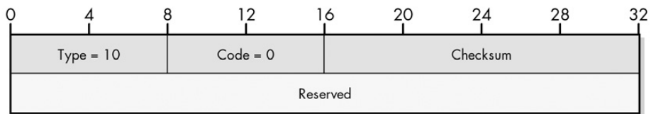
Figure 33-4: ICMPv4 Router Solicitation Message format
