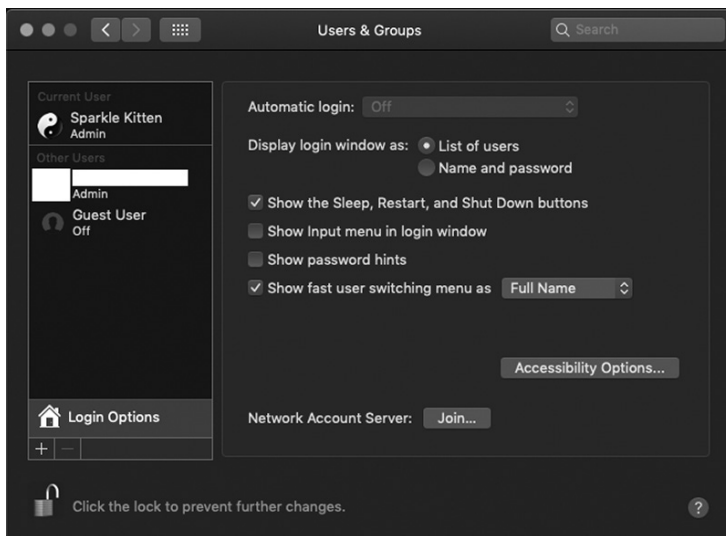
Figure 5-17: Login options
