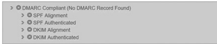
Figure 3-8: DMARC failure
