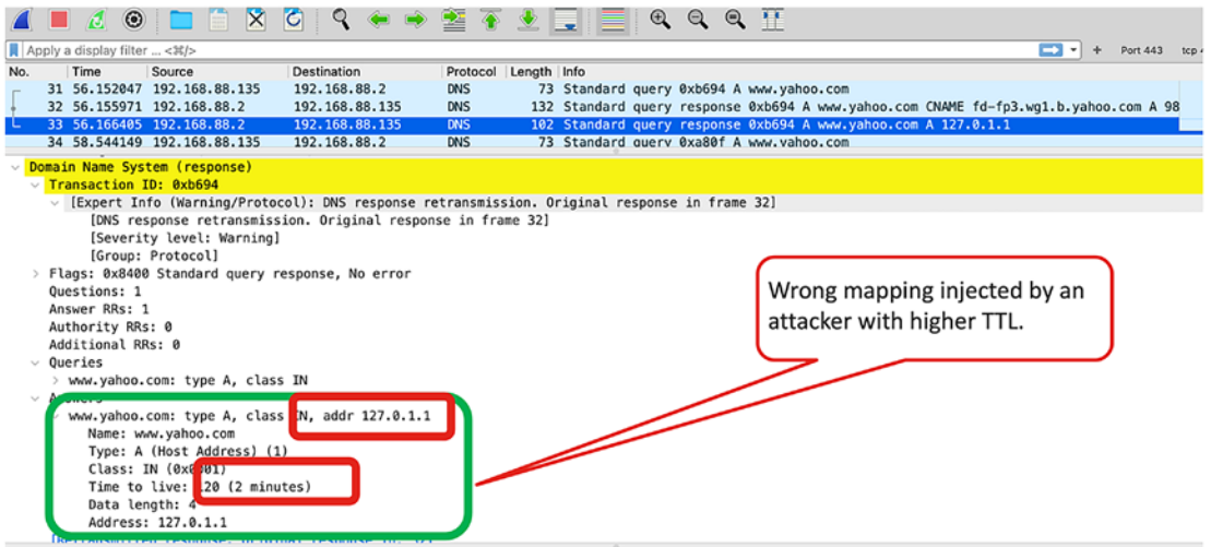
Figure 8-4. DNS spoofing
