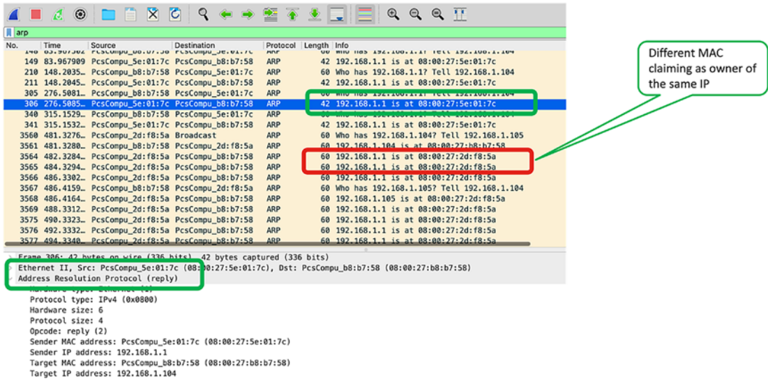
Figure 8-1. ARP spoofing
