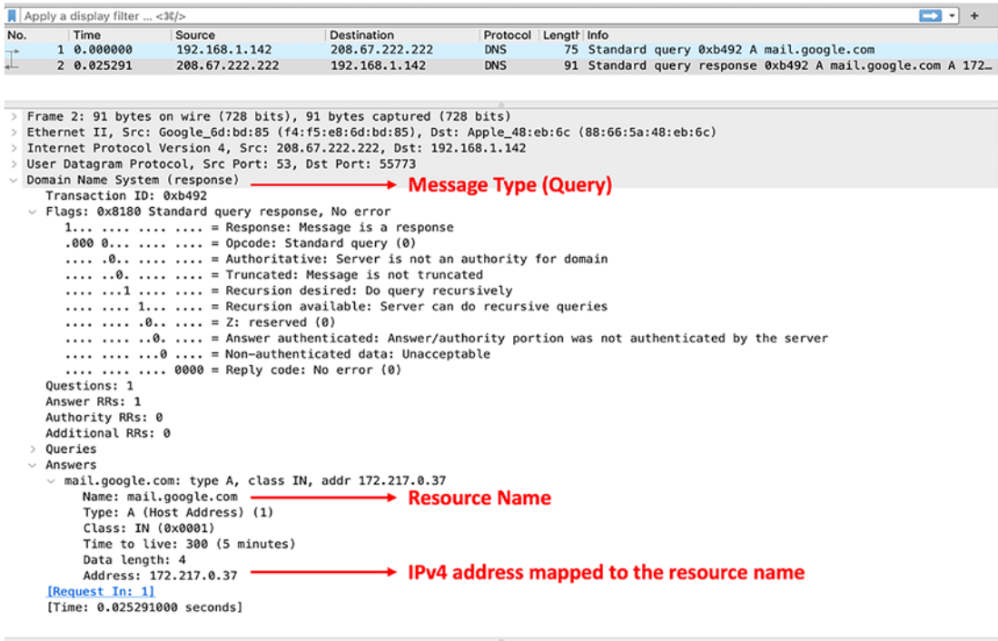
Figure 3-29. DNS response
