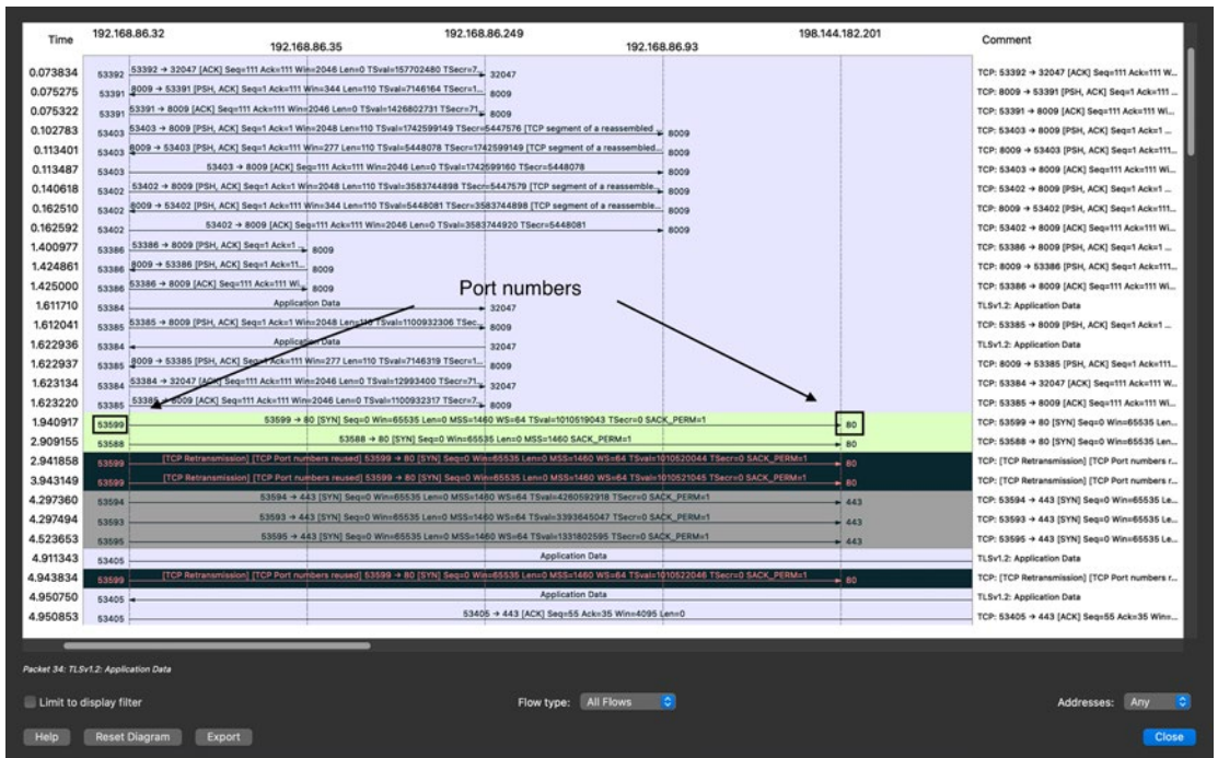
Figure 1-17. Flow graph
