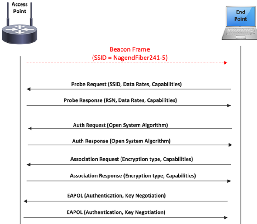
Figure 4-16. Registration process
