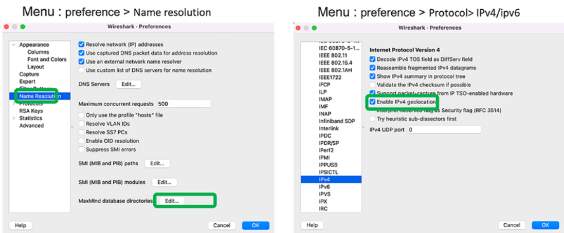
Figure 8-13. Enabling geolocation
