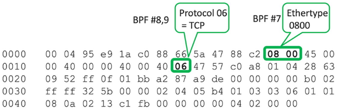
Figure 2-16. BPF example
