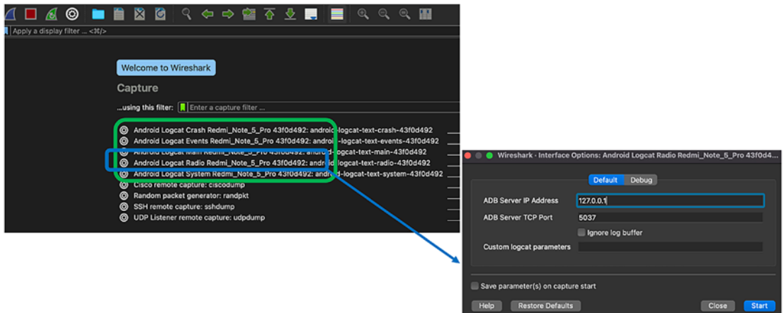
Figure 2-9. Androididump interfaces
