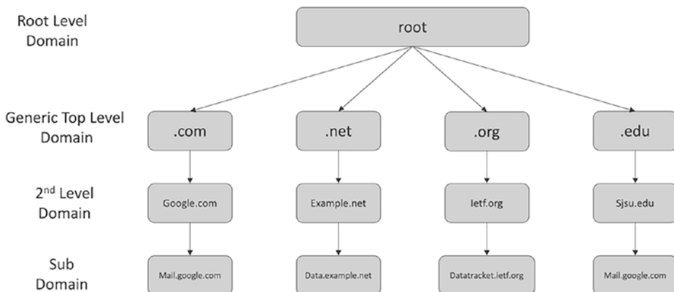
Figure 3-28. DNS hierarchy
