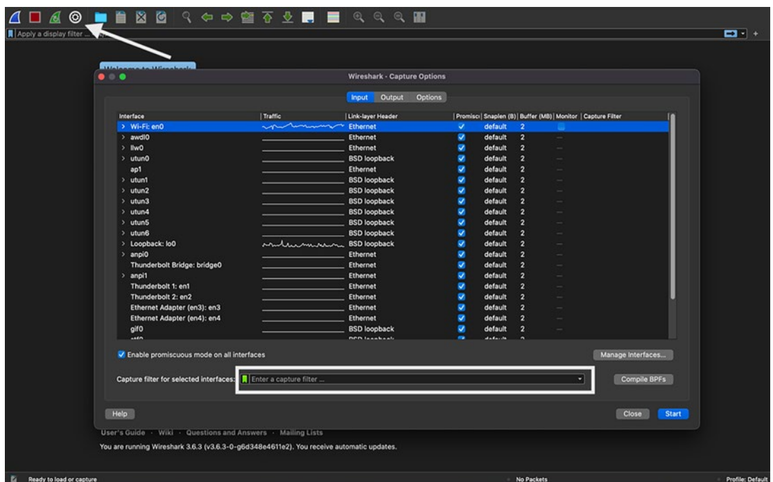
Figure 1-5. Capture filter
