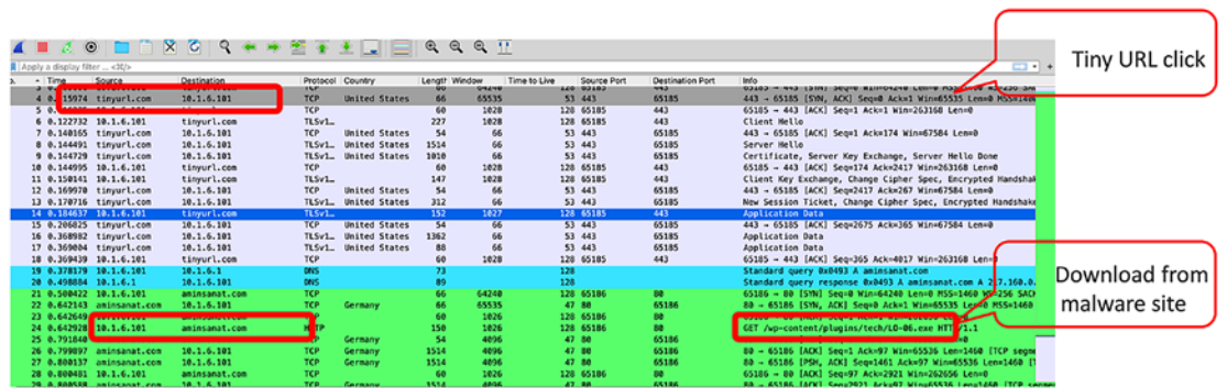
Figure 8-19. Malware download
