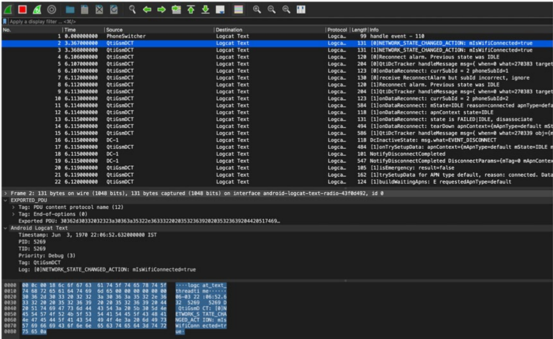
Figure 2-10. Androiddump capture
