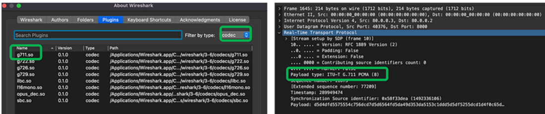
Figure 5-20. Codec types
