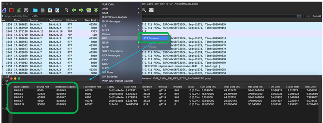
Figure 5-18. RTP streams
