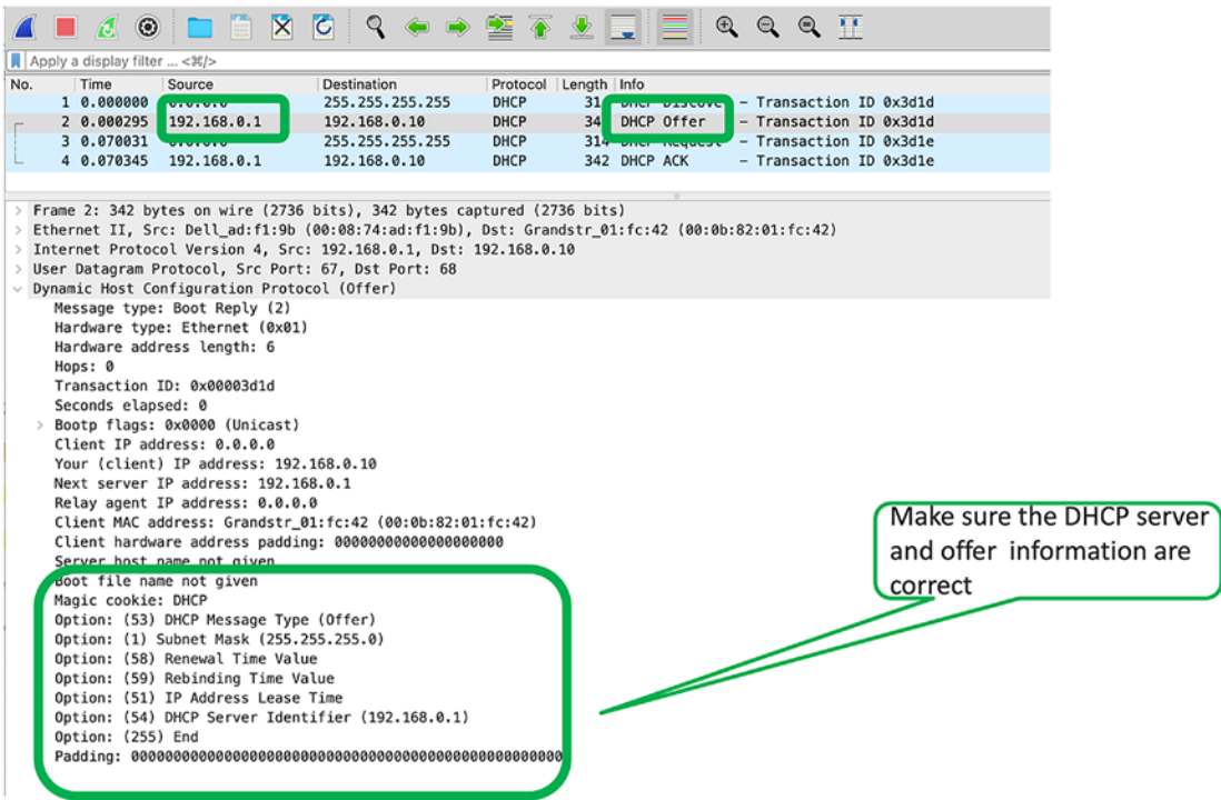
Figure 8-3. DHCP verification
