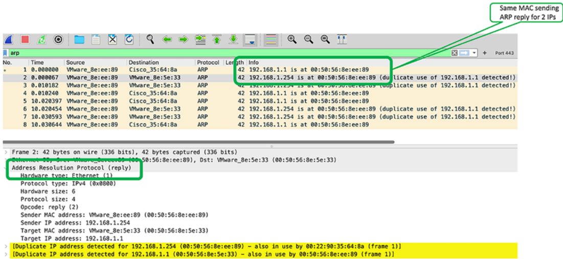
Figure 8-2. ARP poisoning
