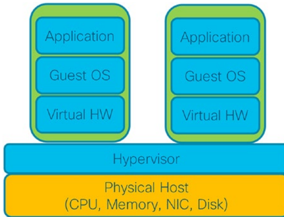
Figure 6-4. Virtual machines
