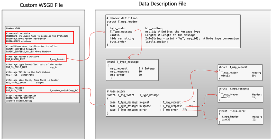
Figure 9-9.
