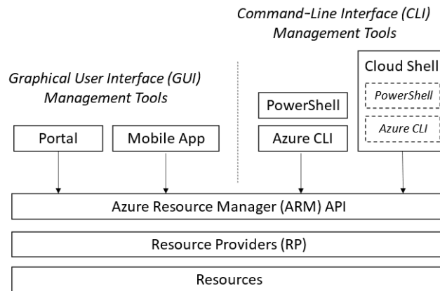
Figure 6.14 – Azure management tools
