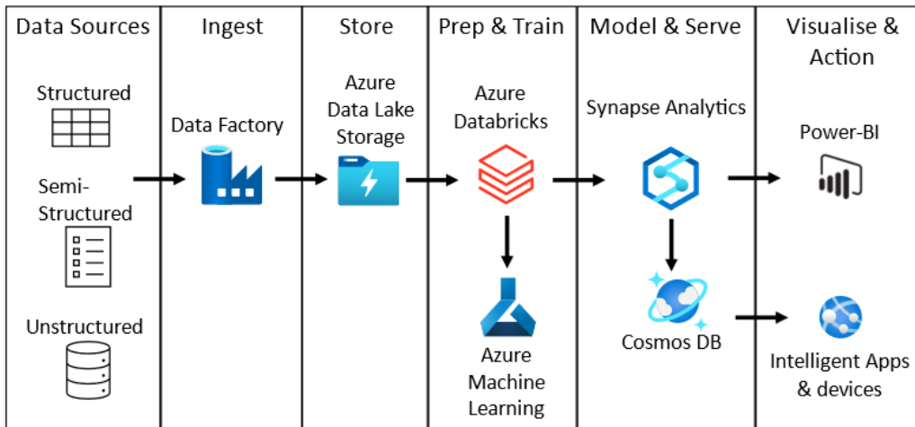
Figure 5.17 – Azure Databricks solution architecture
