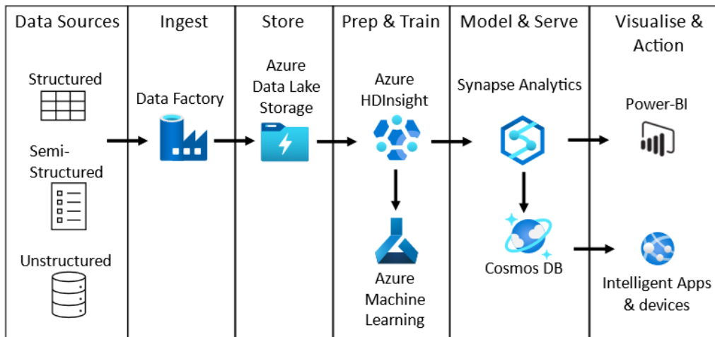
Figure 5.16 – Azure HDInsight solution architecture
