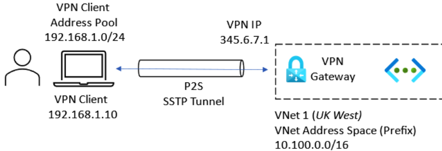
Figure 4.19 – Point-to-Site VPN
