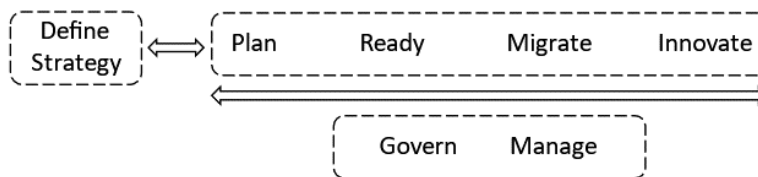
Figure 9.6 – Azure CAF methodologies
