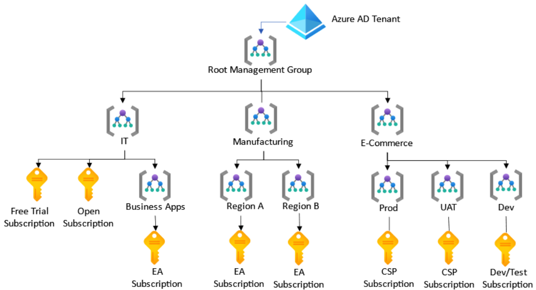
Figure 3.18 – Azure management group and subscription relationships
