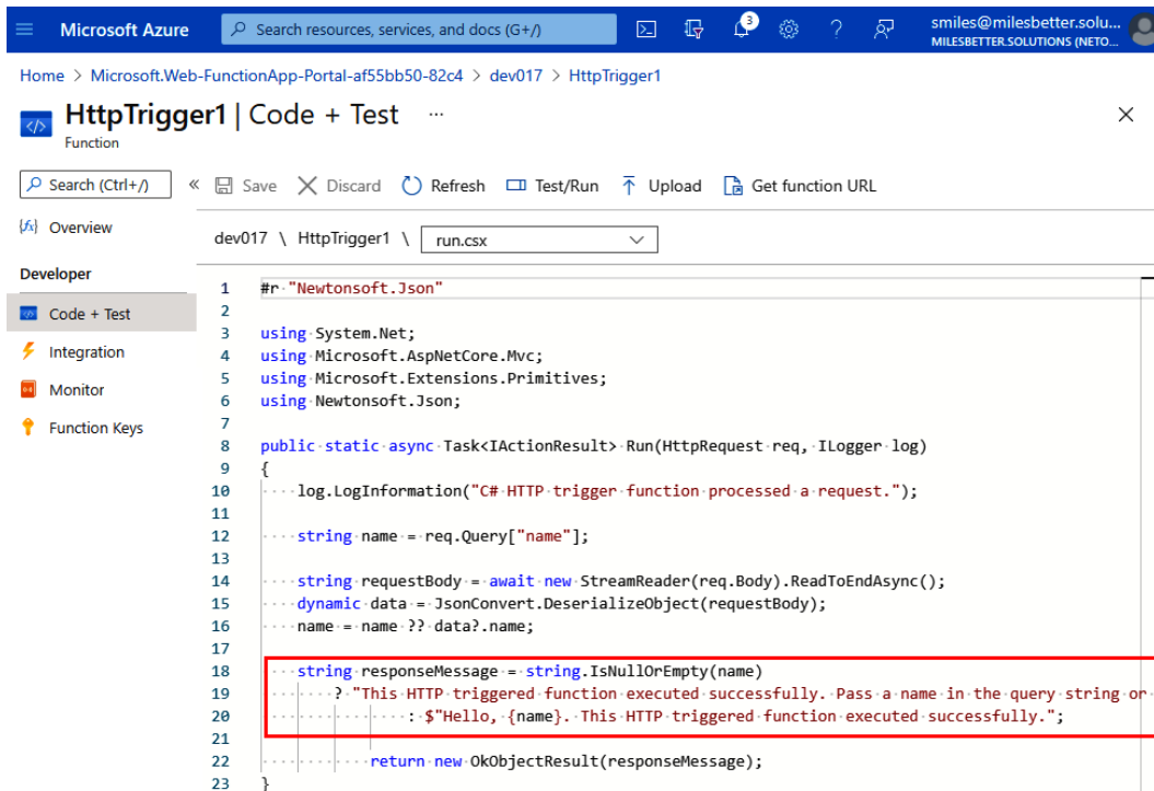
Figure 5.27 – Function app code
