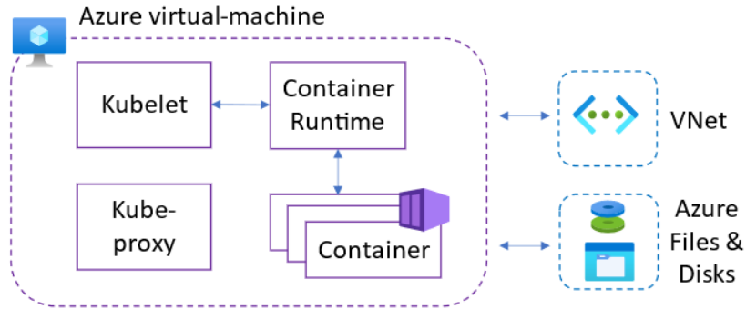
Figure 4.8 – Worker node high-level service architecture
