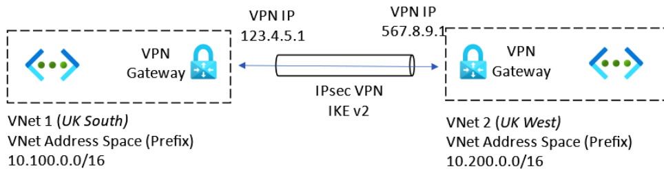
Figure 4.21 – VNet-to-VNet VPN
