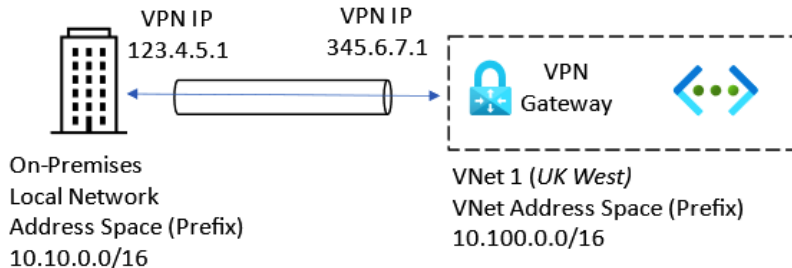
Figure 4.20 – Site-to-Site VPN
