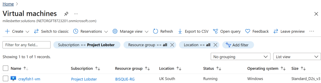
Figure 4.26 – Virtual machines
