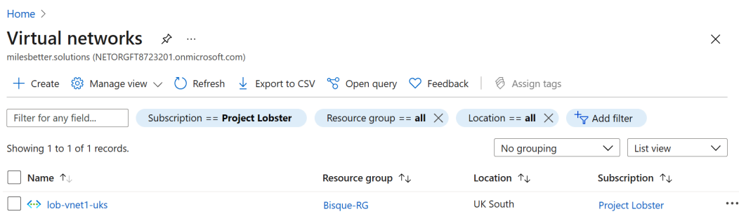
Figure 4.24 – Virtual networks
