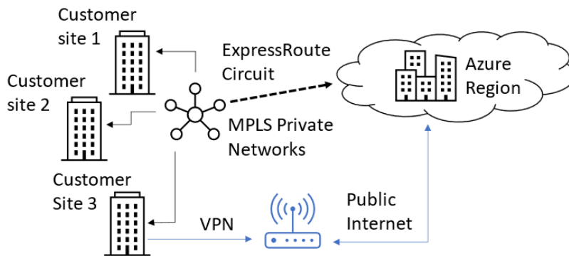
Figure 4.22 – ExpressRoute
