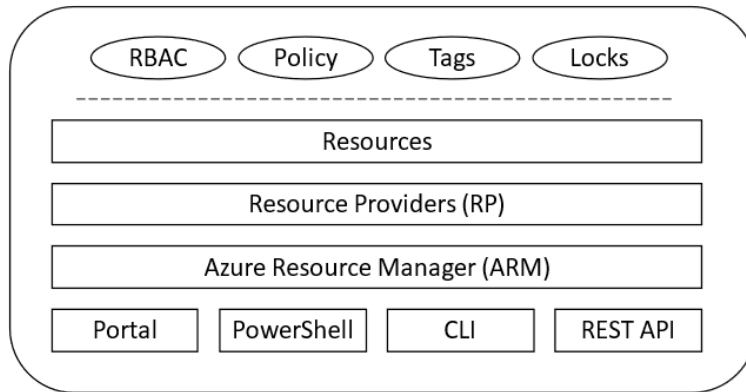
Figure 3.23 – ARM architecture
