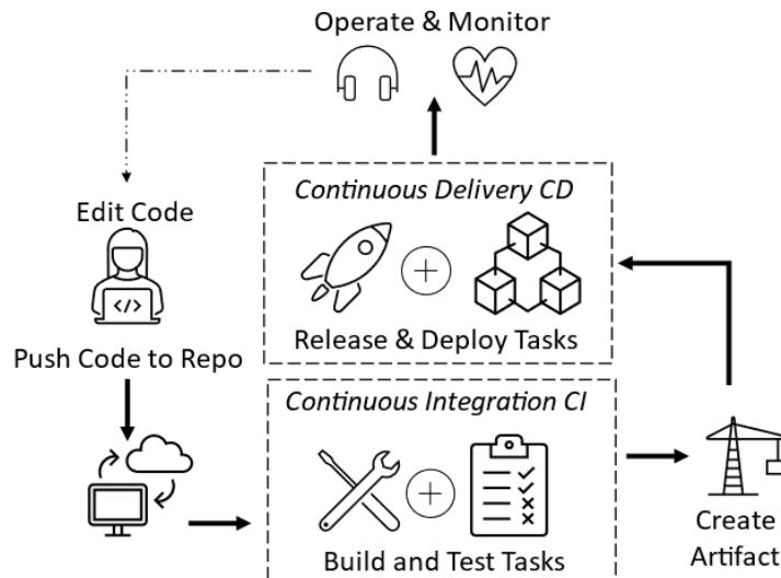
Figure 5.22 – Continuous integration/continuous delivery
