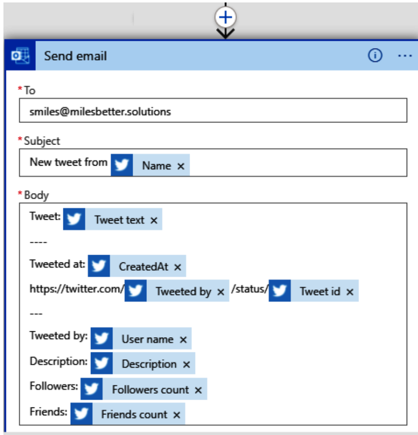
Figure 5.33 – Logic app workflow
