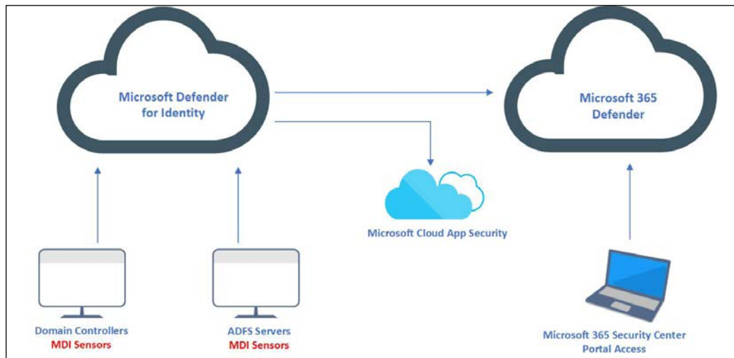
Figure 19.19: MDI architecture
