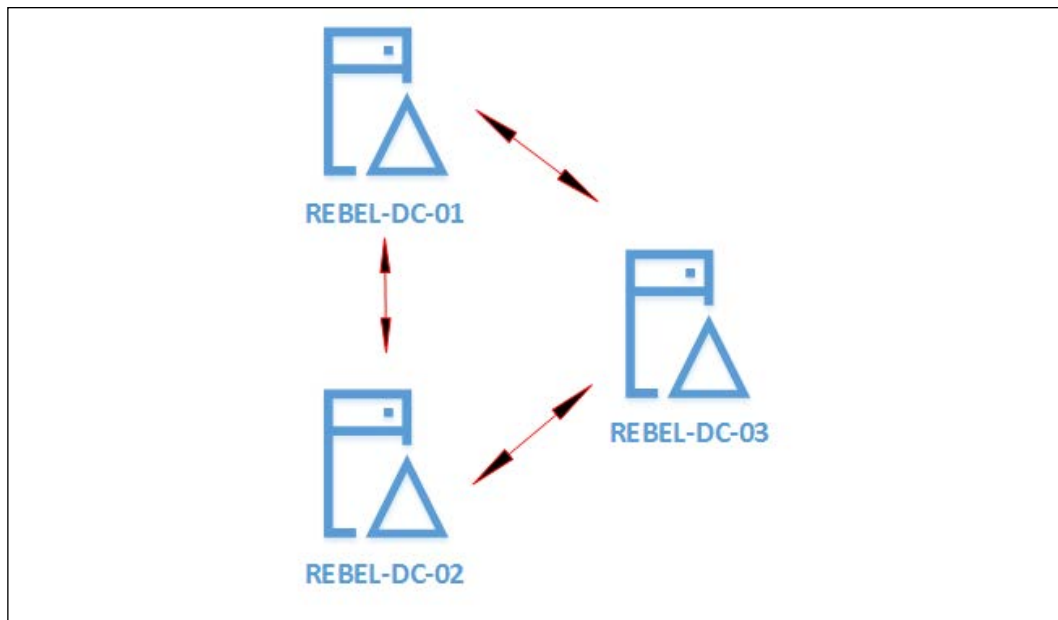
Figure 11.14: Intra-site replication
