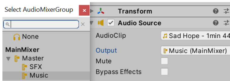
Figure 10.15 – Making an AudioSource belong to an Audio Mixer group
