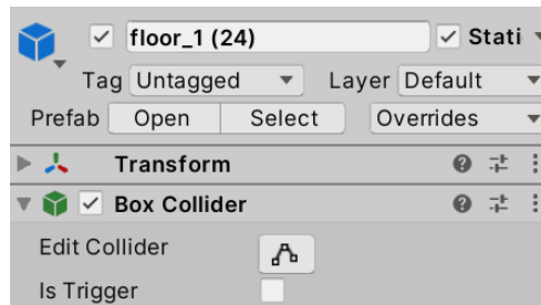
Figure 15.5 – Configuration for floor tiles; remember the static checkbox is for lighting only
