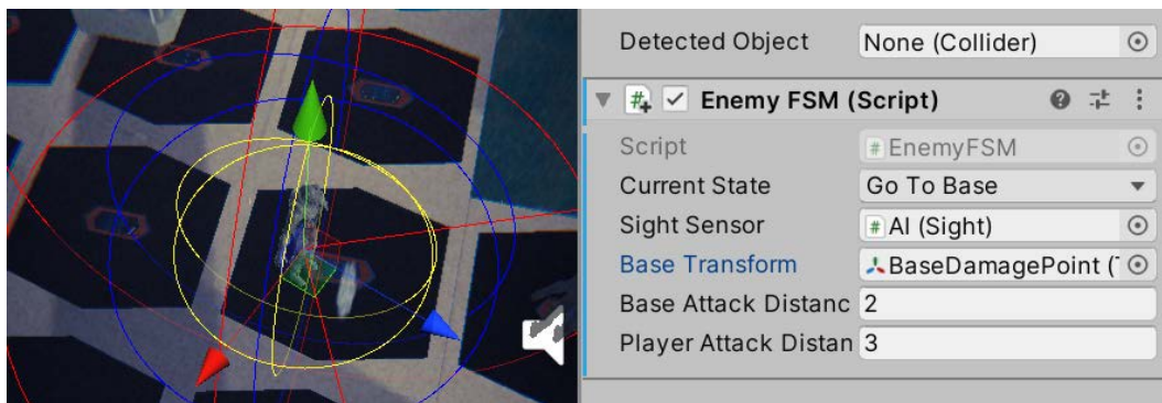
Figure 18.28 – Enemy FSM settings
