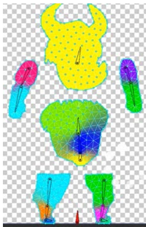
Figure 12.2 – Mesh skinning weights visually represented as colors
