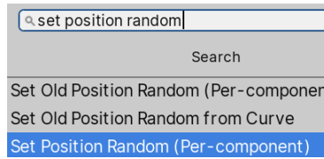
Figure 7.47 – Adding blocks
