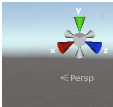
Figure 3.8 – Axis Gizmo
