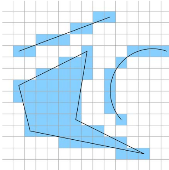
Figure 6.2 – Example of figures being rasterized
