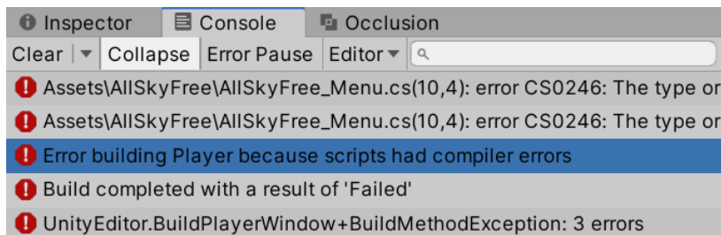
Figure 20.5 – Build errors
