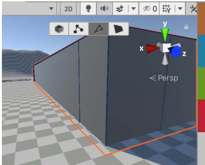
Figure 4.43 – Overlapping faces
