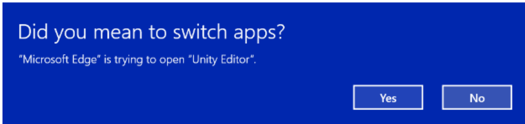
Figure 5.10 – Switching apps
