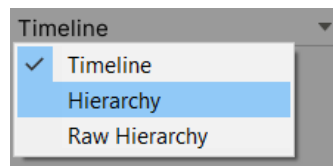
Figure 19.18 – Selecting Hierarchy
