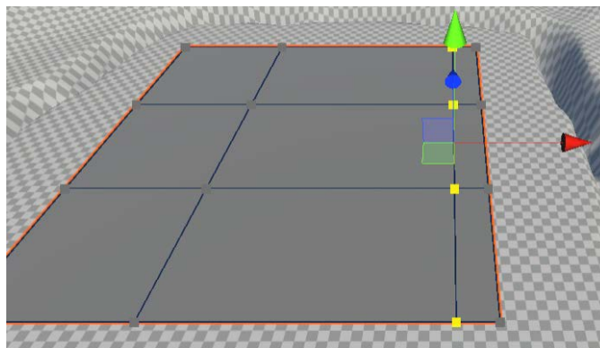
Figure 4.32 – Moved vertexes
