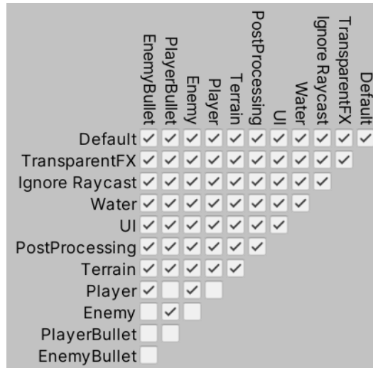
Figure 15.12 – Making Player bullets to collide with enemies and Enemy bullets with the Player
