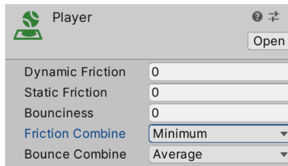
Figure 15.25 – Creating a Physics Material
