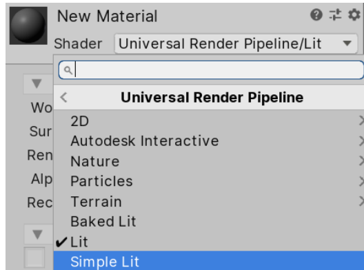
Figure 6.10 – Simple Lit Shader selection
