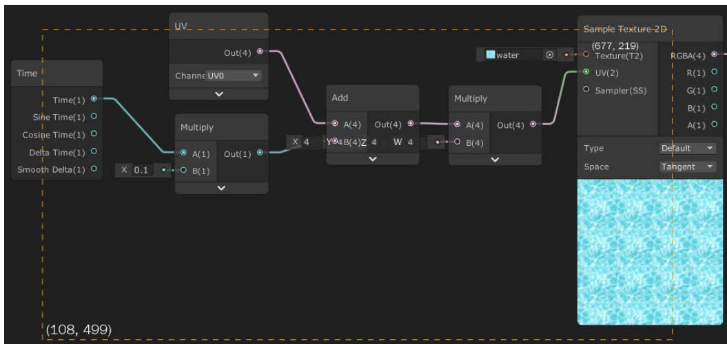
Figure 6.42 Selecting several nodes
