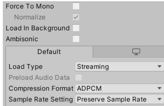
Figure 10.5 – Music and ambient settings
