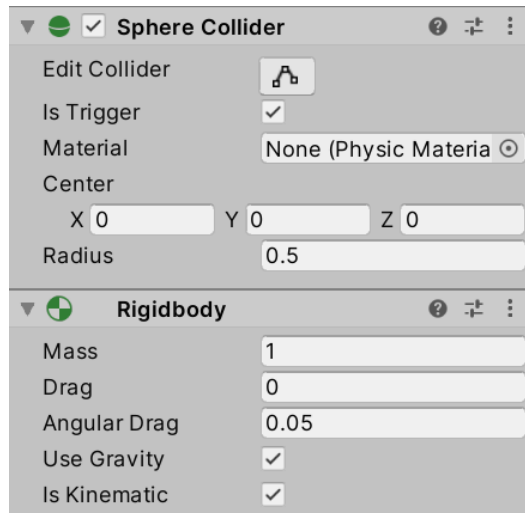
Figure 15.8 – The Kinematic Trigger setting for our bullet; Is Trigger and Is Kinematic are checked
