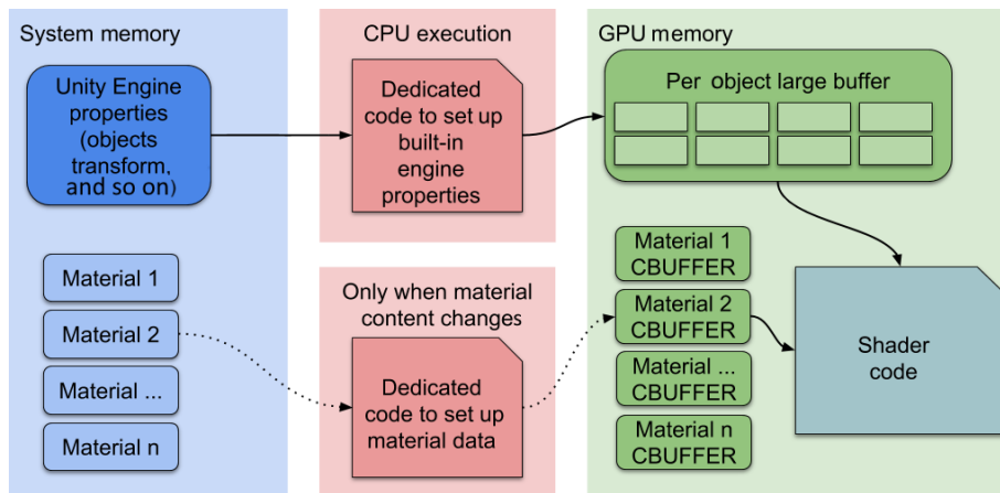
Figure 19.10 – GPU data persistence for materials, which allows SRP Batcher to exist
