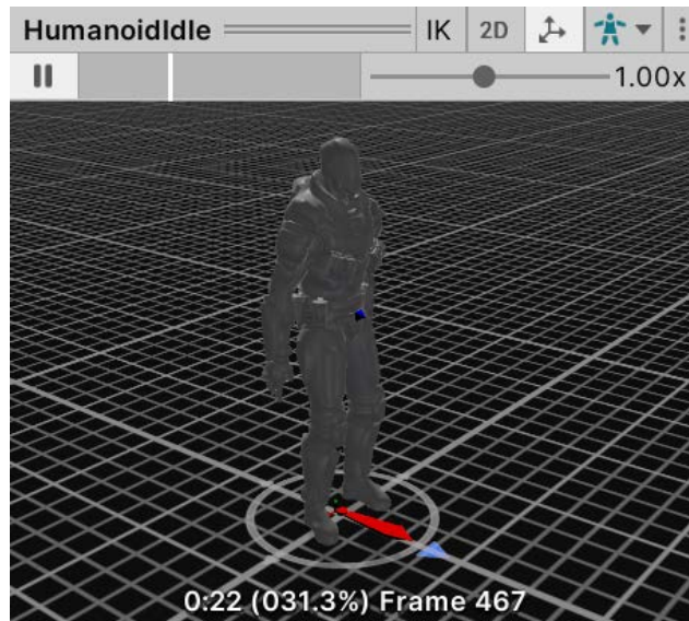
Figure 12.8 – Animation preview
