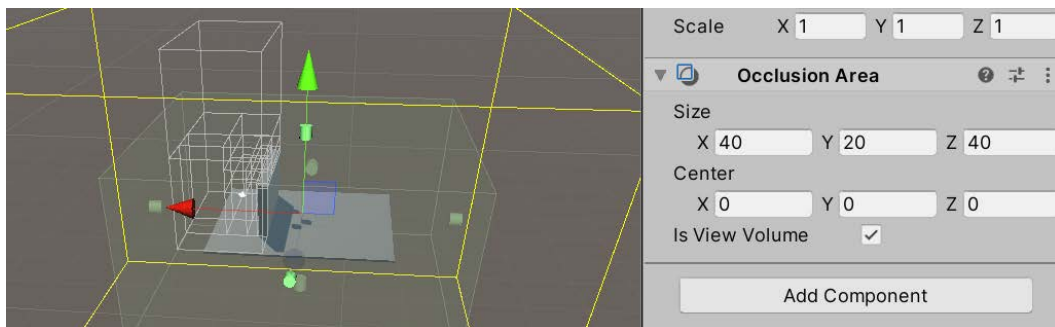
Figure 19.15 – Occlusion Area
