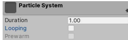
Figure 7.7 – Looping checkbox
