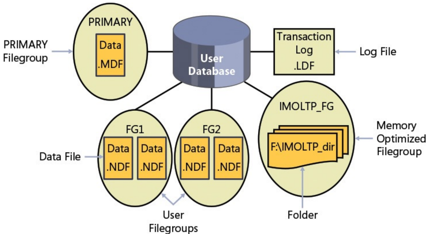
FIGURE 1-7 Database layout.
