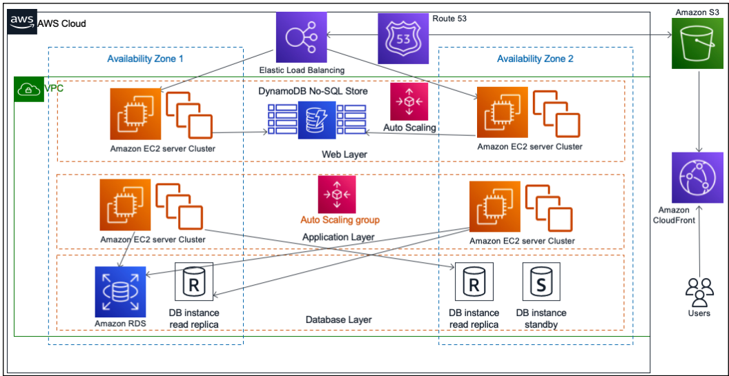
Figure 6.3: A stateless application architecture
