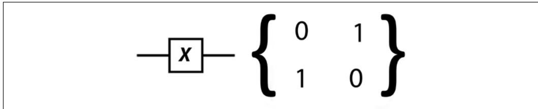
Figure 16.3: Pauli-X gate
