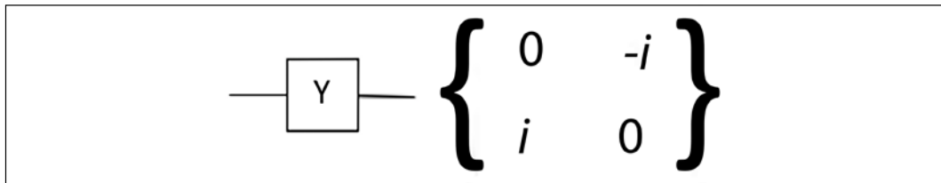
Figure 16.4: Pauli-Y gate
