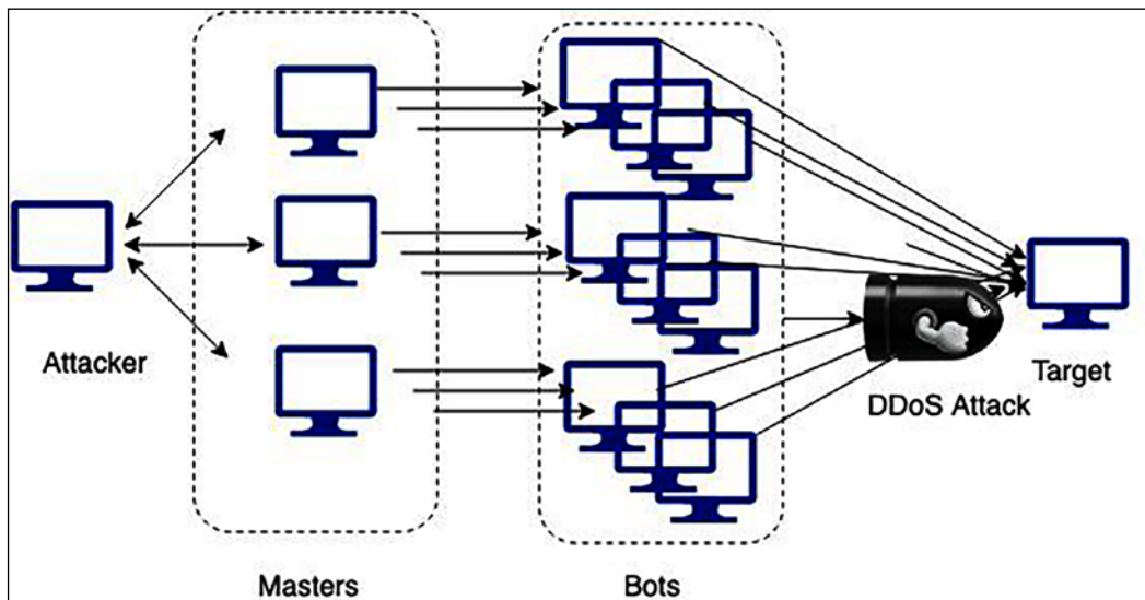
Figure 8.8: DDoS attack
