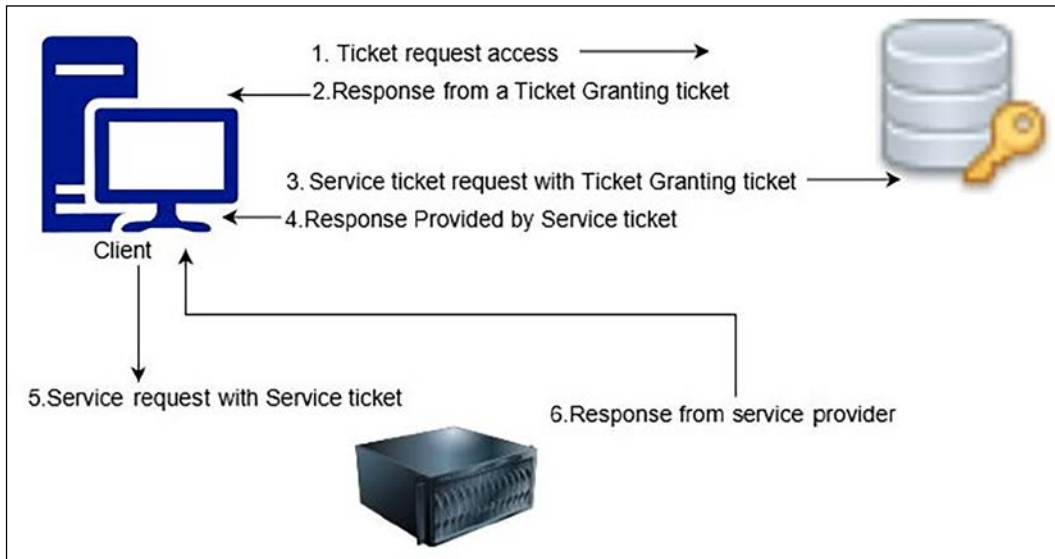
Figure 8.3: Kerberos authentication
