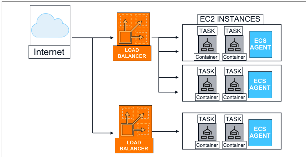
Figure 6.23: Container deployment architecture
