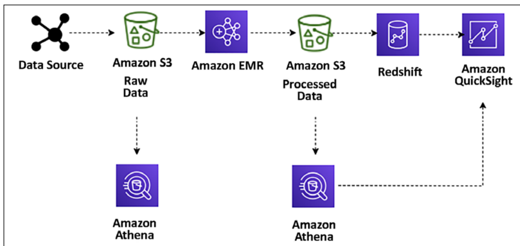
Figure 13.5: Data lake ETL pipeline for big data processing
