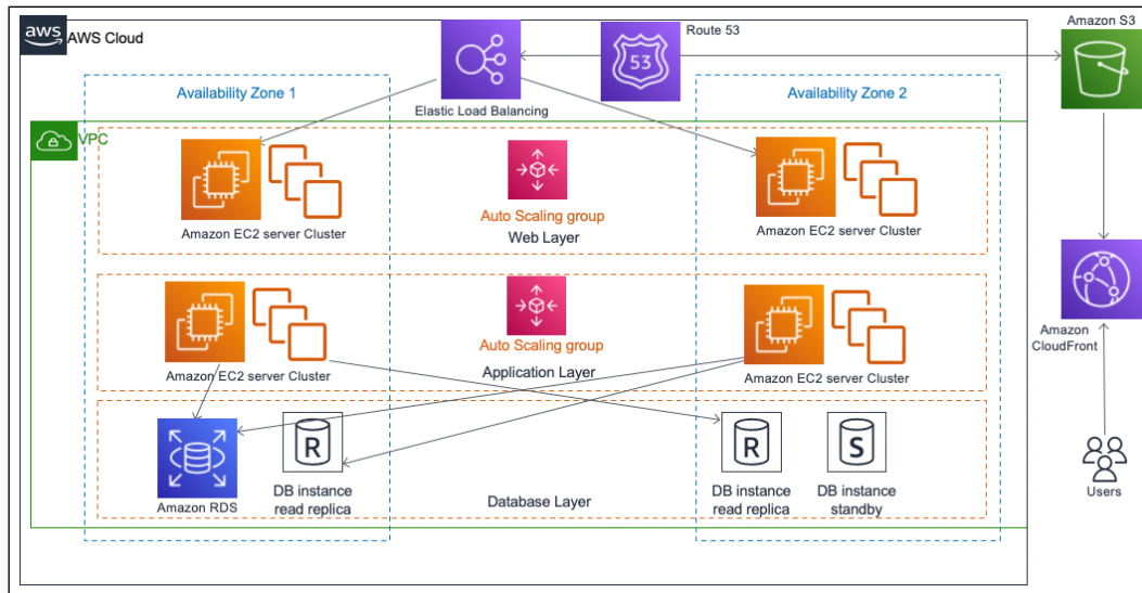
Figure 5.4: On-premise to AWS cloud architecture mapping
