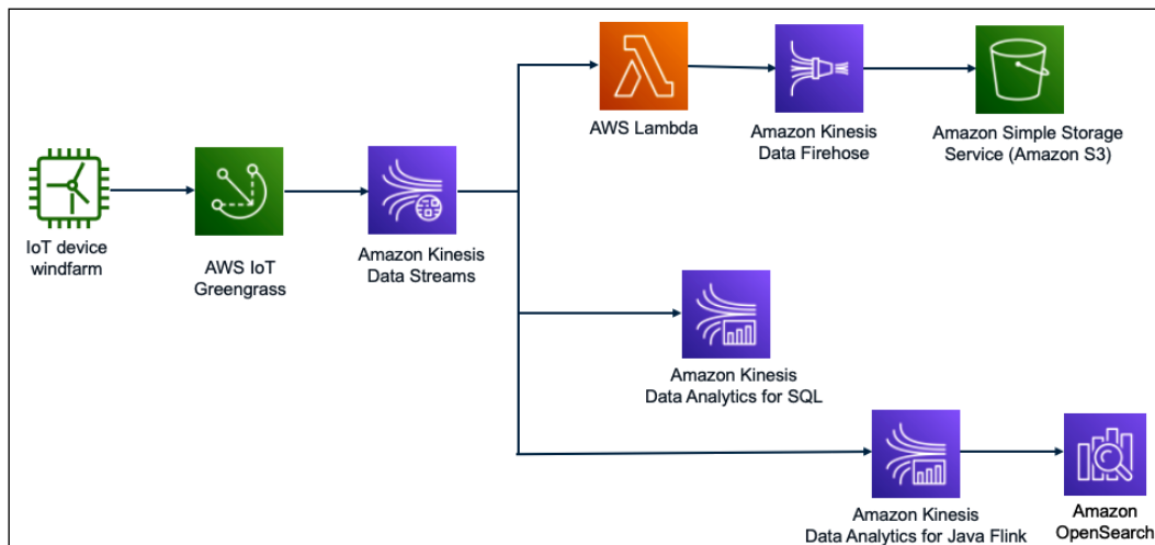
Figure 13.11: Streaming data analytics for IoT data
