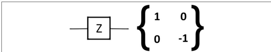
Figure 16.5: Pauli-Z gate
