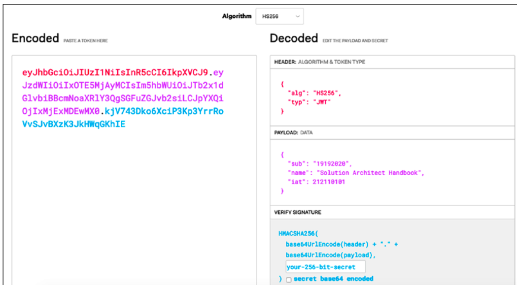
Figure 8.7: Sample JWT
