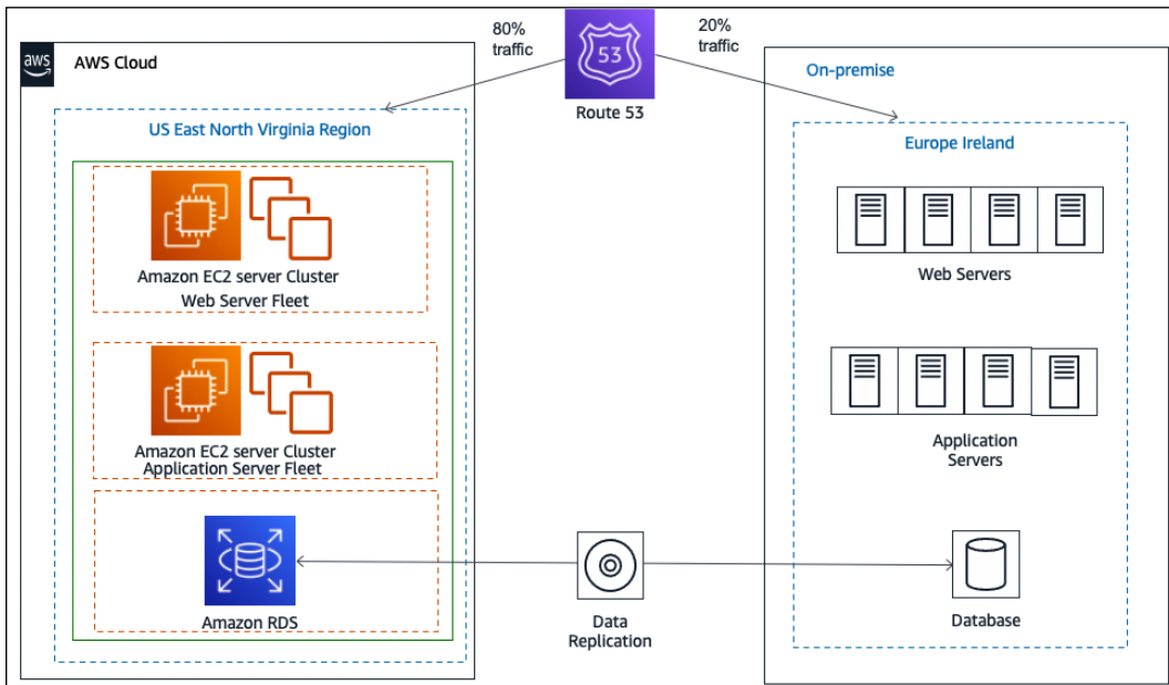
Figure 5.5: Live migration cutover using blue-green deployment
