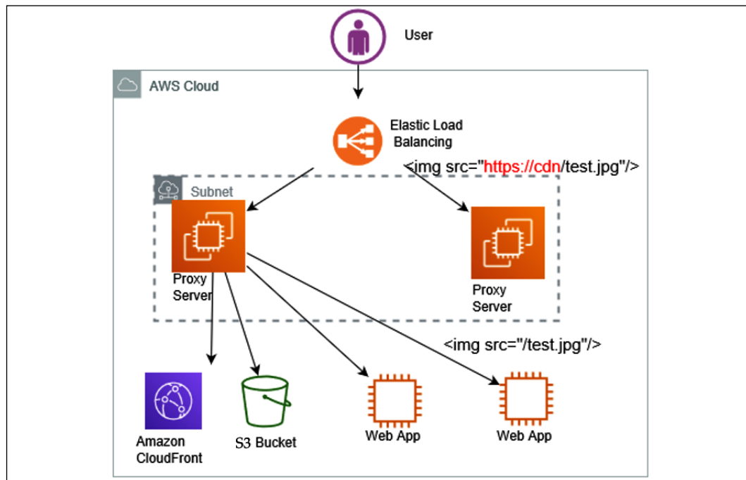
Figure 6.17: Rewrite proxy pattern architecture
