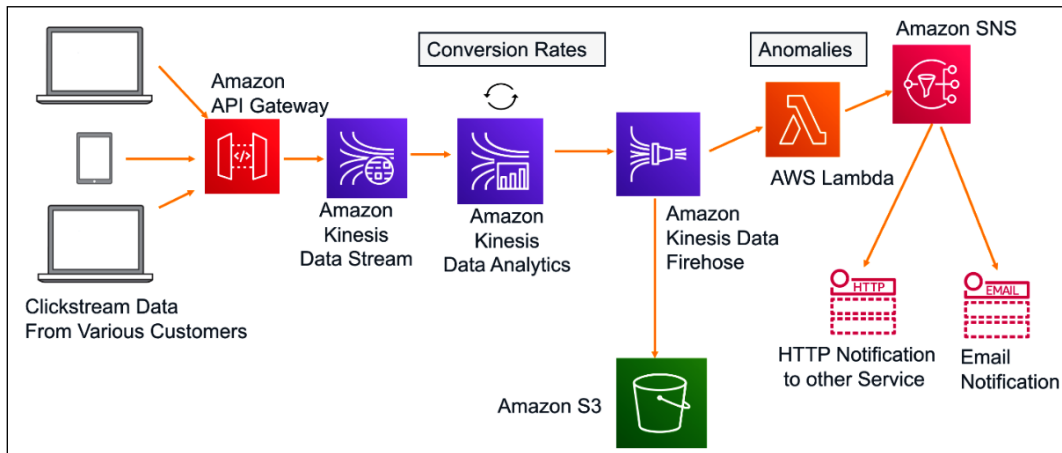
Figure 6.12: Clickstream analysis event stream architecture
