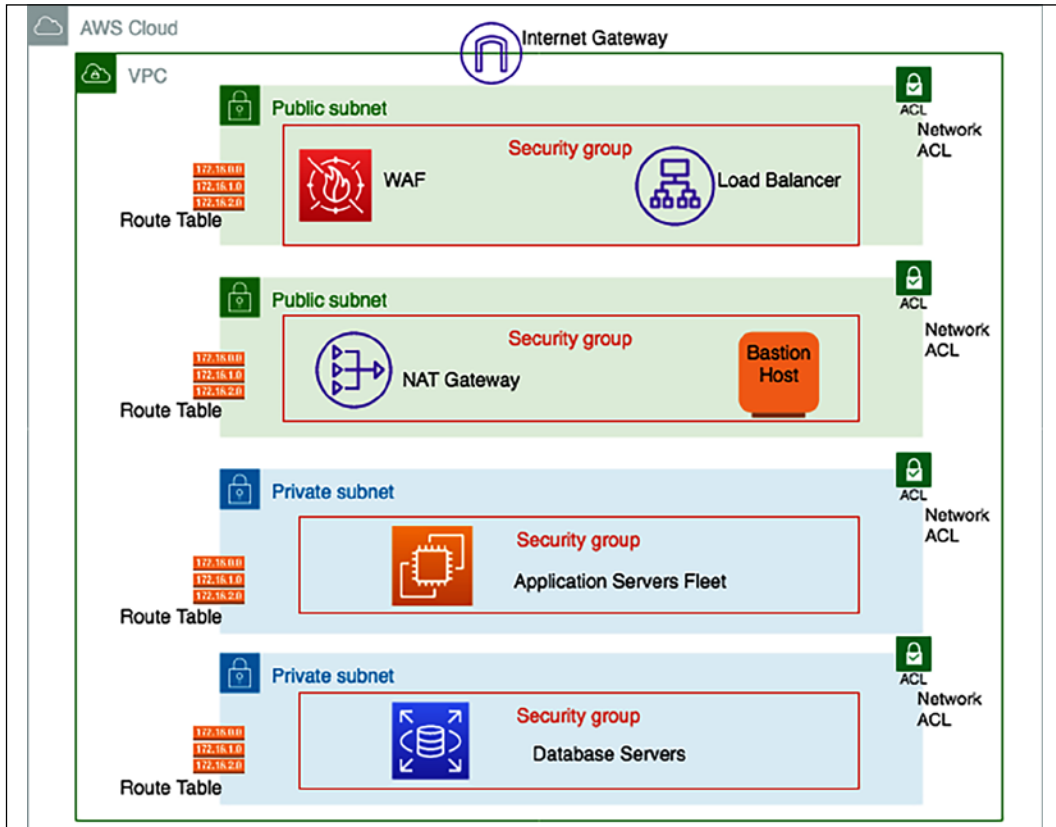
Figure 8.10: Network configuration for infrastructure security
