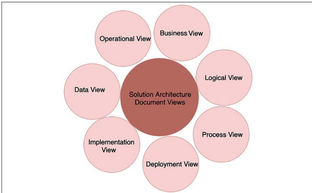
Figure 18.1: SAD views
