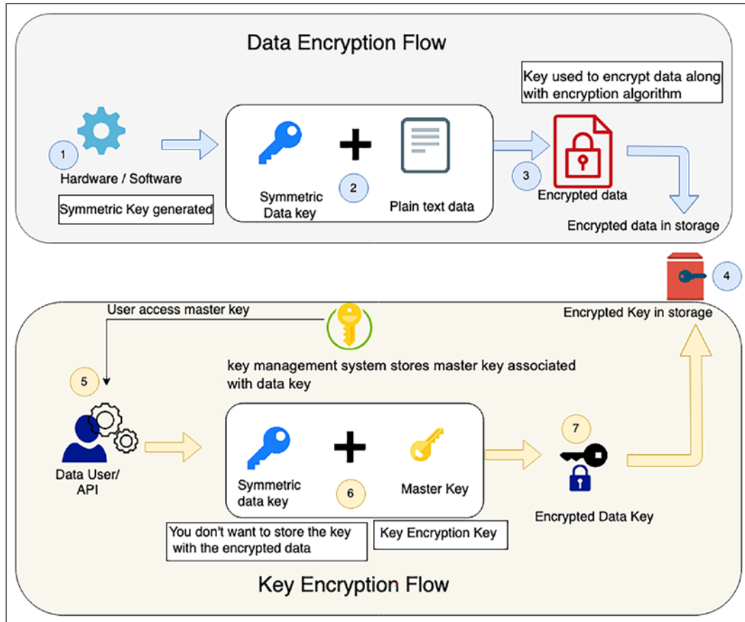
Figure 8.11: Envelope encryption
