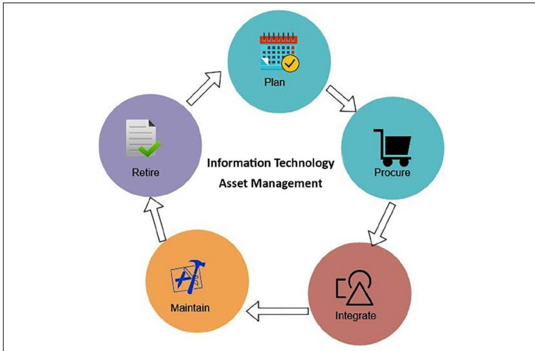
Figure 10.1: ITAM process
