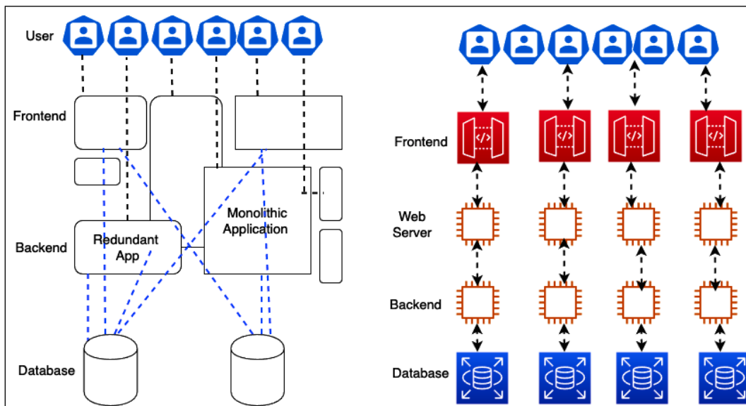
Figure 11.3: Architectural standardization
