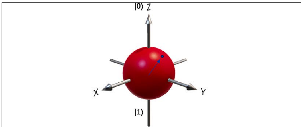
Figure 16.2: 3D representation of an electron's spin along with its axes
