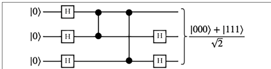
Diagram 16.8: Operation in a quantum circuit
