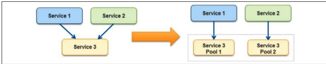
Figure 6.19: Bulkhead pattern
