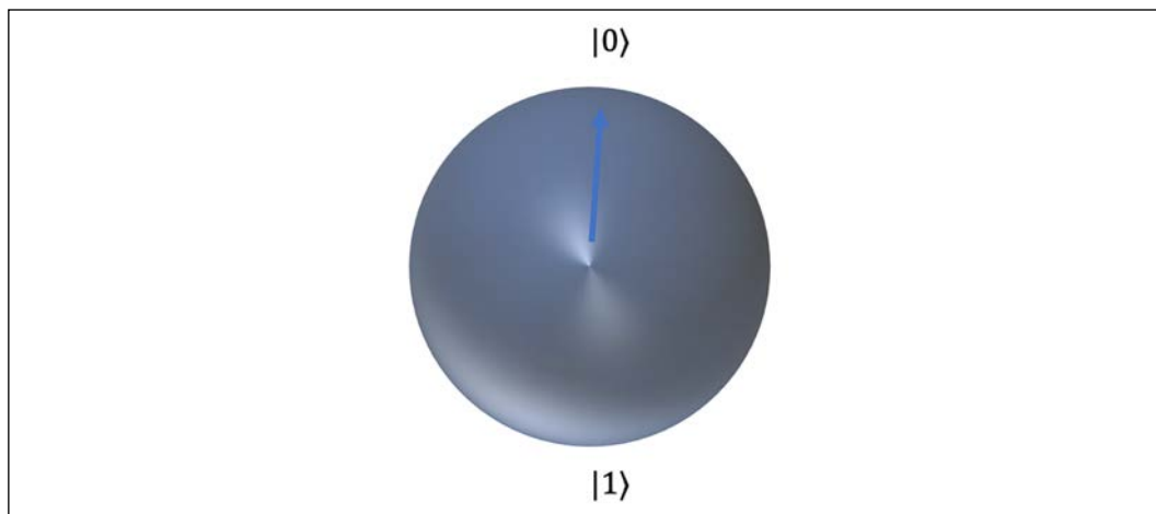
Figure 16.1: Bloch sphere – abstract representation of a qubit
