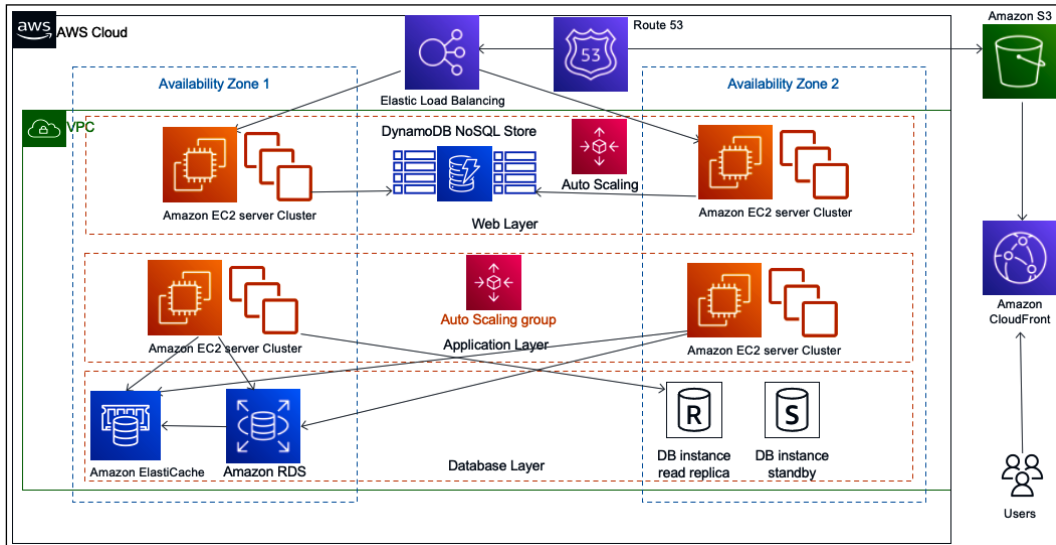
Figure 6.14: Cache distribution pattern architecture
