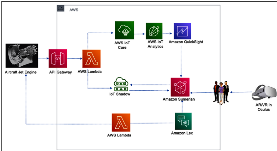
Figure 15.6: Digital twin architecture for an aircraft jet engine
