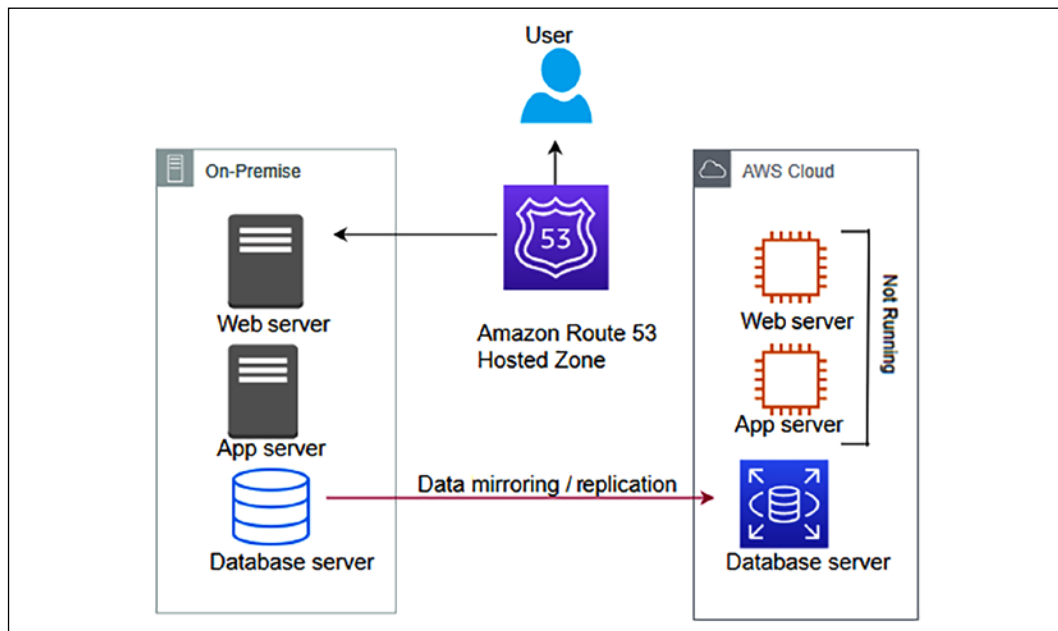
Figure 9.6: The pilot light data replication to DR site scenario
