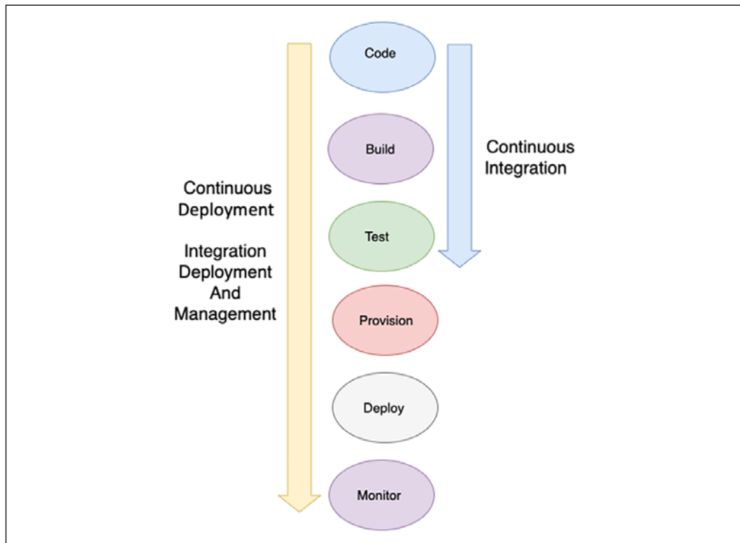
Figure 12.2: CI/CD
