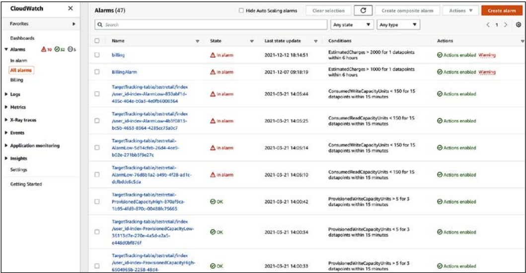
Figure 10.10: Alarm dashboard
