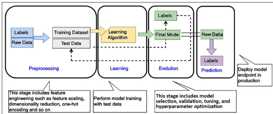
Figure 14.1: ML workflow
