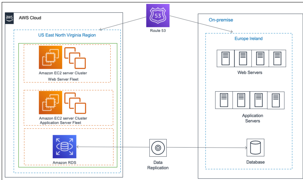
Figure 3.6: Hybrid multi-site disaster recovery architecture
