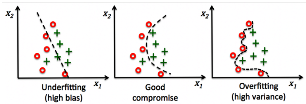
Figure 14.2: ML model overfitting versus underfitting
