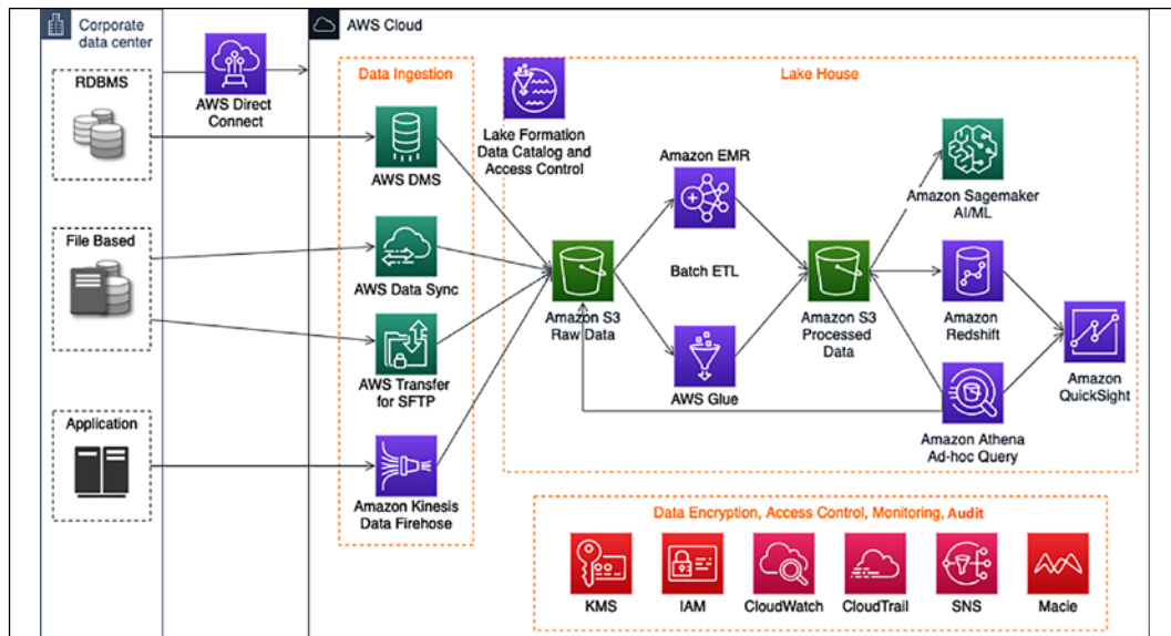
Figure 13.12: Data lake reference architecture
