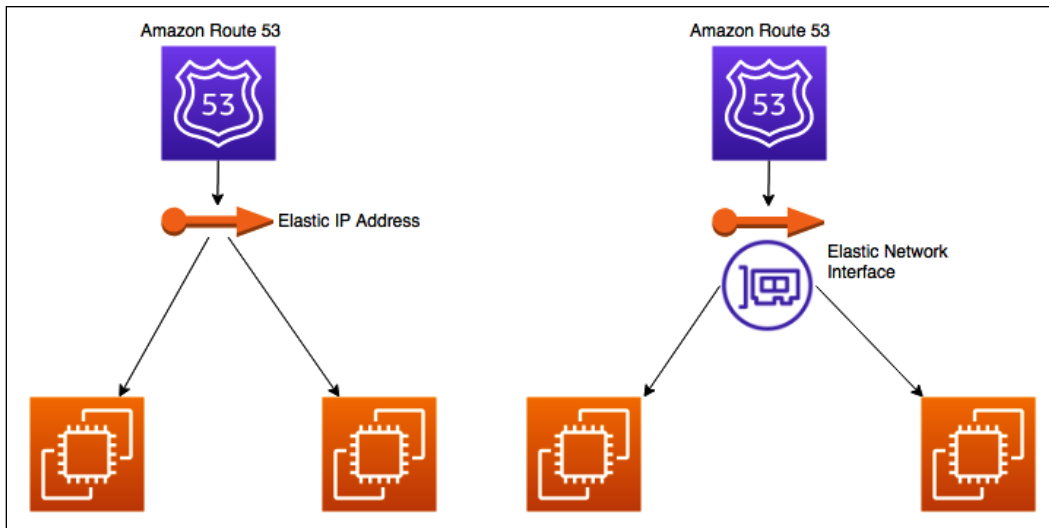
Figure 6.20: Floating IP and interface pattern
