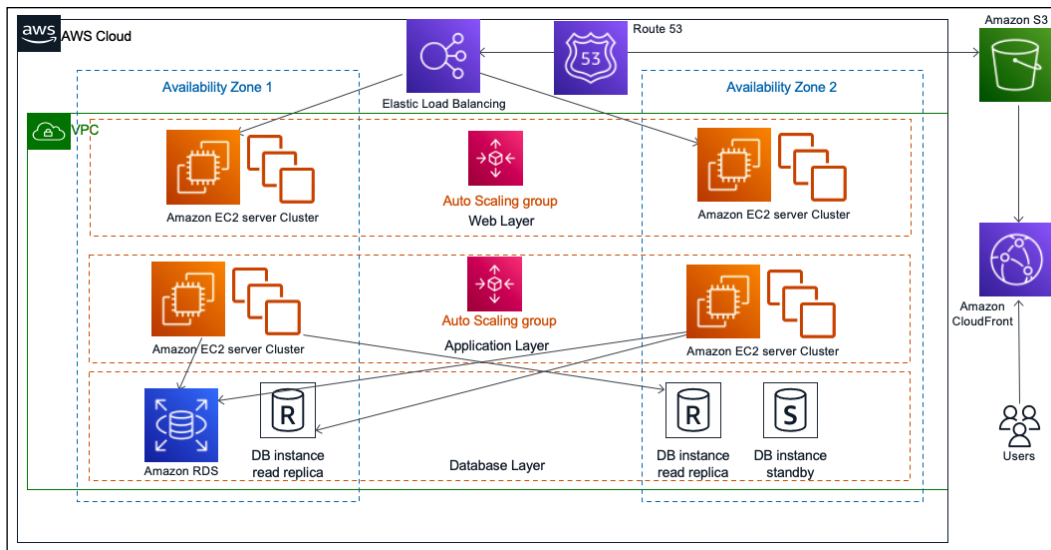
Figure 6.1: Three-tier website architecture
