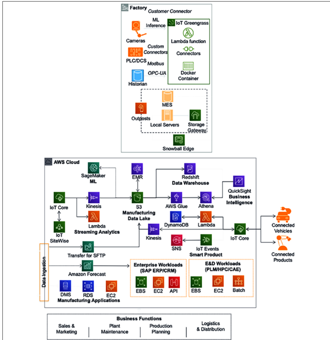
Figure 15.4: Connected Factory architecture in the AWS cloud
