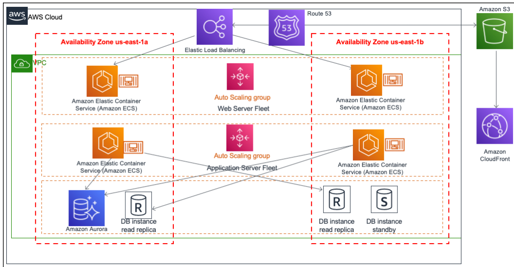
Figure 3.4: High availability and resilience architecture
