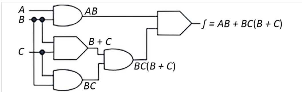
Figure 16.7: Operation in a Boolean circuit
