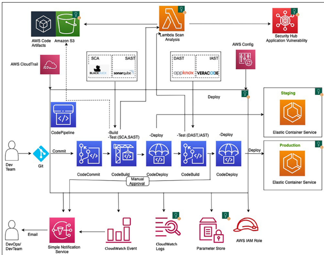
Figure 12.15: DevSecOps CI/CD pipeline architecture in the AWS cloud
