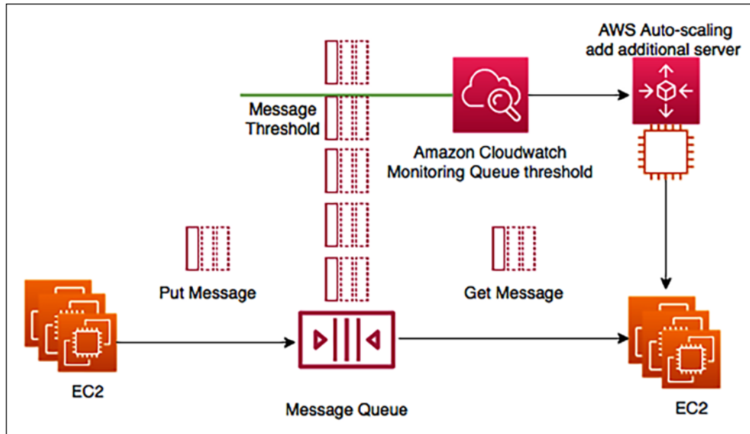
Figure 6.10: Job observer pattern architecture
