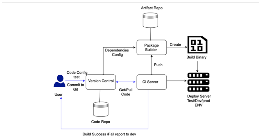
Figure 12.3: CI/CD for DevOps
