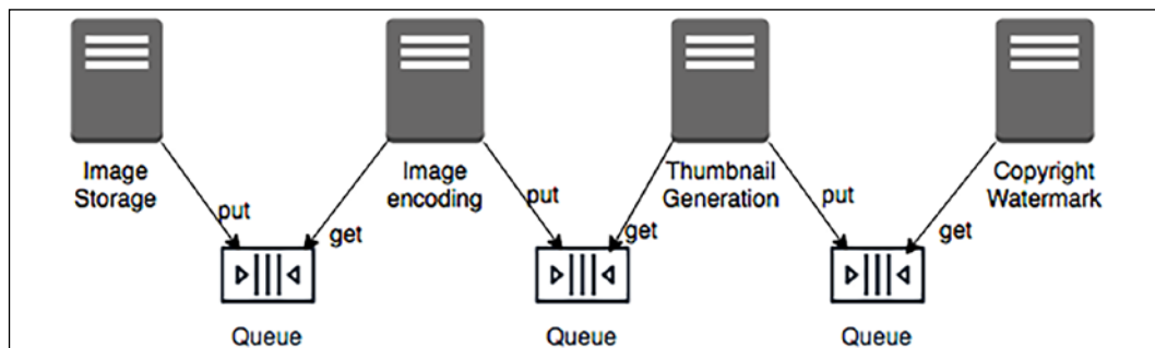
Figure 4.7: Queue-based, loosely coupled architecture
