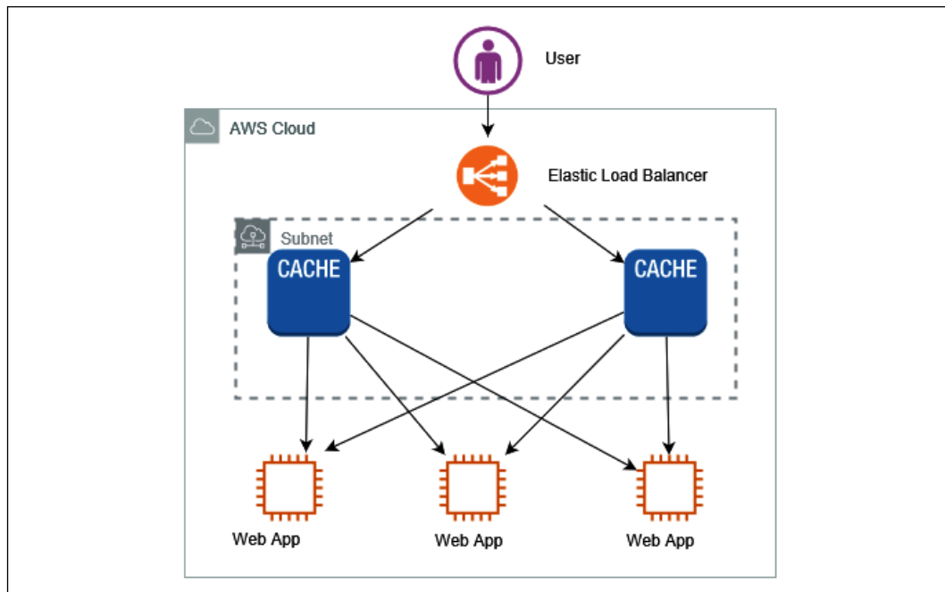
Figure 6.16: Cache proxy pattern architecture
