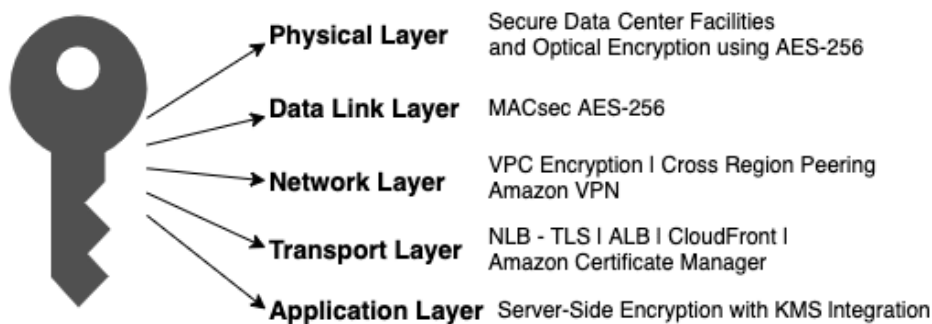
Figure 19.1 – The AWS cryptography stack
