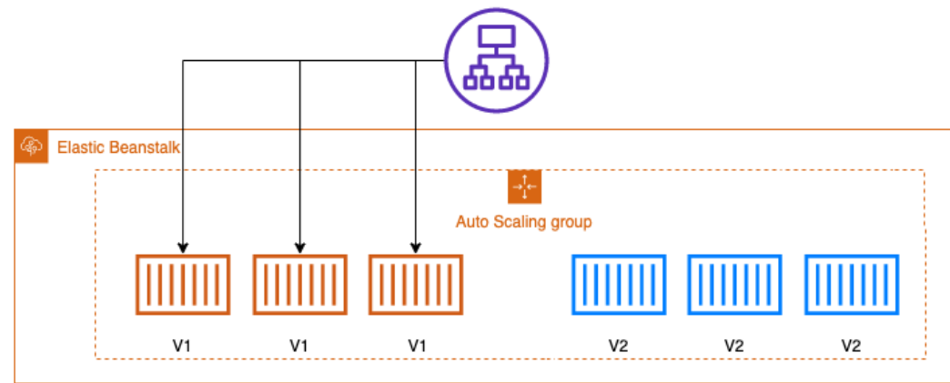
Figure 11.6 – Immutable deployment during deployment
