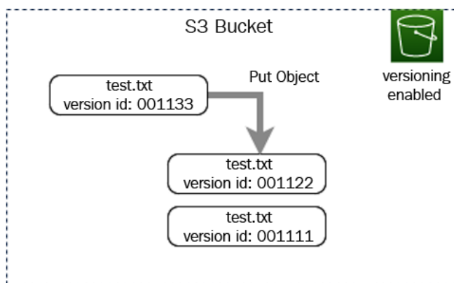
Figure 4.19 – An S3 bucket with versioning enabled showing version ids
