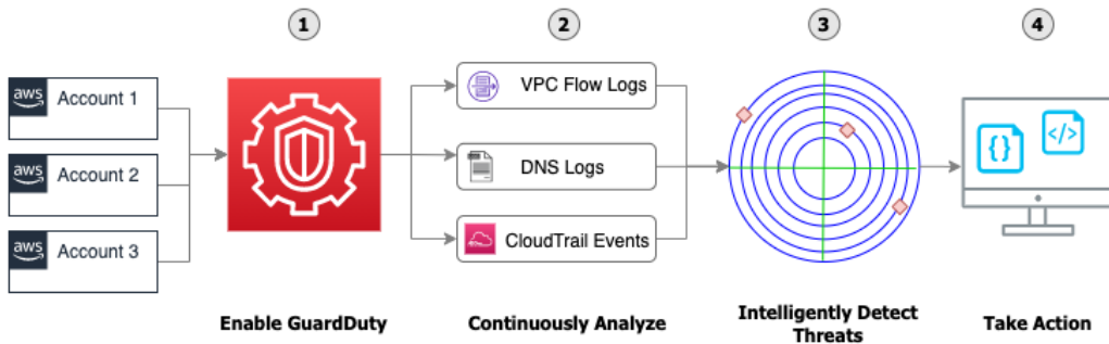
Figure 22.1 – The GuardDuty flow from enablement to taking action
