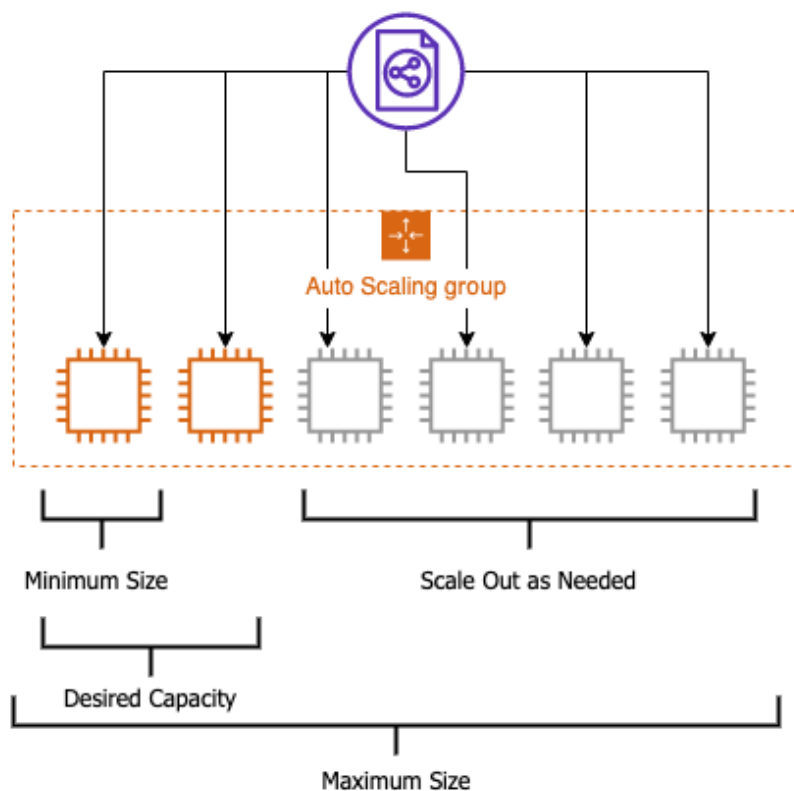
Figure 18.2 – ASG visualization
