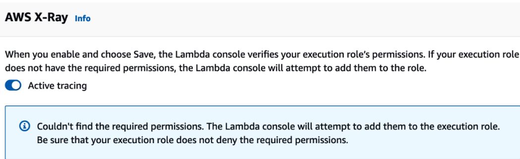
Figure 14.9 – Adding AWS X-Ray to our Lambda function
