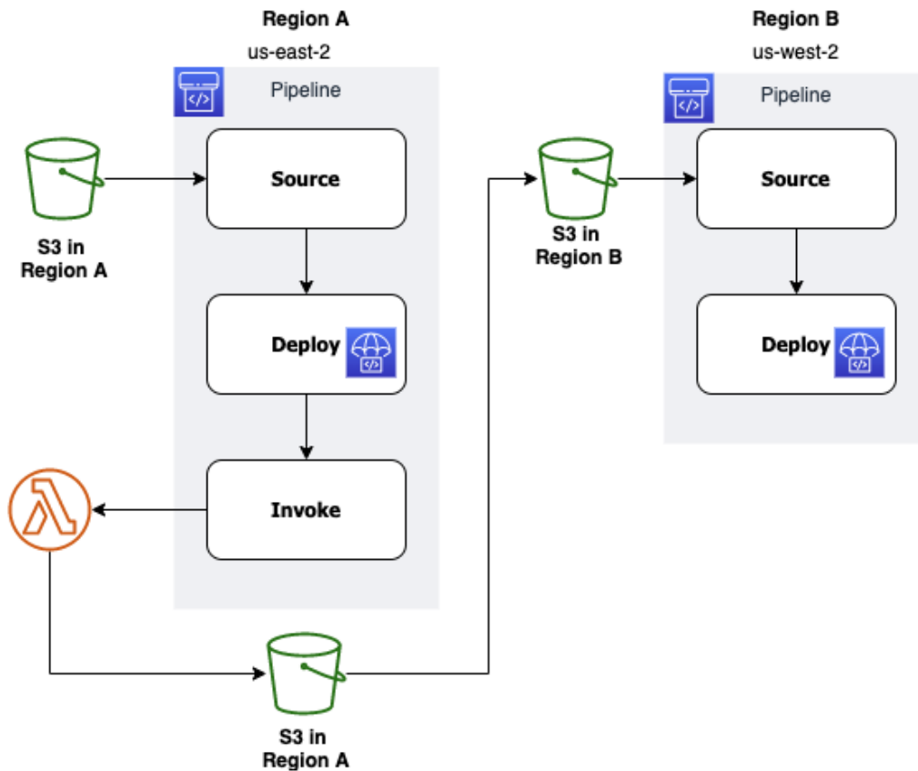
Figure 9.13 – Using CodePipeline and CodeDeploy to deploy to multiple regions
