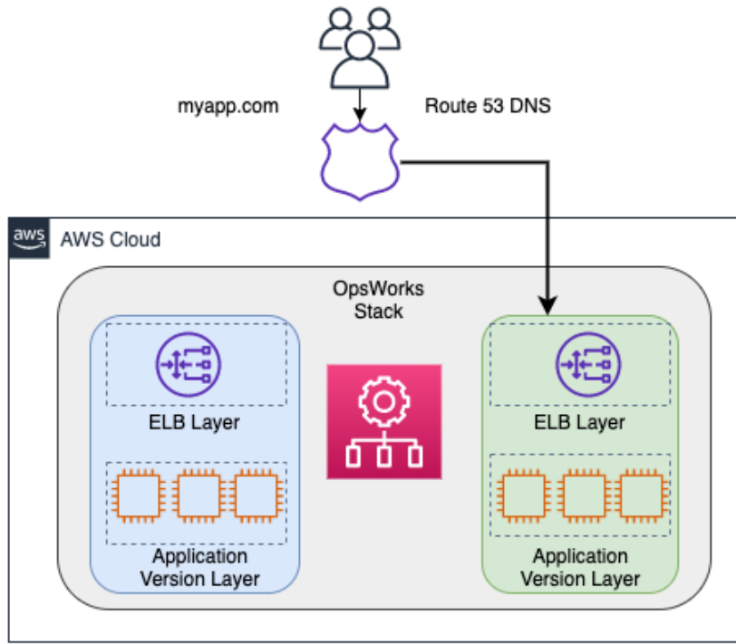
Figure 13.8 – Cloning an OpsWorks stack
