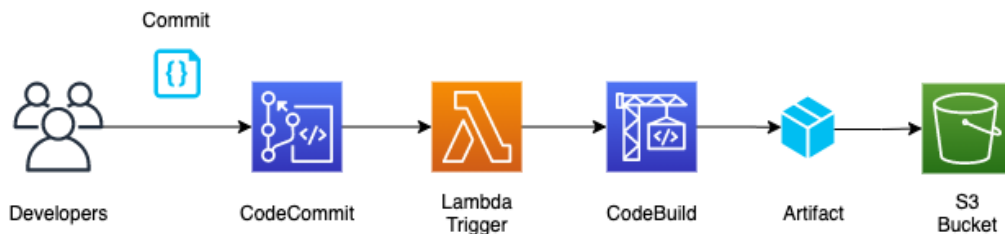
Figure 8.23 – Triggering a CodeBuild job from CodeCommit
