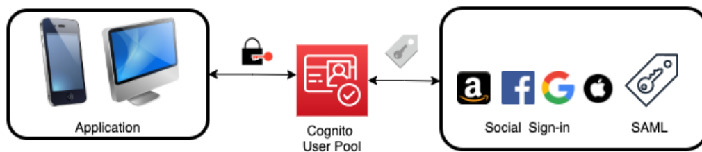
Figure 3.18 – Cognito user pool authentication
