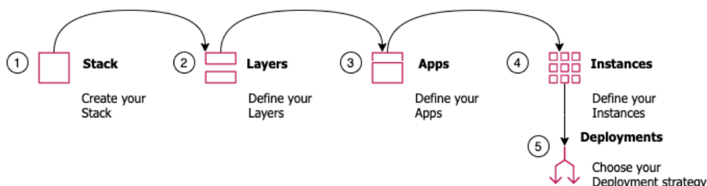
Figure 10.2 – Overview of how OpsWorks operates
