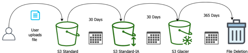
Figure 4.3 – An example S3 lifecycle policy
