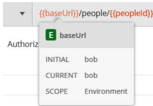
Figure 4.8 – Variable values coming from the narrowest scope
