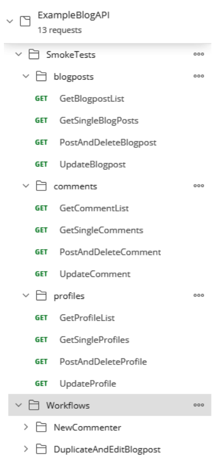
Figure 10.6 – Test folder structure
